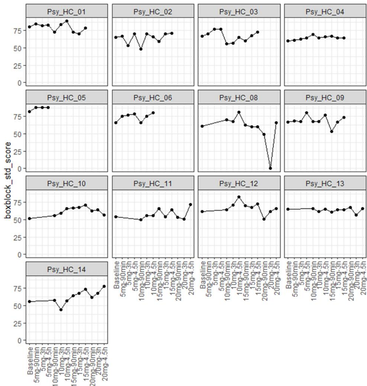
FigureS3.3: Individual profiles for boxblock_std_score .
