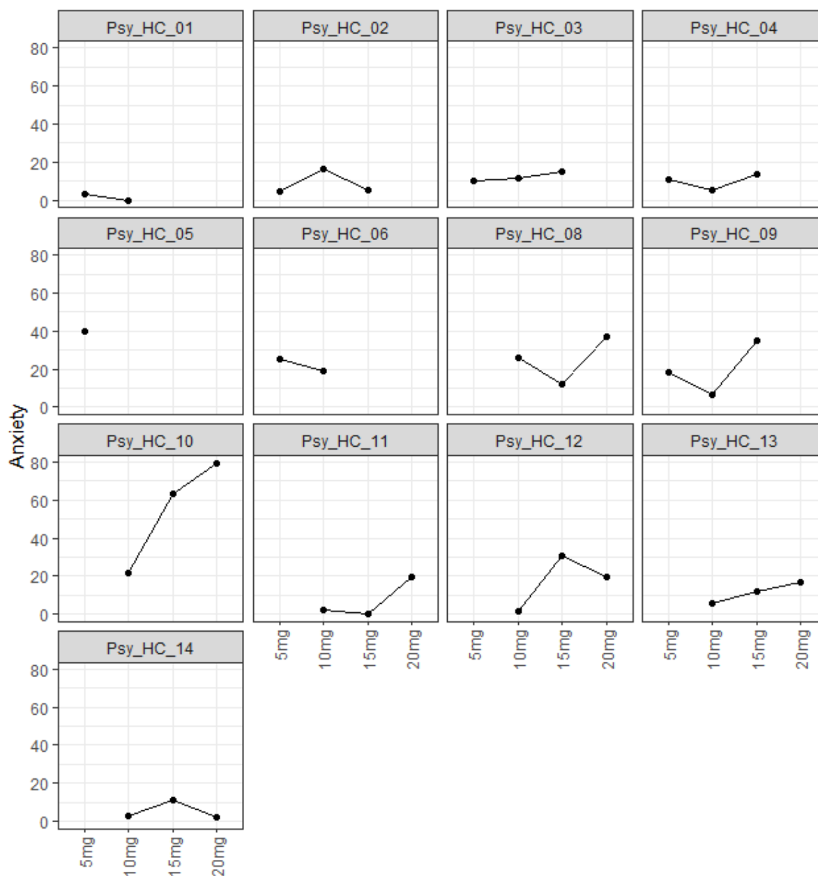
Figure S3.23: Individual profiles for Anxiety.
