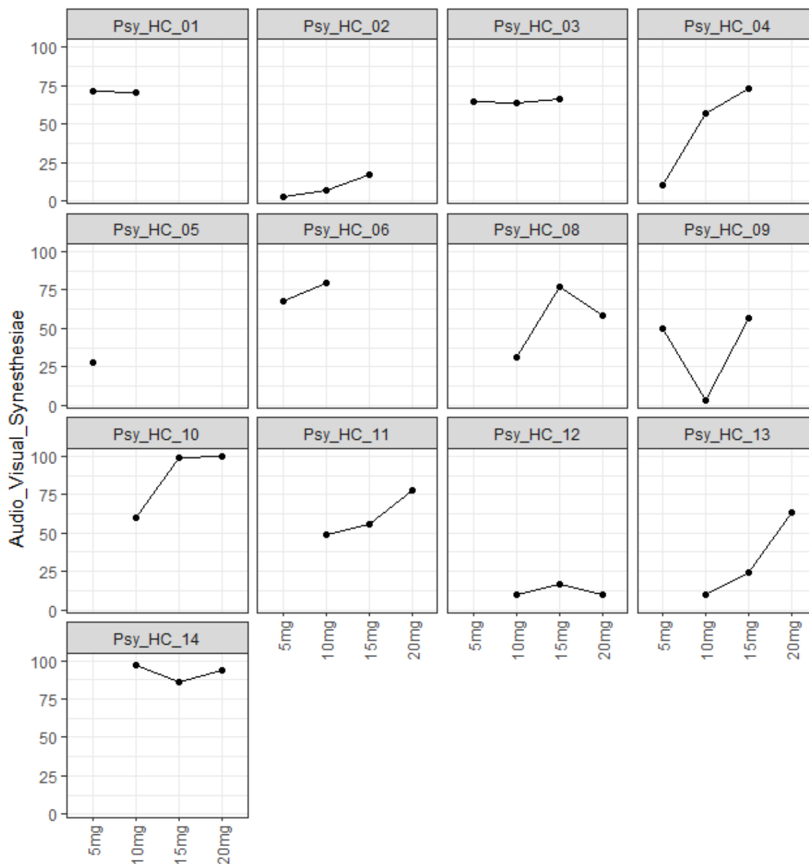
Figure S3.26: Individual profiles for Audio_Visual_Synesthesiae.
