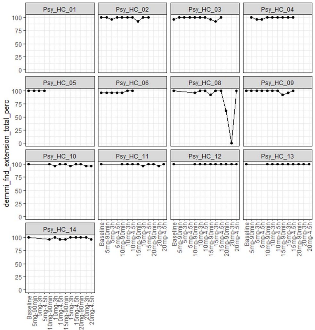
Figure S3.1: Individual profiles for demmi_fnd_extension_total_perc.
