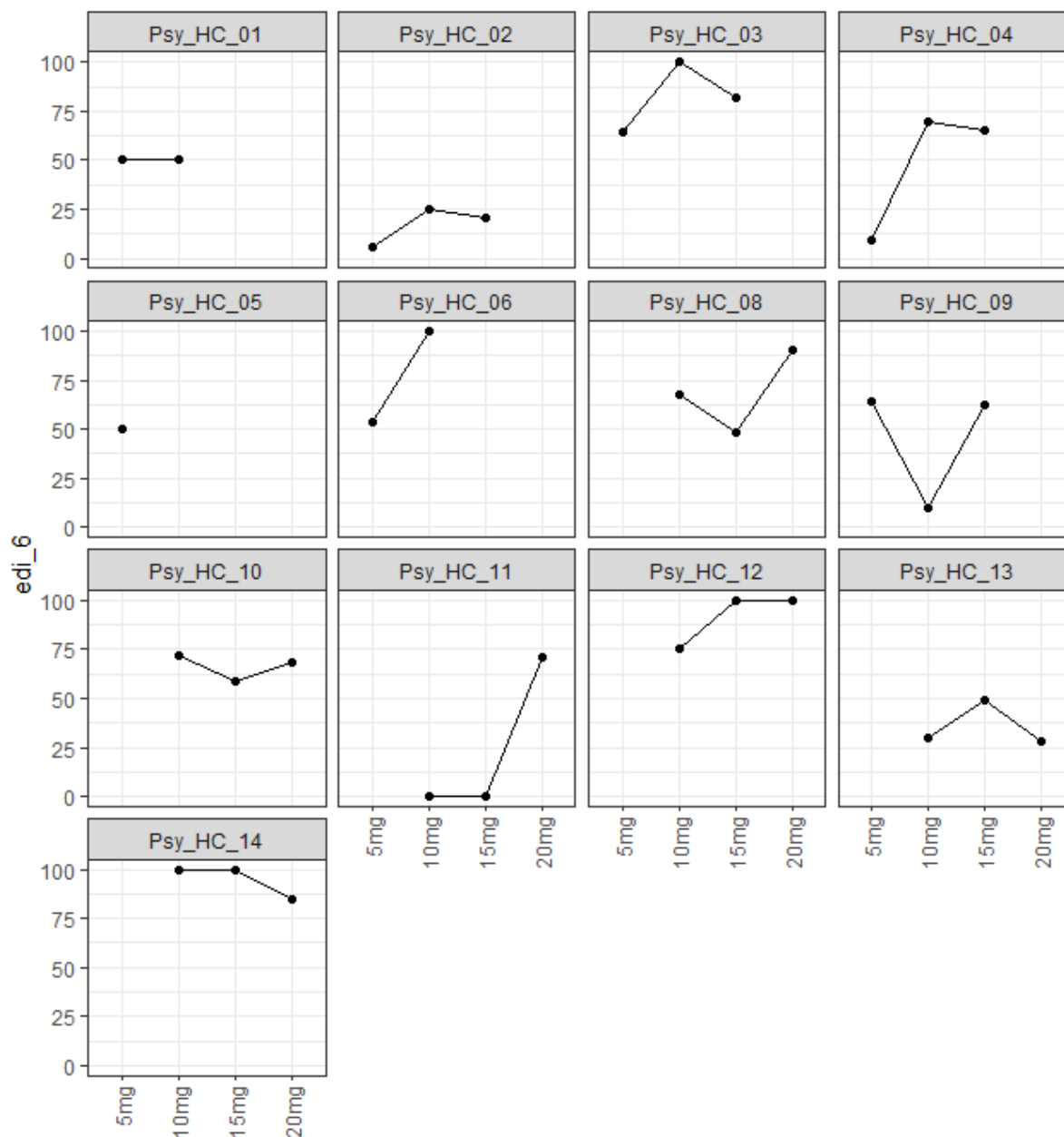
Figure S3.13: Individual profiles for edi_6 .
