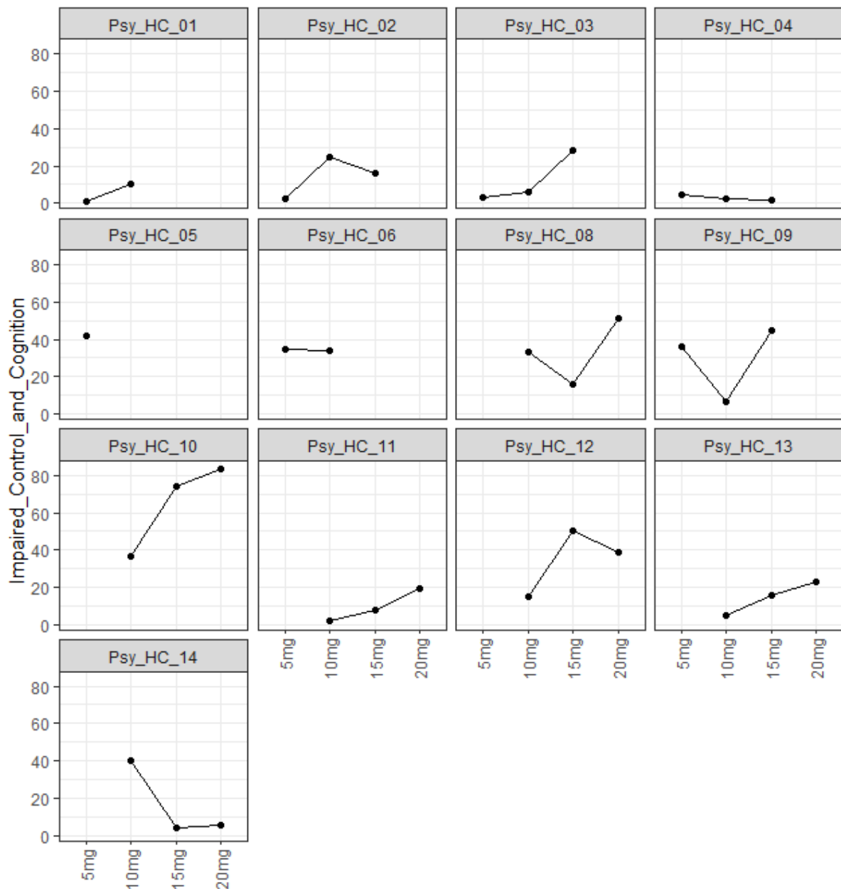
Figure S3.22: Individual profiles for Impaired_Control_and_Cognition .
