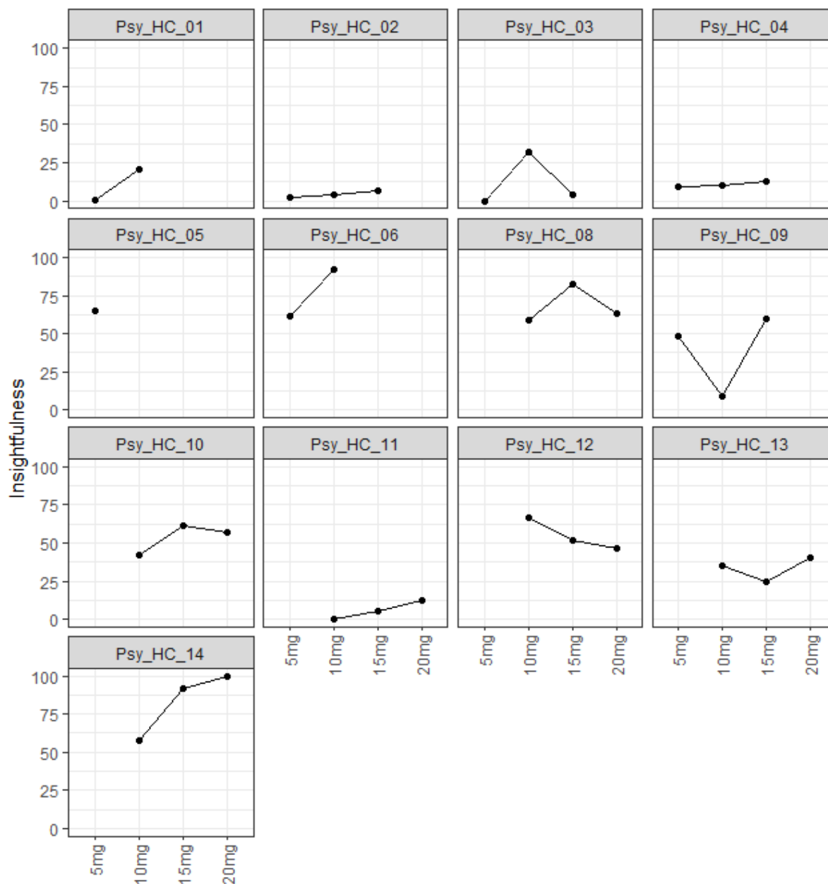
Figure S3.20: Individual profiles for Insightfulness.
