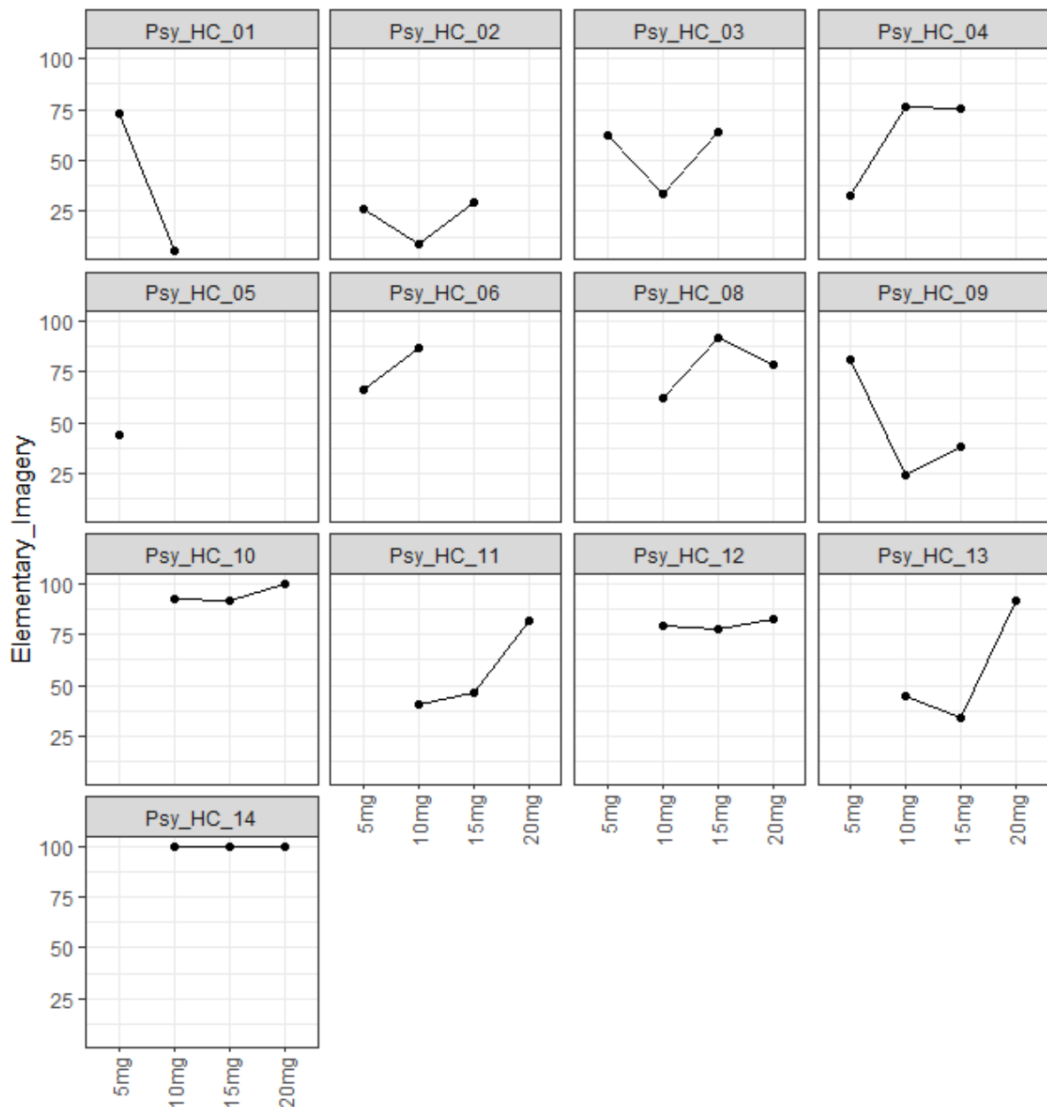
Figure S3.25: Individual profiles for Elementary_Imagery.
