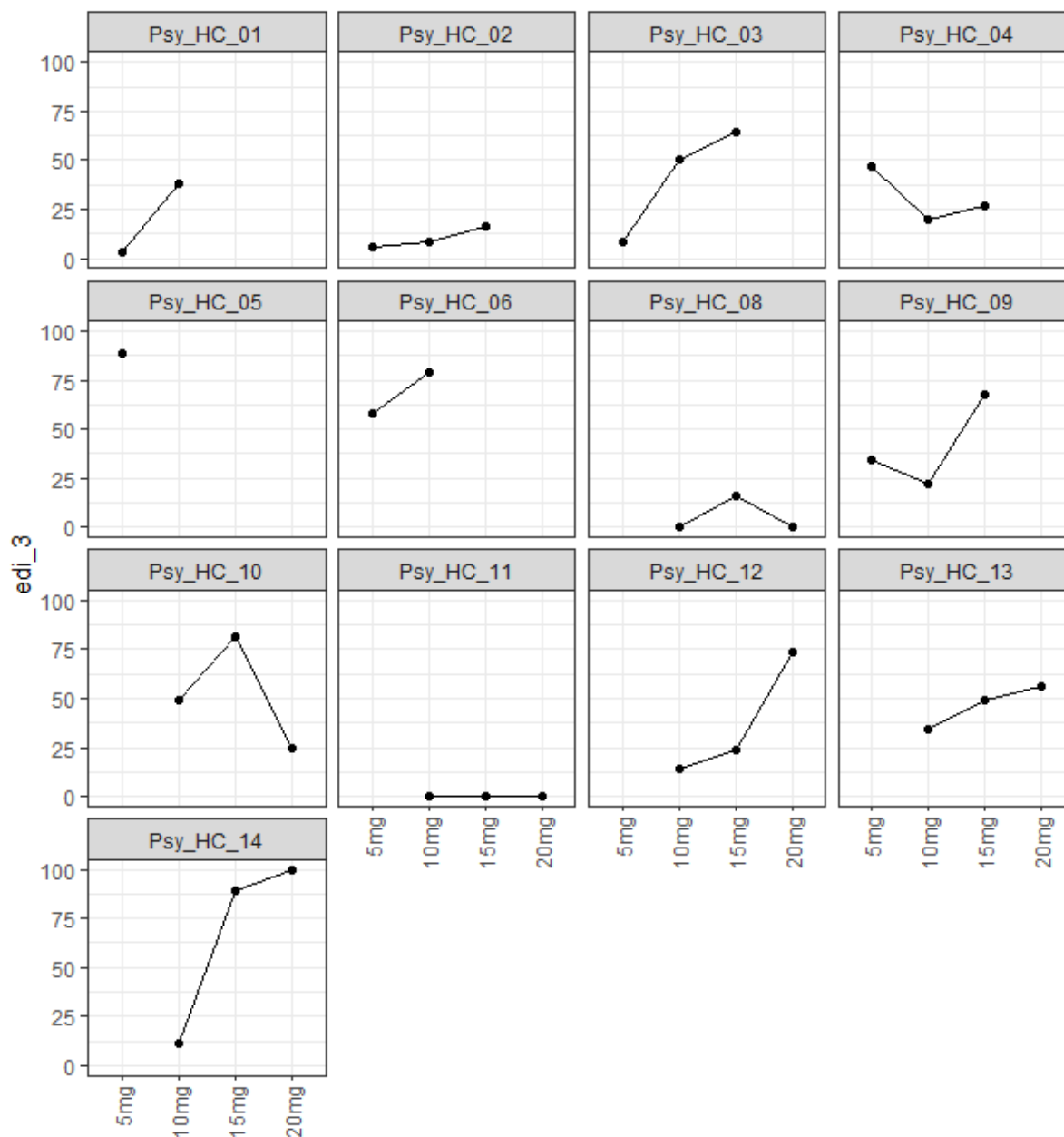
Figure S3.10: Individual profiles for edi_3.
