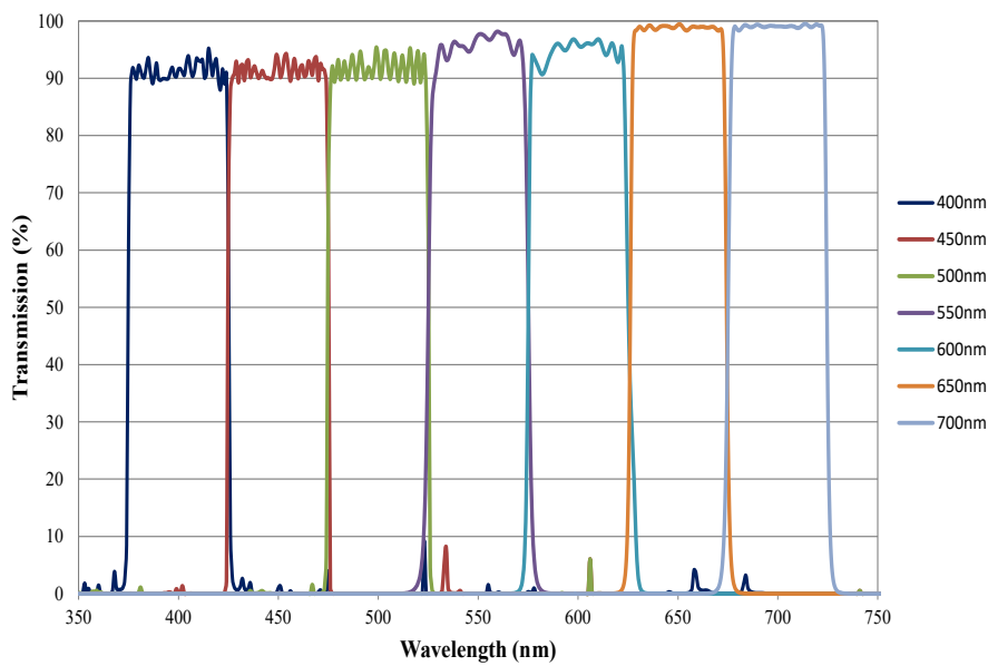
Figure S1: Transmission graphs of bandpass filters: VIS (400-700nm) 50nm Bandpass Filter Kit OD >4.0 Source: www.edmundoptics.com
