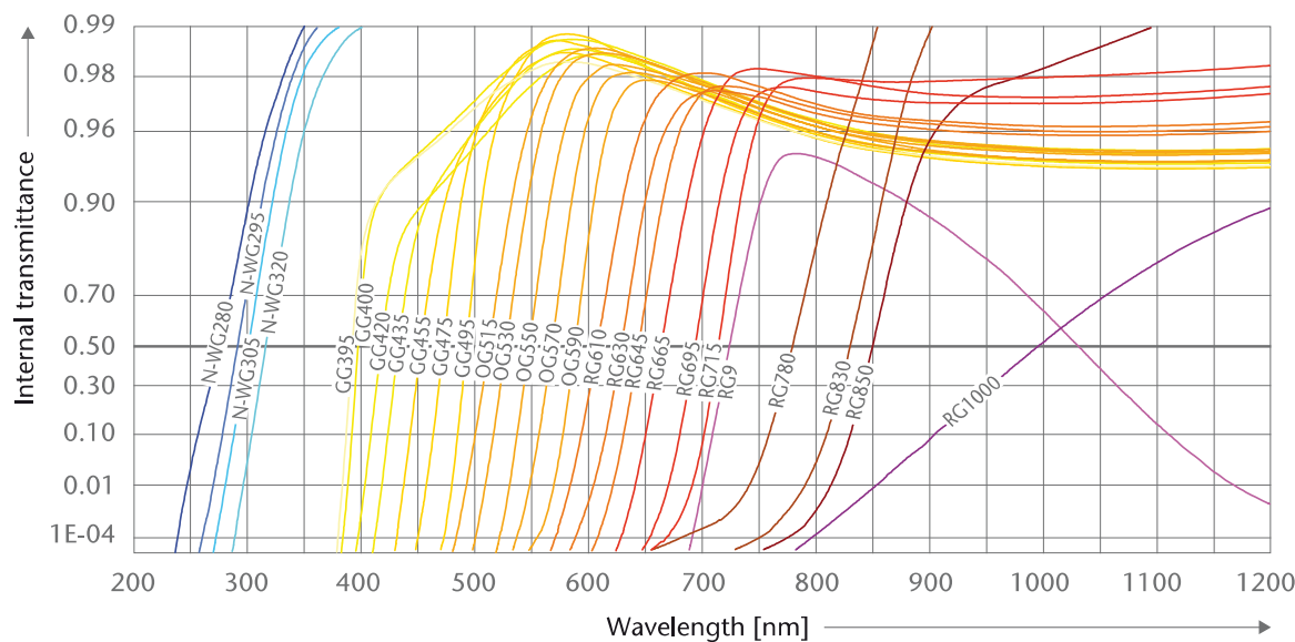
Figure S2: Internal transmittance graphs of long pass or cut-on Schott filters. Filters used: N-WG320, GG400, GG455, GG495, OG550, RG610, RG645, RG695 and RG780.
