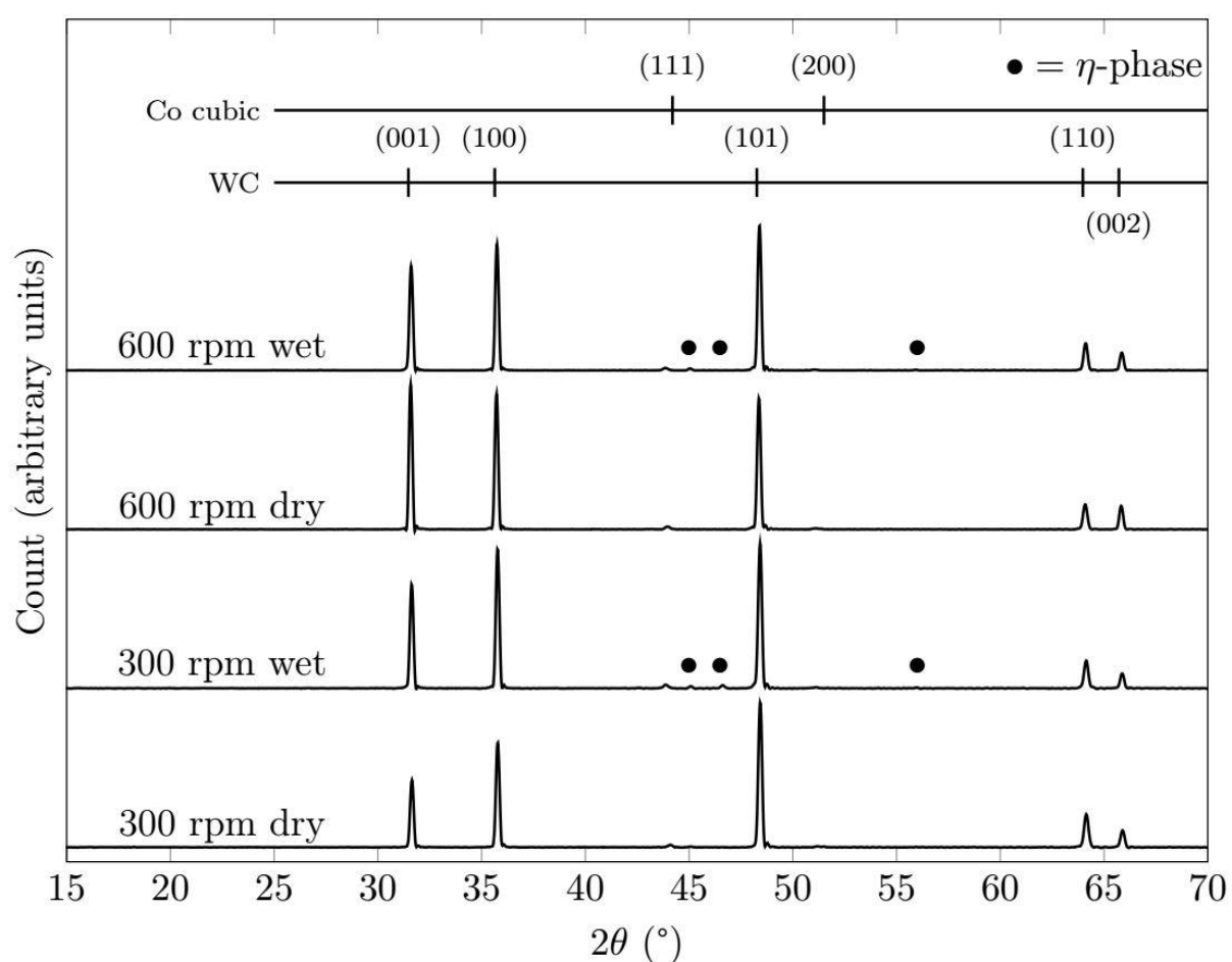
Supplementary Figure – XRD patterns of the sintered samples
