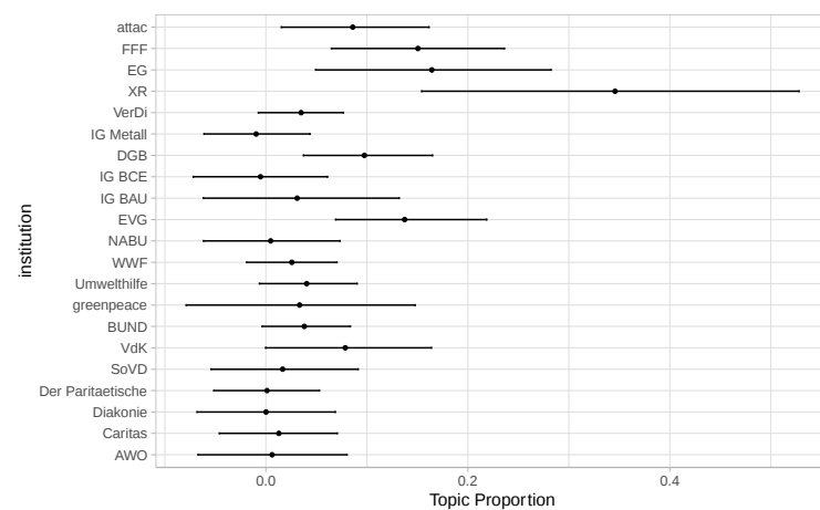
Fig. 8 STM with K=12, point estimation for topic 2, mean topic proportion by actor
