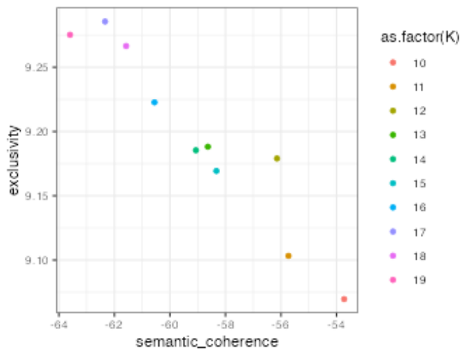
Fig. 5 STM with different K's, average values of exclusivity and semantic coherence, maximized with K = 12
