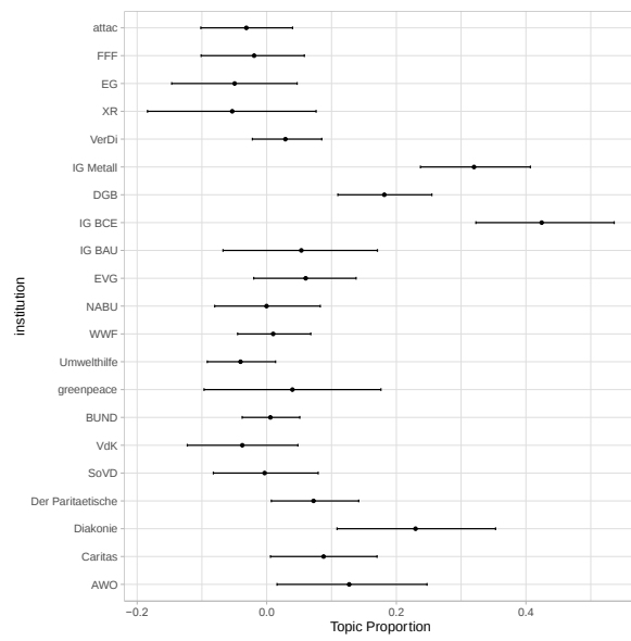
Fig. 9 STM with K=12, point estimation for topic 4, mean topic proportion by actor
