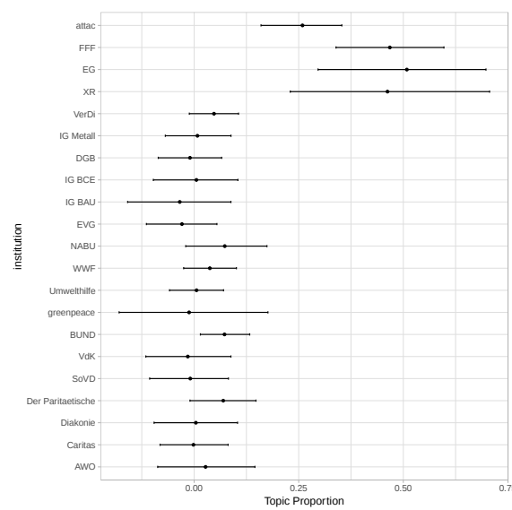
Fig. 7 STM with K=12, point estimation for topic 1, mean topic proportion by actor
