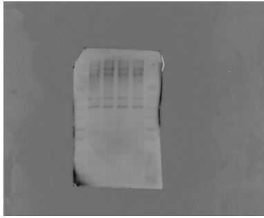
PI3K p85
