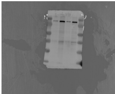
p-PI3K p85
