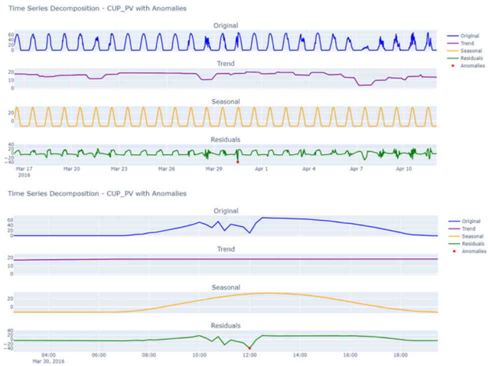
Fig. S4: A random Zoomed view of Seasonal Decomposition plots of Figure S3
