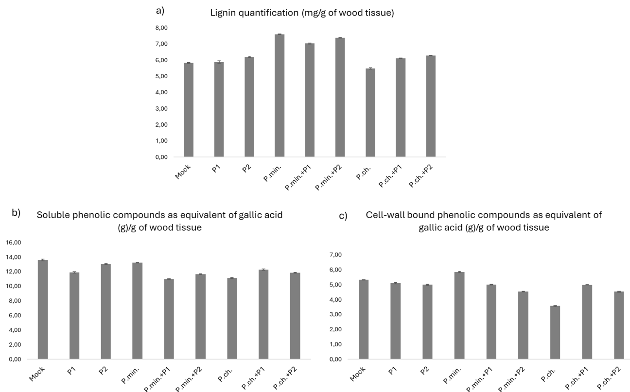
Fig. S4 Lignin (a), soluble phenolic compounds (b), and cell-wall phenolic compounds (c) quantification on 112 dpi wood tissue. All samples were tested in triplicates. Columns represent means of the three replications and the vertical bars indicate standard errors. Columns with an asterisk (*) are significantly different from the control, as determined by one-way analysis of variance (ANOVA), followed by Dunnett's test for multiple comparisons with the control ( p -value < 0.05).
