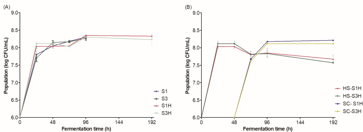
Fig. S2 Yeast growth kinetics: (A) Total viable population in pure cultures S1 ( S. cerevisiae ), S3 ( S. cerevisiae ) and in sequential inoculation schemes with Hanseniaspora sp. (S1H, S3H); (B) S. cerevisiae (SC) and Hanseniaspora sp. (HS) populations in sequential cultures (S1H and S3H). Average value of three experiments \pm standard deviation.
