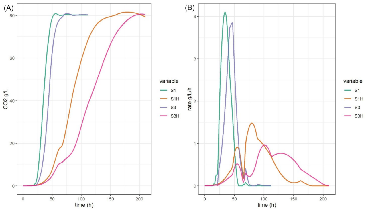
Fig. S1 (A) Fermentation kinetics expressed in released CO 2 (g/L) over time and (B) Fermentation rate expressed in released CO 2 (g/L/h) over time in pure (S1 ( S. cerevisiae ), S3 ( S. cerevisiae ) and mixed (S1H, S3H) cultures. Average values of three experiments, standard deviation <5%.
