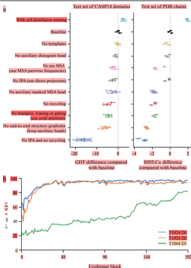
Fig. 4 | Interpreting the neural network. a , Ablation results on two target sets: the CASP14 set of domains ( n = 87 protein domains) and the PDB test set of chains with template coverage of \leq 30\% at 30% identity ( n = 2,261 protein chains). Domains are scored with GDT and chains are scored with IDDT-C \alpha . The ablations are reported as a difference compared with the average of the three baseline seeds. Means (points) and 95% bootstrap percentile intervals (error bars) are computed using bootstrap estimates of 10,000 samples. b , Domain GDT trajectory over 4 recycling iterations and 48 Evoformer blocks on CASP14 targets LmrP (T1024) and Orf8 (T1064) where D1 and D2 refer to the individual domains as defined by the CASP assessment. Both T1024 domains obtain the correct structure early in the network, whereas the structure of T1064 changes multiple times and requires nearly the full depth of the network to reach the final structure. Note, 48 Evoformer blocks comprise one recycling iteration.
