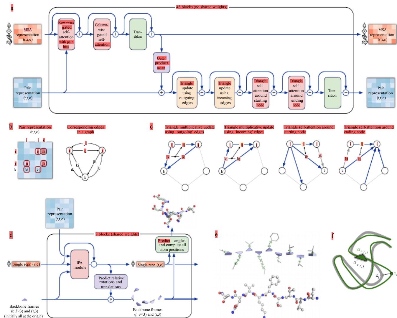
Fig. 3 | Architectural details. a , Evoformer block. Arrows show the information flow. The shape of the arrays is shown in parentheses. b , The pair representation interpreted as directed edges in a graph. c , Triangle multiplicative update and triangle self-attention. The circles represent residues. Entries in the pair representation are illustrated as directed edges and in each diagram, the edge being updated is ij . d , Structure module including Invariant point attention (IPA)
