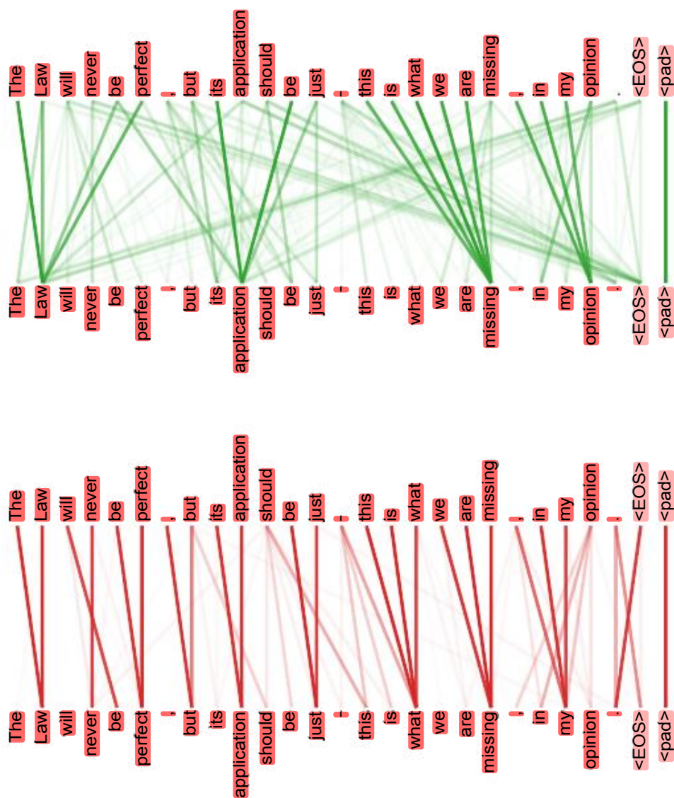
Figure 5: Many of the attention heads exhibit behaviour that seems related to the structure of the sentence. We give two such examples above, from two different heads from the encoder self-attention at layer 5 of 6. The heads clearly learned to perform different tasks.
