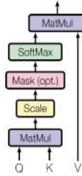
Scaled Dot-Product Attention
