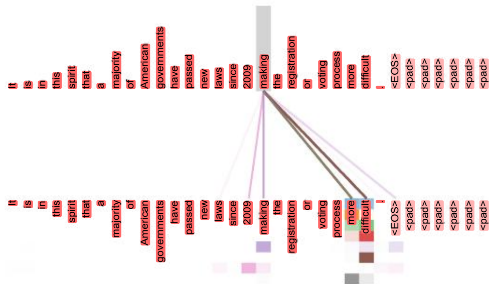
Figure 3: An example of the attention mechanism following long-distance dependencies in the encoder self-attention in layer 5 of 6. Many of the attention heads attend to a distant dependency of the verb 'making', completing the phrase 'making...more difficult'. Attentions here shown only for the word 'making'. Different colors represent different heads. Best viewed in color.
