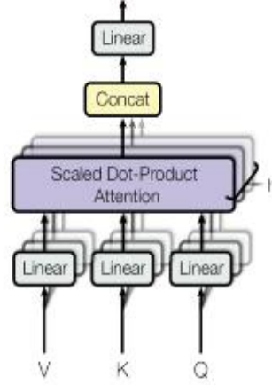
Multi-Head Attention
