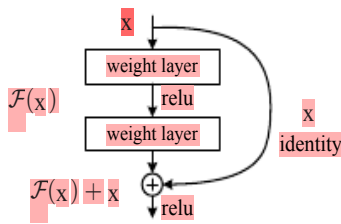
Figure 2. Residual learning: a building block.
