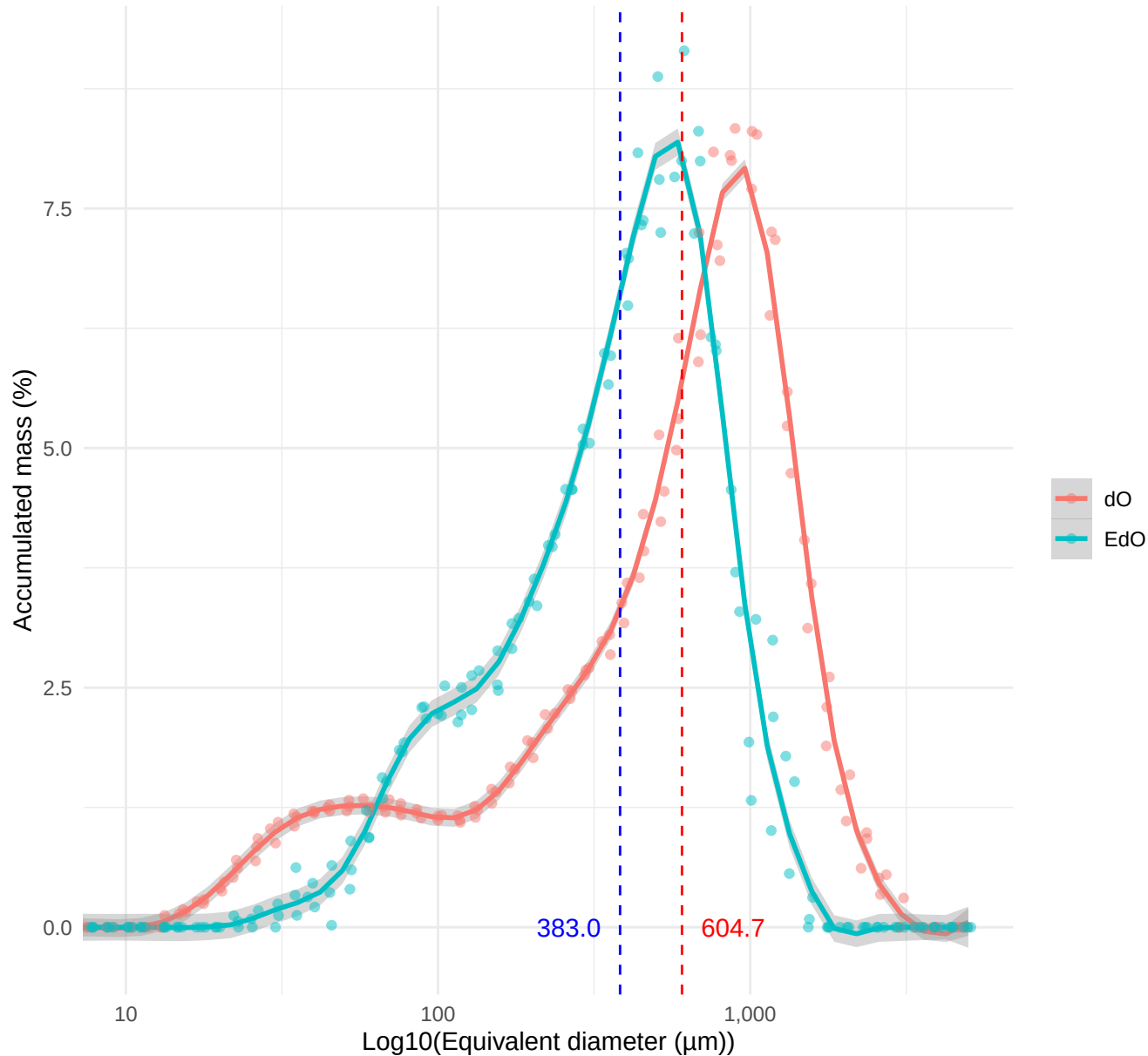
Fig. S1: Particle size distribution for samples dO (in red) and EdO (in blue). The vertical line in the respective color indicates the median position for each sample.
