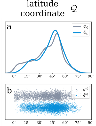
Fig. A1 True and inferred latitude distribution align closely for model (3). a. KDE of the true and inferred latitude parameter sample depicted in b . The true sample and KDE approximation are visualised in grey, while the EPI reconstruction is given in blue.
