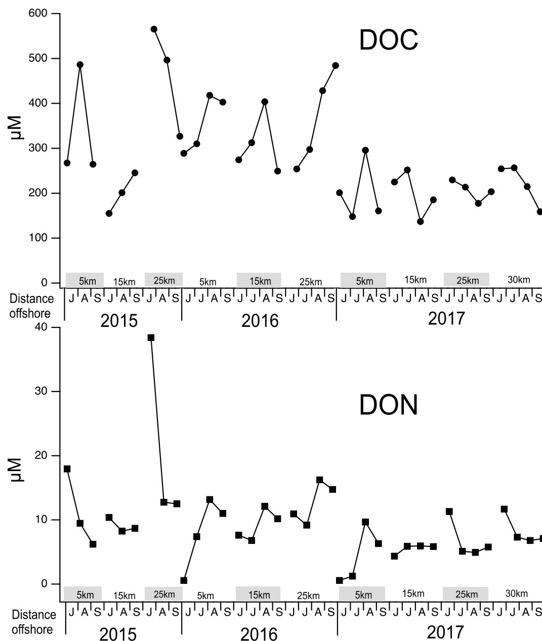
Supplementary Fig. 1 DOC and DON concentration detected at Transect Rompin, from 2015 to 2017. For Transect Rompin, the sampling period was Jul, Aug and Sep 2015 (JAS) and Jun, Jul, Aug and Sep in both 2016 and 2017 (JJAS).
