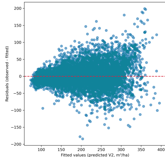
Svr Filtered Data - Residuals vs Fitted
