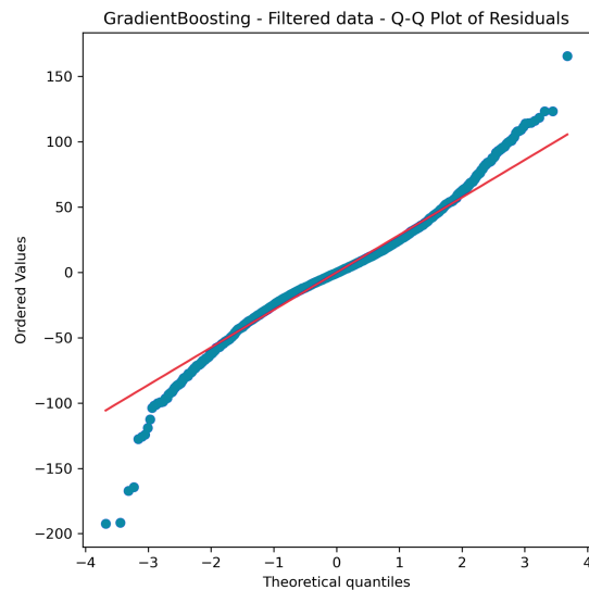
Gradientboosting Filtered Data - Q-Q Plot
