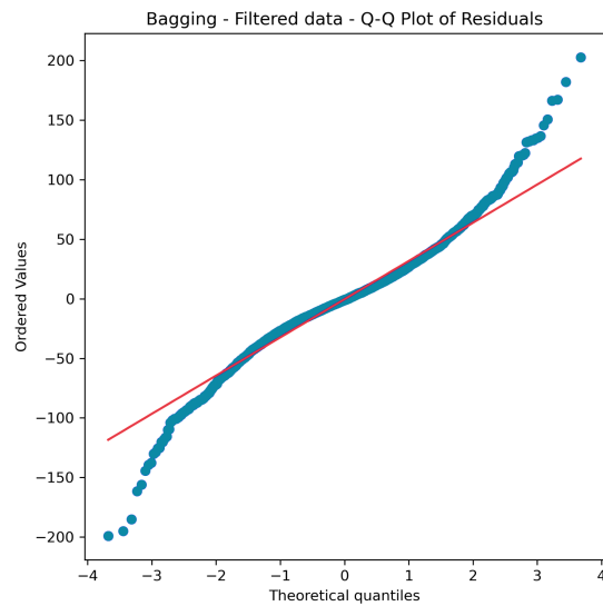
Bagging Filtered Data - Q-Q Plot
