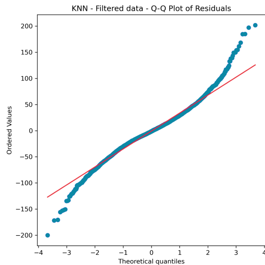
Knn Filtered Data - Q-Q Plot
