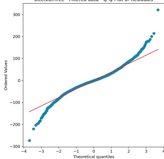
Decisiontree Filtered Data - Q-Q Plot
