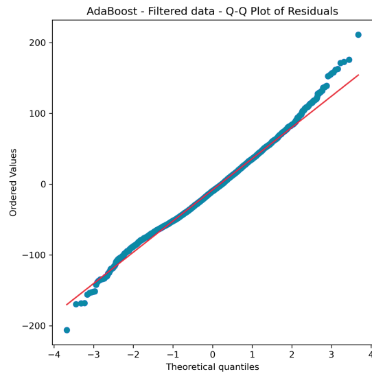
Adaboost Filtered Data - Q-Q Plot
