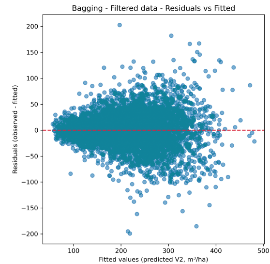
Bagging Filtered Data - Residuals vs Fitted
