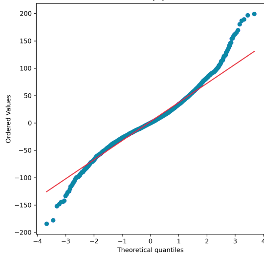
Svr Filtered Data - Q-Q Plot
