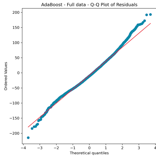
Adaboost Full Data - Q-Q Plot
