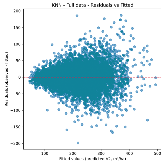
Knn Full Data - Residuals vs Fitted
