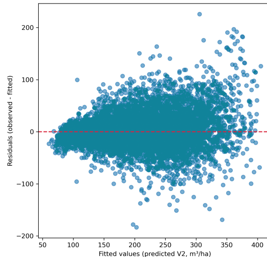
Svr Full Data - Residuals vs Fitted
