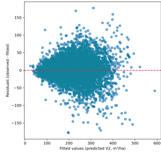
Mlp Full Data - Residuals vs Fitted
