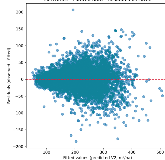
Extratrees Filtered Data - Residuals vs Fitted
