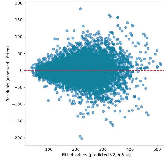
Randomforest Full Data - Residuals vs Fitted
