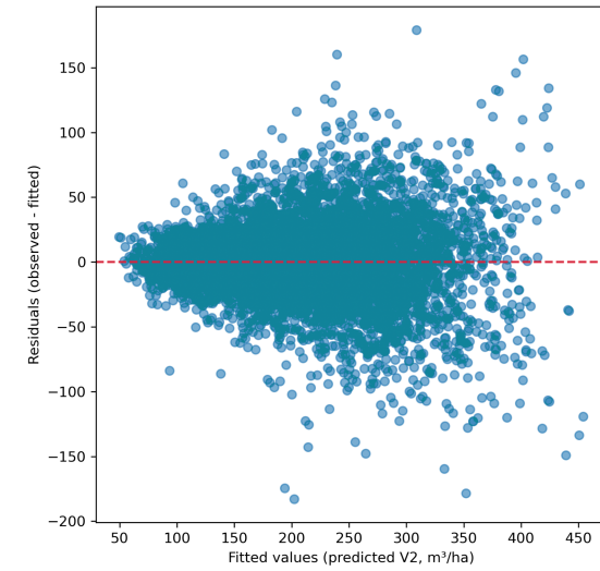
Mlp Filtered Data - Residuals vs Fitted
