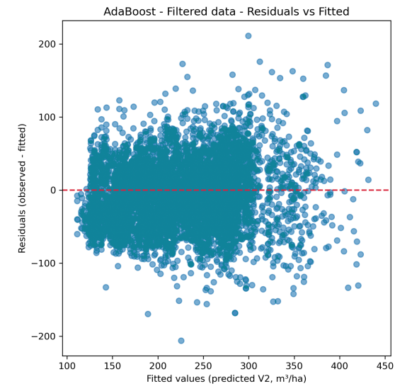
Adaboost Filtered Data - Residuals vs Fitted
