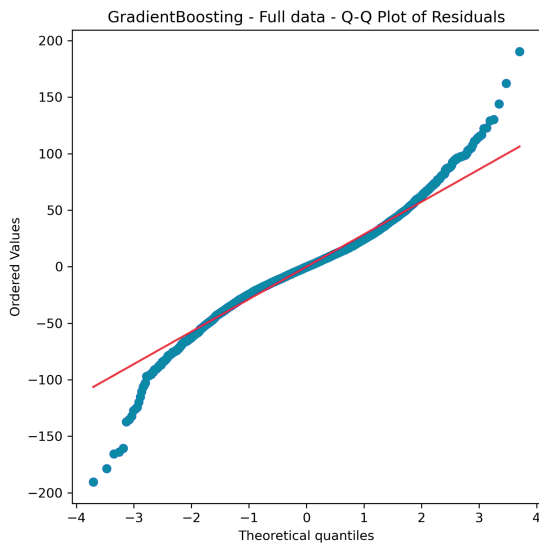
Gradientboosting Full Data - Q-Q Plot
