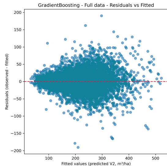
Gradientboosting Full Data - Residuals vs Fitted
