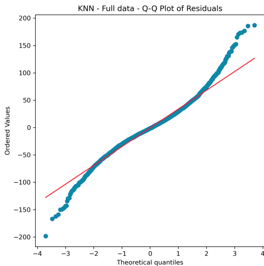
Knn Full Data - Q-Q Plot
