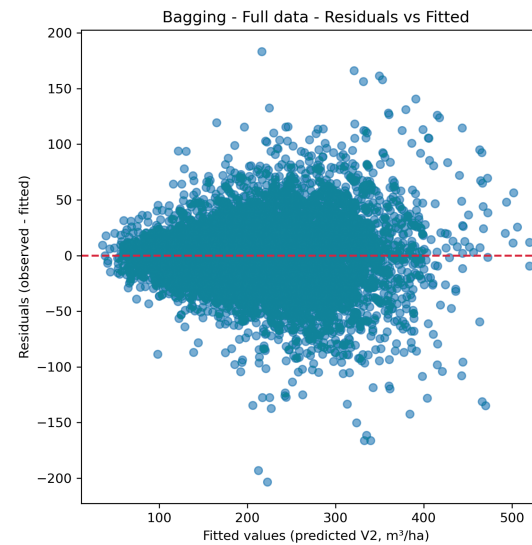
Bagging Full Data - Residuals vs Fitted
