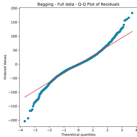
Bagging Full Data - Q-Q Plot
