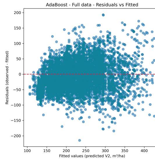
Adaboost Full Data - Residuals vs Fitted
