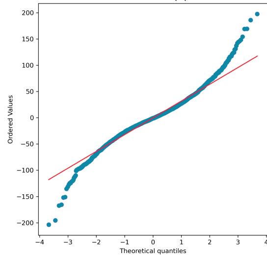
Randomforest Filtered Data - Q-Q Plot
