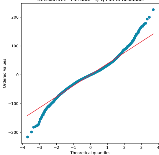
Decisiontree Full Data - Q-Q Plot
