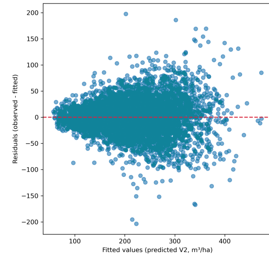
Randomforest Filtered Data - Residuals vs Fitted
