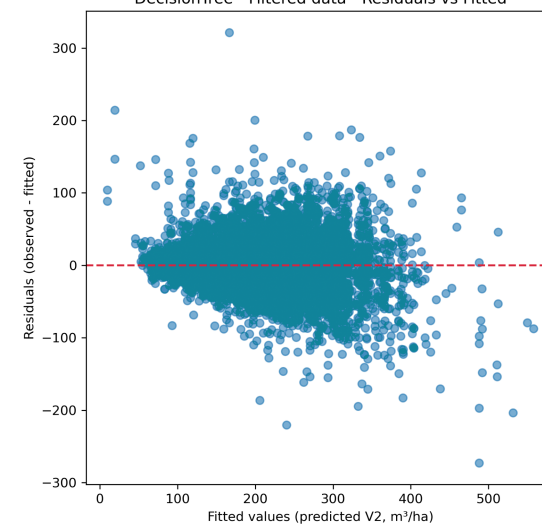
Decisiontree Filtered Data - Residuals vs Fitted
