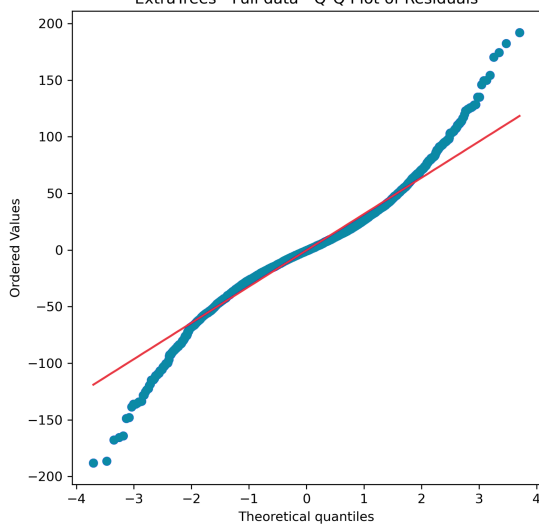
Extratrees Full Data - Q-Q Plot
