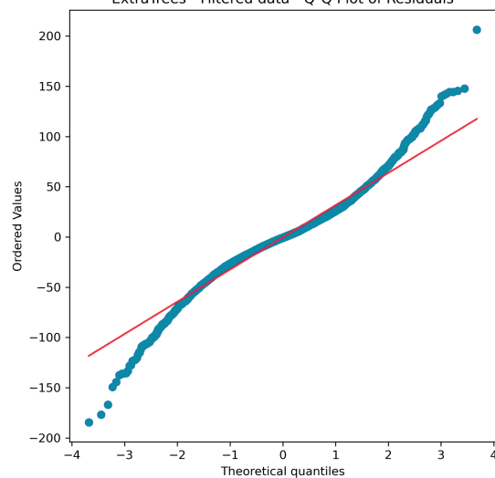
Extratrees Filtered Data - Q-Q Plot
