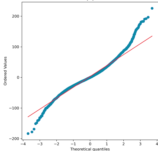
Svr Full Data - Q-Q Plot
