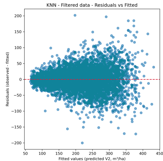
Knn Filtered Data - Residuals vs Fitted
