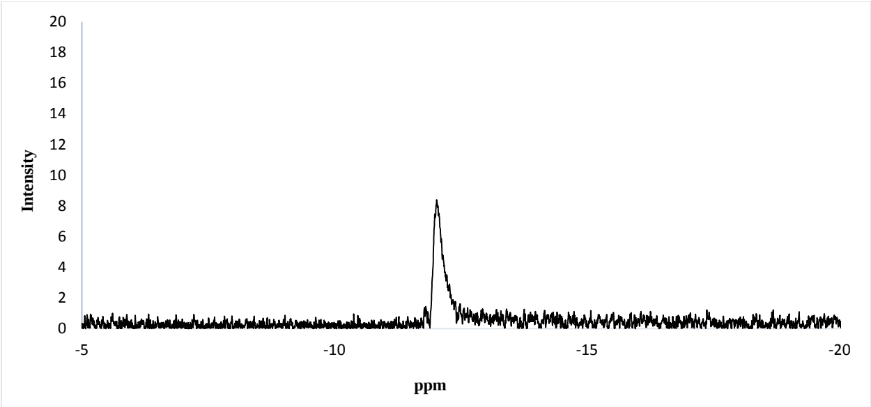
Fig. S8. ^{11}\text{B} NMR structure of complex 2
