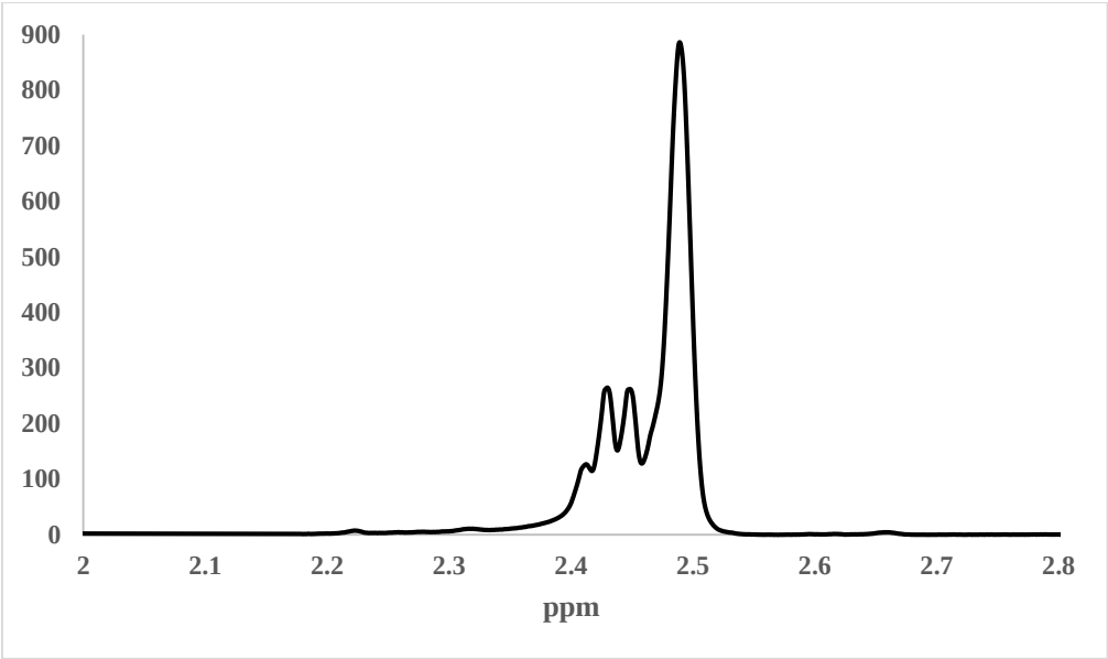
Fig.S1: ^1\text{H} NMR structure of \text{CH}_2 in complex 1
