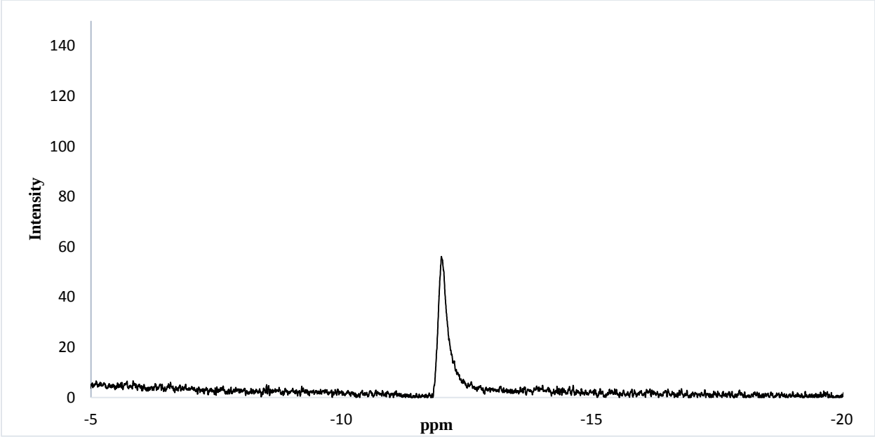
Fig. S7. ^{11}\text{B} NMR structure of complex 1
