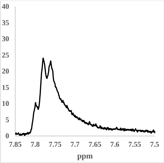
Fig. S5. 1 H NMR structure of CH-pyridine peak in complex 2
