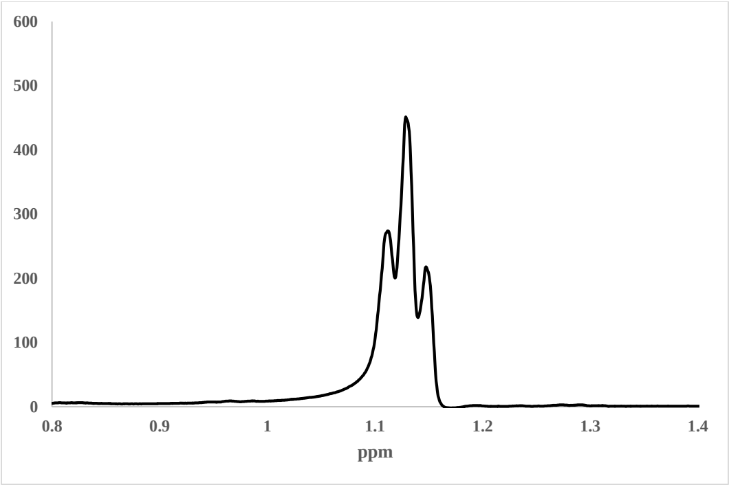
Fig. S2. 1 H NMR structure of CH 3 peak in complex 1
