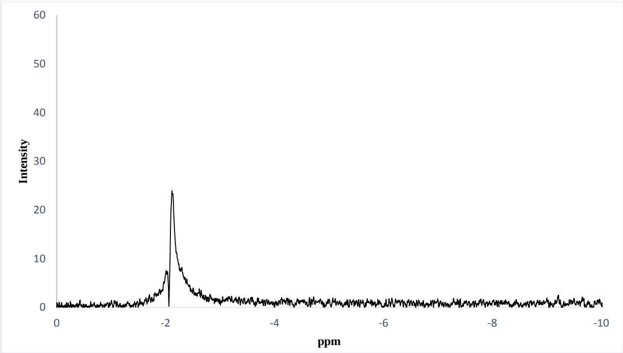
Fig. S10. ^{11}\text{B} NMR structure of complex 4
