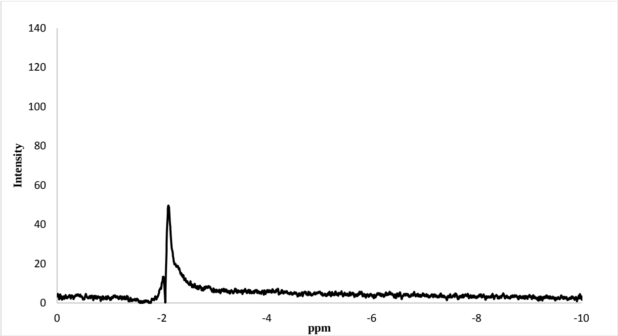
Fig. S9. ^{11}\text{B} NMR structure of complex 3
