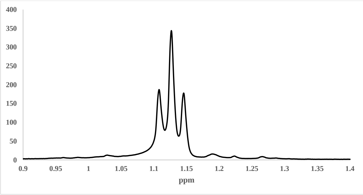
Fig. S4. 1 H NMR structure of CH 3 peak in complex 3
