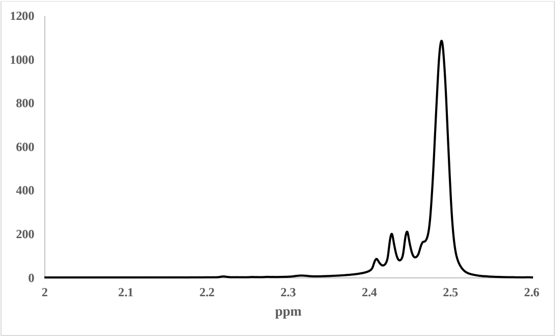
Fig. S3. ^1\text{H} NMR structure of \text{CH}_2 peak in complex 3
