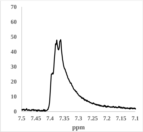
Fig. S6. 1 H NMR structure of CH-pyridine peak in complex 4
