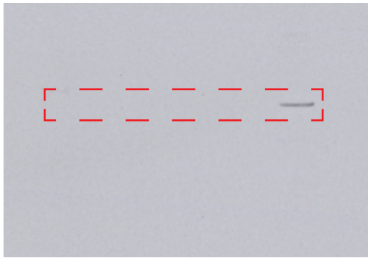
His-MBP-TBP
