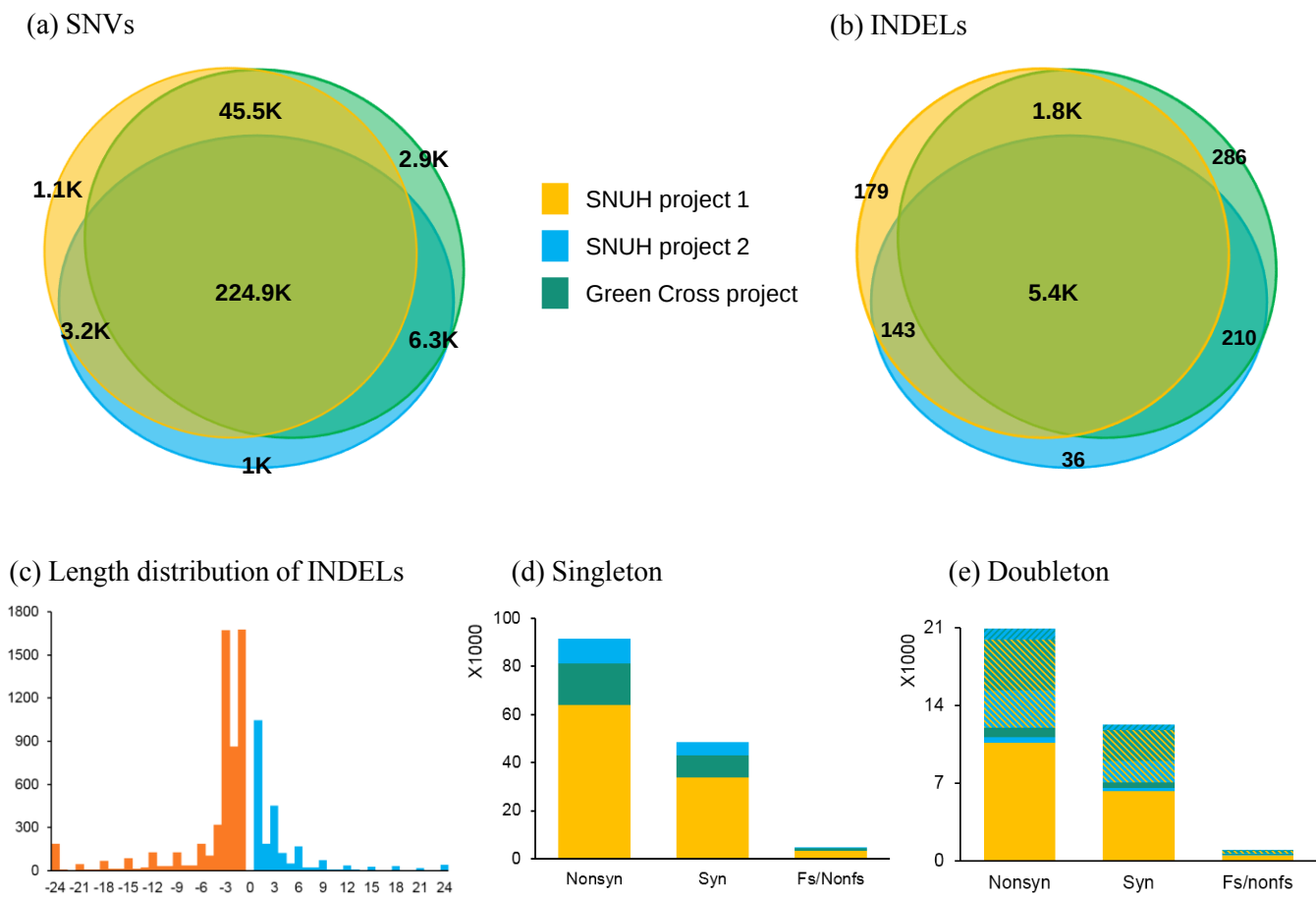
Supplementary Figure 1. Characteristics of CDS variants. Distribution of variants identified in each project on SNVs (a) and INDELs (b). Length distribution of INDELs (c). The number of frameshift insertion/deletion tends to increase. Number of singleton (d) and doubleton (e) variants of each cohort separated by exonic functional annotation. Colors and patterns indicate each cohort.
