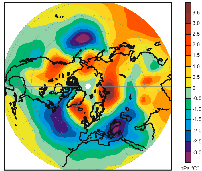
Figure S6 (Supplementary Figure 6) Relationship between the modelled sea surface temperature (SST) index of the coral region and the modelled sea level pressure (SLP) field of the Northern Hemisphere, based on the coupled atmosphere-ocean general circulation model ECHO-G. Regression of the modelled SST index covering the eastern Mediterranean and the Red Sea (see Supplementary Fig. S7 for definition) against the modelled Northern Hemisphere SLP field for the period 1820-1920 A.D. (December, January, February). Prior to the calculation the trends have been eliminated.
