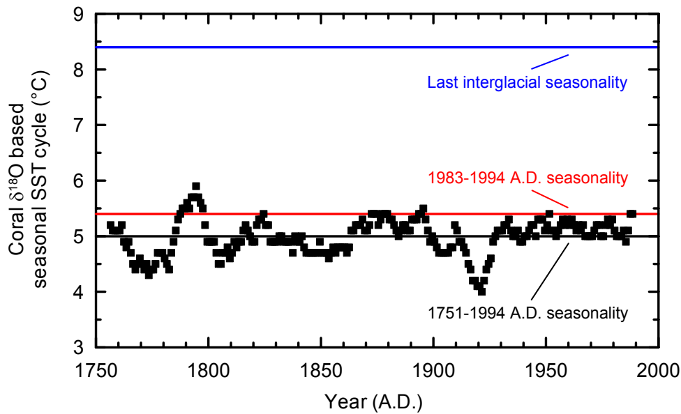
Figure S3 (Supplementary Figure 3) Coral \delta^{18}\text{O} based seasonal cycle of sea surface temperature (SST) in the northernmost Red Sea during the past centuries, compared with that of the last interglacial. The mean values of a 12 year moving window are shown (squares), based on the application of our coral \delta^{18}\text{O} -SST relationship (see Methods) to a modern coral record from Ras Umm Sidd 2 . Horizontal lines indicate means for the period 1751-1994 A.D. (black), the most recent 12 year window (red), and the 12 year window provided by the last interglacial coral (blue), respectively. There is no 12 year window during the past approximately 250 years during which the coral based seasonal SST cycle was as high as indicated by the last interglacial coral.
