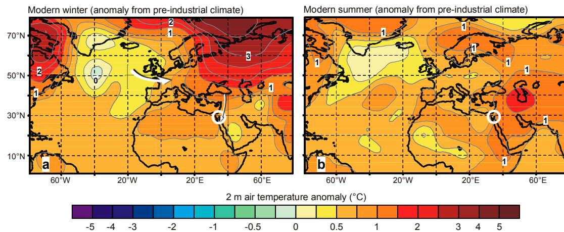
Figure S10 (Supplementary Figure 10) Near surface air temperature anomaly for modern climate based on the coupled atmosphere-ocean general circulation model ECHO-G, showing the anomalous temperature induced by the perturbation of anthropogenic greenhouse gases. Difference between modern (1975-1985 A.D.) and pre-industrial climate (1820-1850 A.D.) for a , winter (December, January, February) and b , summer (June, July, August). Near surface wind anomaly is schematically represented as white arrows. The greenhouse gas concentrations are based on ice core and instrumental records 11-14 . The region of coral collection in the northernmost Red Sea is marked by a white circle.
