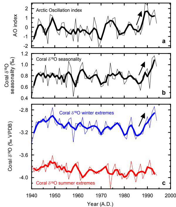
Figure S5 (Supplementary Figure 5) The Arctic Oscillation (AO) index 10 (January-March) and coral \delta^{18}\text{O} seasonality in the northernmost Red Sea over the past decades. a,b A shift toward the AO high index state from the mid-1980s to the early 1990s is accompanied by increased \delta^{18}\text{O} seasonality in a coral record from Ras Umm Sidd 2 . c , The latter results from a shift in the winter coral \delta^{18}\text{O} extremes toward colder/more arid conditions whereas the corresponding summer extremes remain relatively constant. This shows that a shift toward the AO/NAO high index state is accompanied by colder winters in the northernmost Red Sea, thereby increasing the seasonal cycle of temperature in this region. Correlations of the AO index (1940-1994 A.D.) with coral \delta^{18}\text{O} seasonality ( r = 0.47 ) and coral \delta^{18}\text{O} winter extremes ( r = 0.54 ) respectively are highly significant (99.9% level, 2-sided t-test). Bold lines represent 3 year running averages.
