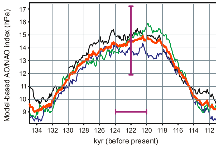
Figure S11 (Supplementary Figure 11) Modelled AO/NAO index for the last interglacial. Modelled AO/NAO index (December, January, February; DJF), defined as the sea level pressure difference between a southerly high pressure region and a northerly low pressure region (see Supplementary Fig. S7) for the last interglacial. A centred 41 year running mean for each of the three individual ensemble members has been applied (thin lines). The thick red line displays the ensemble mean. The vertical purple bar indicates the average and the mean standard deviation of the three experiments, taken from 41 years (DJF) marked by the horizontal purple bar (see Methods). The average (mean standard deviation) for 41 winters centred at 122 kyr, 3 kyr, and the pre-industrial period are 14.6 (5.3) hPa, 12.6 (4.8) hPa, and 11.7 (4.4) hPa, respectively (see also Fig. 3f).
