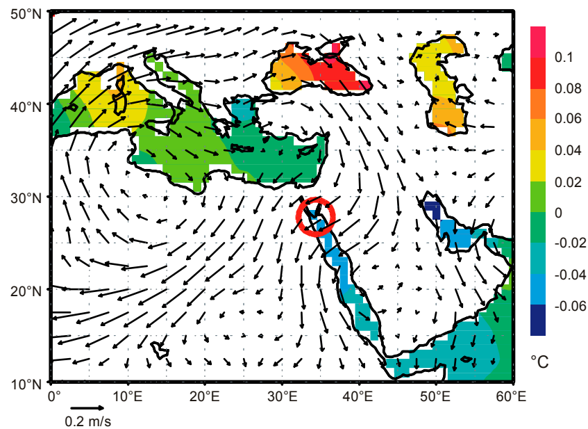
Figure S1 (Supplementary Figure 1) Relationship between a modern coral \delta^{18}\text{O} time series from the northernmost Red Sea (Ras Umm Sidd) 2 and the regional signature of the Arctic Oscillation in the Middle East 6 for interannual variability throughout the year. Regression of the 850 hPa wind field 7 and the sea surface temperature field 8 against the coral \delta^{18}\text{O} time series (1950-1994), performed for bimonthly, detrended, and normalized time series with the average seasonal cycle removed. All data were filtered in the 5-6 year band prior to analyses. The coral location is marked by a red circle.
