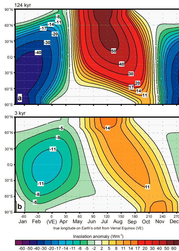
Figure S4 (Supplementary Figure 4) Insolation anomalies for the last interglacial and the late Holocene. Annual distribution of insolation anomaly relative to modern conditions for a , 124 kyr ago and b , 3 kyr ago, calculated after ref. 9. Shown is the latitudinal distribution with respect to the true longitude (angle between perihelion and vernal equinox on the Earth's orbit). Note that following Kepler's Law the track speed on the elliptical orbit varies.
