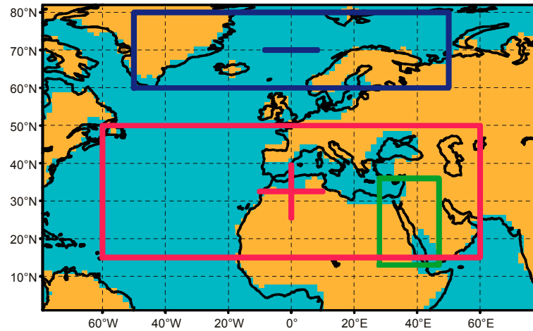
Figure S7 (Supplementary Figure 7) Definition of modelled indices used in this study. The sea surface temperature (SST) index of the coral region (Fig. 3c, e) has been obtained from the averaged modelled SST over the eastern Mediterranean and the Red Sea (28°-47° E; 13°-36° N; green box). The modelled AO/NAO index (Fig. 3f) is calculated from the sea level pressure (SLP) difference between a southerly high pressure region (60° W-60° E; 15°-50° N; red box with plus sign) and a northerly low pressure region (50° W-50° E; 60°-80° N, blue box with minus sign). The brown rectangles mark the sea-land-mask of the atmospheric submodel ECHAM4 in its T30 resolution.
