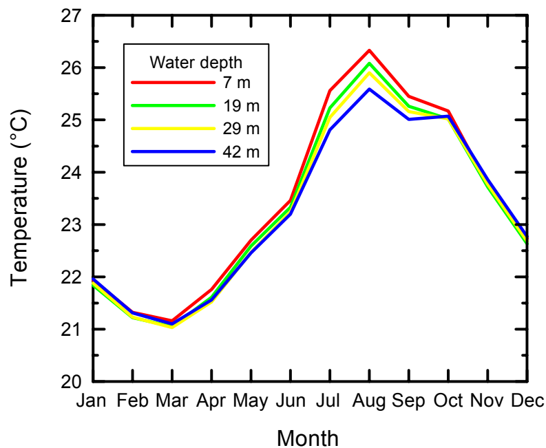
Figure S2 (Supplementary Figure 2) Mean monthly water temperature in the northernmost Red Sea over the depth range of Porites coral growth. The seasonal cycle of temperature decreases with water depth by about 0.7 °C between 7 and 42 m depth. This results from a weak stratification of the water column during summer. During winter the water column is well mixed. Our modern reference corals are from shallow waters (4 to 18 m). Consequently, the increased temperature seasonality documented by the last interglacial coral can not be explained by a relative difference in paleo-depth. Data are based on hourly measurements of four temperature loggers which were deployed along the reef slope at Aqaba for the period May 1999 to November 2001.
