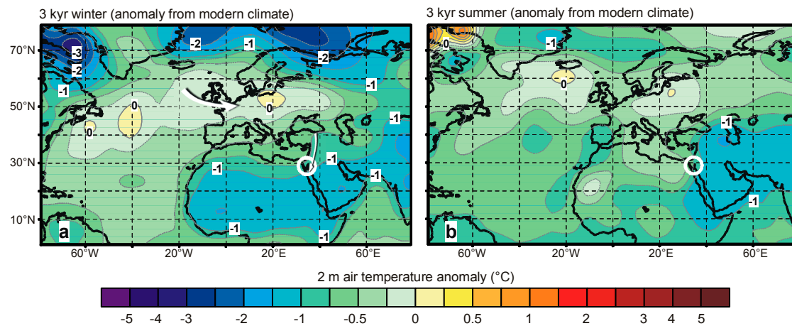
Figure S9 (Supplementary Figure 9) Near surface air temperature anomaly for the late Holocene based on the coupled atmosphere-ocean general circulation model ECHO-G. Difference between late Holocene (3 kyr) and modern climate (1975-1985 A.D.) for a , winter (December, January, February) and b , summer (June, July, August). The corresponding anomalies from pre-industrial climate are shown in Fig. 4c, d. Near surface wind anomaly is schematically represented as white arrows. An average of 11 simulation years has been applied to the late Holocene climate centred at 3 kyr. The region of coral collection in the northernmost Red Sea is marked by a white circle.
