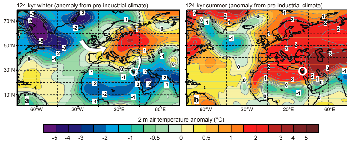
Figure S8 (Supplementary Figure 8) Near surface air temperature anomaly for the last interglacial based on the coupled atmosphere-ocean general circulation model ECHO-G. Difference between last interglacial (124 kyr) and pre-industrial climate (1820-1850 A.D.) for a , winter (December, January, February) and b , summer (June, July, August). The corresponding anomalies from modern climate are shown in Fig. 4a, b. Near surface wind anomaly is schematically represented as white arrows. An average of 11 simulation years has been applied to the last interglacial climate centred at 124 kyr. The region of coral collection in the northernmost Red Sea is marked by a white circle.
