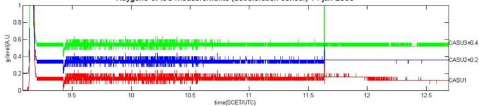
Huygens RASU Radial accelerometer measurements (spin sensor) 14-jan-2005
