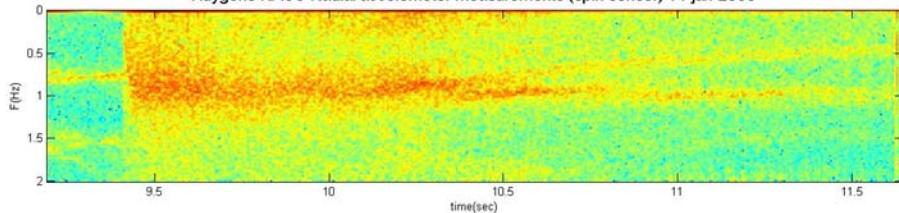
Huygens RASU Radial accelerometer measurements (spin sensor) 14-jan-2005
