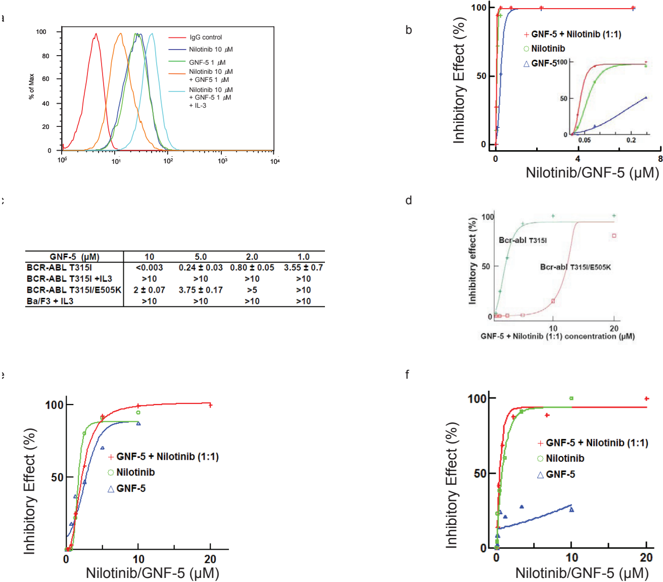
Supplementary Figure 6. Inhibition of GNF-5 and combination with nilotinib. a , Inhibition of STAT5 phosphorylation in T315I Bcr-Abl Ba/F3 cells in the presence of nilotinib (10 μM) or GNF-5 (1 μM) alone or in combination. Inhibition of STAT5 phosphorylation is reversed upon addition of interleukin-3 (IL-3). b , Nilotinib and GNF-5 exhibited cooperativity for inhibition of wild-type Bcr-Abl transformed BaF3 cells with a calculated combination index of 0.61. An enlargement of the region where cooperativity between the agents is apparent is shown in the right corner. The combination curve (red) contains twice the total drug concentration of the single agent curves due to the presence of both drugs. c , Nilotinib's anti-proliferative EC 50 in the presence of 1 to 10 μM GNF-5 on Ba/F3 cells expressing T315I Bcr-Abl. d , Effects of GNF-5 in combination with varying concentrations of nilotinib (0.6-20 μM) on the proliferation of T315I Bcr-Abl and T315I/E505K Bcr-Abl expressing Ba/F3 cells e , Effects of GNF-5, nilotinib, and varying concentrations of GNF-5 in combination with nilotinib (0.3-10 μM) on the proliferation of T315I Bcr-Abl Ba/F3 cells. Note that the combination curve (red, as well in f ) shows the total combined concentration of both drugs and the actual dosage of each drug was only half that present in the corresponding single agent curves. Plots e and f represent the same data as shown in Figure 4a and c respectively but are replotted here so the single agent and combination curves can be compared on the basis of equal amounts of total drug. f , Percent inhibition of T315I Abl kinase by nilotinib, GNF-5, or the combination.
