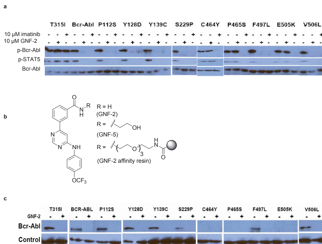
Supplementary Figure 4. Characterization of GNF-2 resistance mutations a , The ability of GNF-2 or imatinib (10 \mu M) to inhibit cellular Bcr-Abl kinase activity in wild-type and mutant expressing cells was tested by monitoring phospho-Bcr-Abl and phospho-STAT5 following treatment of cells with inhibitor for 2 hours. b , Chemical structures of GNF-2, GNF-5, and GNF-2-Affigel-10. c , Ability of wild-type and mutant Bcr-Abl to bind to GNF-2 affinity support. Western blot with the anti-Abl antibody K-12 detects the amount of wild type or mutant Bcr-Abl from cell lysates retained on the GNF-2 affinity resin in the presence or absence of 50 \mu M competitive GNF-2.
