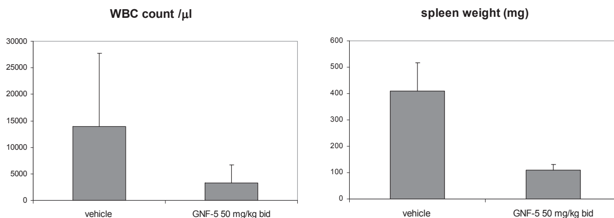
Supplementary Figure 14. GNF-5 treatment normalizes blood counts and spleen size of Bcr-Abl BMT mice. Bone marrow cells from donor mice pretreated with 5-fluorouracil (5-FU) were transduced with a wild-type Bcr-Abl retroviral vector and transplanted into irradiated recipient mice. Seven days after transplantation, a dose regimen consisting of 50 mg/kg GNF-5 twice daily or vehicle was administered during seven days. Peripheral blood cell counts measured on the last day of treatment were high, with 95% neutrophils or blast cells, in the vehicle treated mice, consistent with development of CML-like disease. In contrast, GNF-5 treated mice showed normal blood cell counts. The spleen size from the vehicle group was increased 3- to 4-fold compared to those of normal mice (normal spleen weight: 80-90 mg), while GNF-5 treated mice had normal spleen weights. Error bars are s.e.m.
