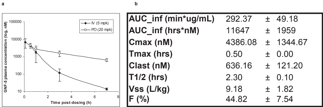
Supplementary Figure 11. GNF-5 pharmacokinetic parameters in mice. Following an oral dose of 20 mg/kg to Balb/C mice, GNF-5 appeared rapidly in the circulation to attain a maximum concentration of 4.4 \pm 1.3 \mu\text{M} at 0.5 h, decreasing to 0.63 \pm 0.12 \mu\text{M} after 7 hours, with a terminal half-life of 2.3 hours; oral bioavailability was 44.8 \pm 7.5\% . In SCID mice, as used for efficacy studies in the xenograft model, the pharmacokinetic profile in plasma was similar to that observed in normal mice. a , GNF-5 plasma concentration (nanomolar) versus time (hours) following intravenous and oral doses of 5 mg/kg and 20 mg/kg, respectively. b , Pharmacokinetic parameters: AUC = area under the curve (measure of exposure), C_{\text{max}} = maximum plasma concentration, T_{\text{max}} = time of maximum plasma concentration, C_{\text{last}} = concentration at last measured time point, T_{1/2} = time required for plasma concentration to reach half of the highest concentration, V_{\text{ss}} = volume of distribution, F = percentage oral bioavailability.
