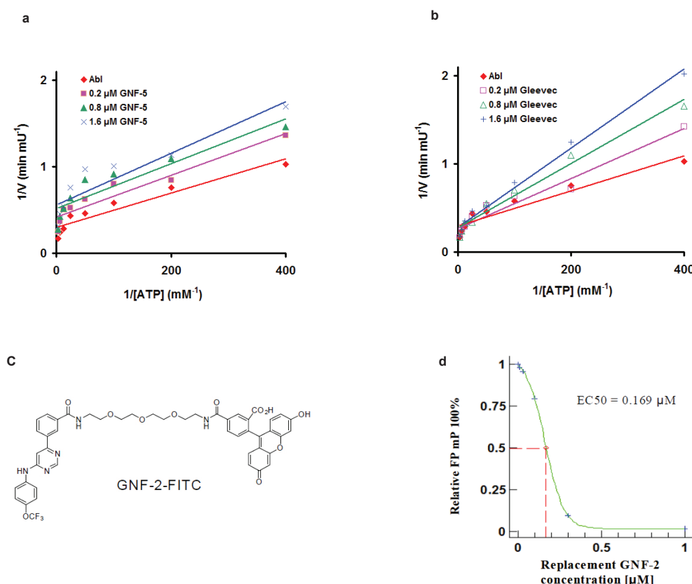
Supplementary Figure 9. GNF-5 inhibits Abl kinase in a non-ATP competitive fashion a , Abl kinase activity was measured in a PEP-LDH coupled assay at different ATP concentrations, using formation of NAD as the indicator of reaction. Enzyme activity was measured in the presence of 0, 0.2, 0.8, and 1.6 μM GNF-5 with increasing concentrations of ATP. b , As in a with imatinib instead of GNF-5. Each data point is the average of three independent experiments. Data are plotted in double-reciprocal form to determine K_m and V_{max} with ATP concentration ranging from 2.5 to 160 μM. For imatinib (Gleevec), the value is constant at 4.18 \pm 0.5 , 4.46 \pm 0.5 , and 4.25 \pm 0.6 mU min -1 in the presence of 0, 0.2, and 0.8 μM imatinib concentrations, respectively. This is as expected for an ATP-competitive inhibitor. In contrast, V_{max} decreases with increasing concentrations of GNF-5, and these effects are clearly seen in the double-reciprocal plot. For GNF-5, the value of V_{max} decreases from 4.18 \pm 0.5 in the absence of GNF-5 to 2.43 \pm 0.2 and 2.2 \pm 0.2 mU min -1 in the presence of 0.2 and 0.8 μM GNF-5, respectively. These kinase assay results demonstrate that the mechanism of Abl inhibition by GNF-5 is non-competitive with respect to ATP and that no additional co-factors are needed to observe inhibition in vitro . c , Fluorescence polarization titration of GNF-2 with wild-type Abl using GNF-2-FITC. Chemical structure of GNF-2-FITC modified compound. d , Fluorescence polarization titration of GNF-2 with wild-type Abl using GNF-2-FITC probe yields and EC 50 of 169 nM.
