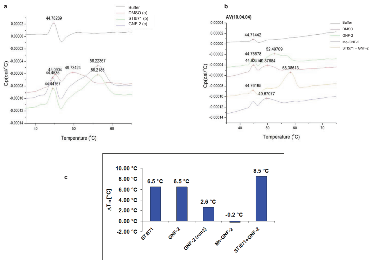
Supplementary Figure 15. Differential scanning calorimetry (DSC). a. Samples consisting of 1mg/ml of wt Abl (46-531) mixed with DMSO or imatinib (STI571) at 10 \mu M final concentration or GNF-2 at 20 \mu M final concentration in 20mM Tris pH 8.0, 5% glycerol, 1mM TCEP buffer were subjected to DSC. The results indicate that both STI-571 and GNF-2 bind to Abl (46-531). b. Samples consisting of 1mg/ml of wt Abl (46-531) mixed with DMSO, GNF-2, or Me-GNF-2 (inactive analog of GNF-2) at 20 \mu M final concentration, or 1mg/ml of wt Abl (46-531) pre-incubated with imatinib at 10 \mu M for 30 min and to which GNF-2 was added at 20 \mu M final concentration were subjected to DSC. c. The increase in melting temperature observed in the presence of both compounds suggests strongly that binding of both compounds causes additional stabilization of the kinase relative to the kinase bound to only one of the compounds.
