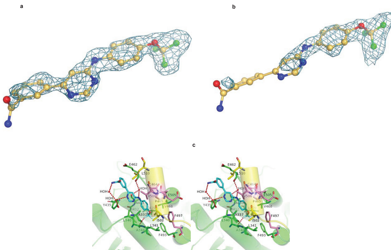
Supplementary Figure 1. Difference electron density and crystal structure for GNF-2 bound to Abl kinase. The F_o - F_c Fourier map, calculated before fitting the ligand to the model, is contoured at 3.0 \sigma for the two molecules of GNF-2 in the asymmetric unit. Density for molecule a is shown on the left and that for molecule b on the right. c , Stereo view of the GNF-2-Abl interactions: Abl kinase is indicated in green (helices indicated with transparent cylinders) with the bent part of the I-helix in yellow, GNF-2 resistance mutations in pink, and GNF-2 carbons in cyan. H-bonding and other polar interactions are indicated by dotted red lines. A water molecule forms a hydrogen bond bridge between the aniline NH and the main chain carbonyls of A433 and E462 in both the fully and partially occupied myristate binding sites in the crystal. Residues contacting GNF-2 at the base of the pocket are L341 and A344 from \alpha E , I432 from \alpha F , V468 from \alpha H , F493 from \alpha I and I502 from \alpha I' . The surface in the central part of the pocket is formed by A337 from \alpha E , C464 and P465 from the start of \alpha H , A433 from \alpha F , and V506 from \alpha I' . There are fewer interactions at the mouth of the pocket (Y435 from \alpha F , E462 from the loop before \alpha H and L510 at the end of \alpha I' ), which is reflected in the weak electron density and hence flexibility of the benzamide part of GNF-2. Mutations, C464Y, P465S, and V506L presumably confer direct steric hindrance to the binding of GNF-2, while F497L and E505K are in the second shell of residues forming the binding site, and are likely to have an indirect unfavorable steric effect. The overall structure of the Abl kinase domain complexed to GNF-2 is similar to that of the myristate complex, except for the positions of residues between F497 and S501 which are shifted by up to 4 \text{ \AA} . This is due to crystal contacts between this part of the structure and a neighboring molecule in the crystal. GNF-2 does not affect the myristate binding site but the SH2-docking surface is altered to prevent clash between its helix \alpha A and the ligand. There is also a very small rotation of the N-terminal lobe of the kinase with respect to the C-terminal lobe, but this may also be due to slight changes in crystal packing due to the replacement of the myristoylated peptide. There is very little difference between the relative orientations of these lobes when comparing the Abl/imatinib complex 7 with the Abl/imatinib/myristate complex 1,8 .
