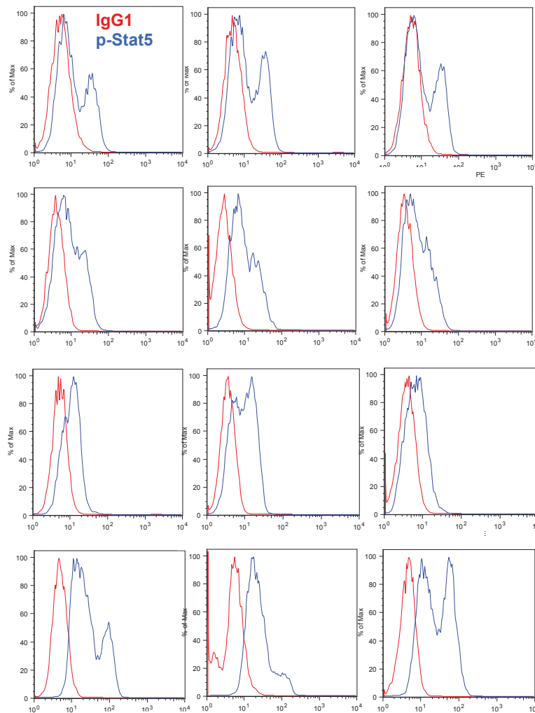
Supplementary Figure 13. GNF-5 efficacy correlates with inhibition of Bcr-Abl-mediated STAT5 phosphorylation. Phospho-STAT5 (blue curves) was monitored by FACS at various time-points and doses (indicated on left). Each box corresponds to an individual animal.
