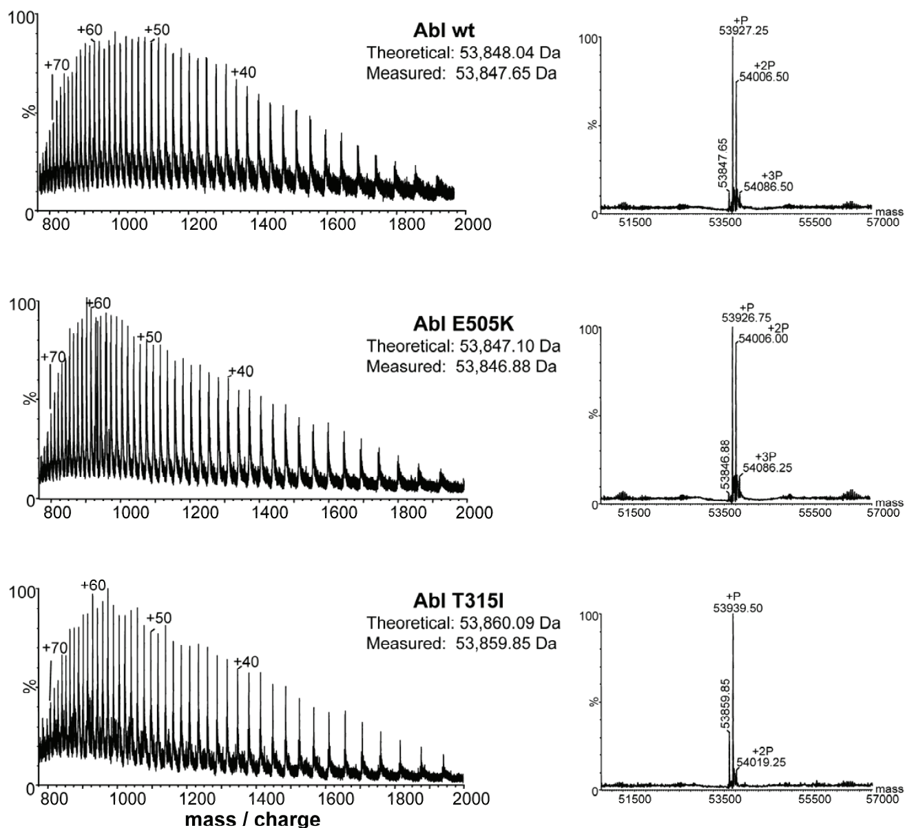
Supplementary Figure 8. Mass spectra of the Abl proteins: wild-type, E505K, and T315I. The raw m/z data are shown on the left, and the transformed, mass only spectra shown on the right. The measured and theoretical molecular weights of the unmodified form of each protein are indicated. In the transformed mass spectra, peaks corresponding to each phosphorylation are indicated.
