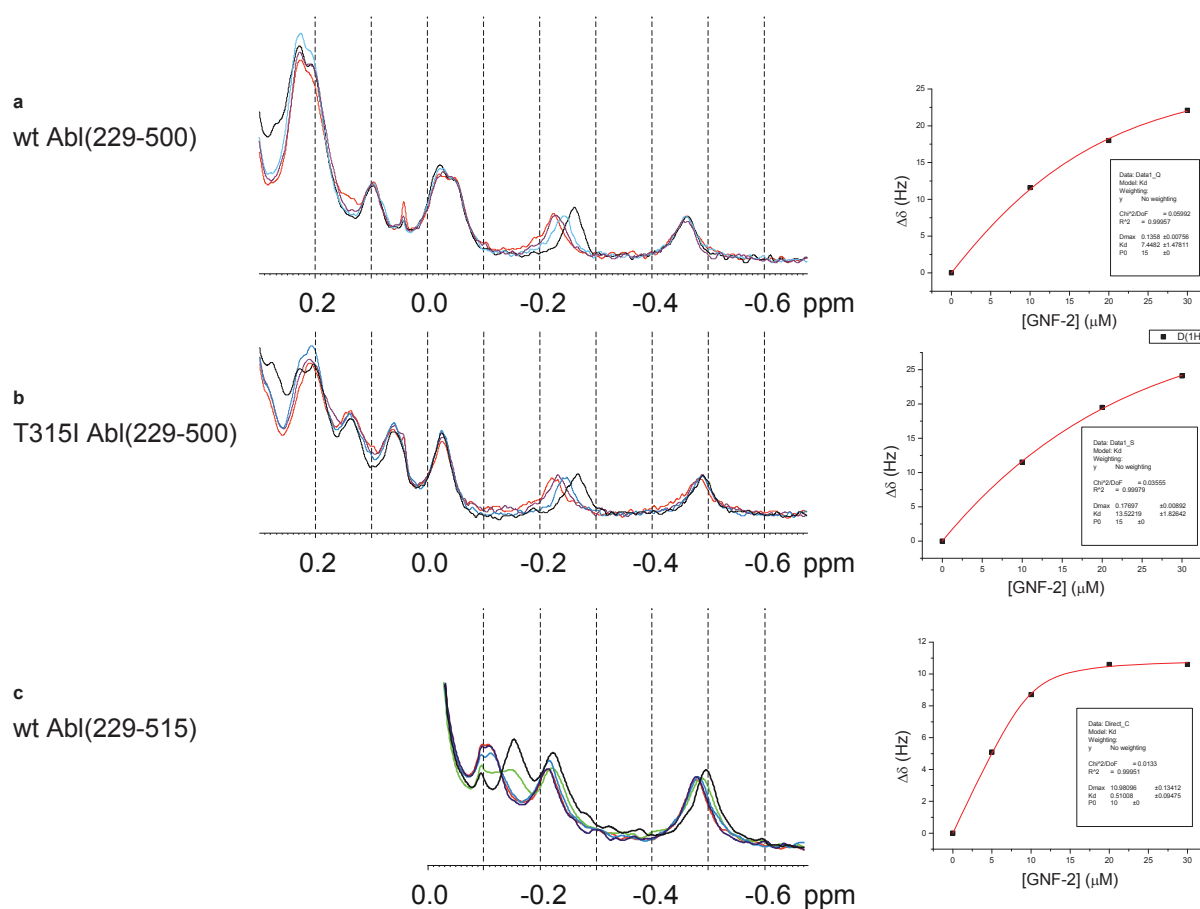
Supplementary Figure 5. NMR-detected titration of GNF-2 to Abl complexes. The upfield parts of NMR spectra are shown (left) which include an Abl methyl group near the myristate pocket. Chemical shift changes of this methyl group are followed as GNF-2 is added at concentrations up to its solubility limit of 30 \mu M. The chemical shift changes plotted versus GNF-2 concentration directly yield the dissociation constant (right). a , 15 \mu M wildtype Abl(229-500), b , 15 \mu M T315I Abl(229-500), c , 10 \mu M wildtype Abl(229-515). Although binding of GNF-2 to wt Abl(229-515) shows signs of slow to intermediate exchange for some resonances, the K_D could be unambiguously determined: 0.5 \pm 0.1 \mu M for GNF-2 binding to the imatinib/Abl complex using the full-length catalytic domain (residues 229-515; Abl 1a numbering – panel c), and 7.4 \pm 1.5 \mu M using the imatinib/Abl complex with a C-terminal truncated form of Abl (residues 229-500) not including helix I (panel a) and 13.5 \pm 1.8 \mu M using the T315I mutant of a C-terminal truncated form of Abl (residues 229-500) not including helix I (panel b). The lower affinity to the (229-500) construct is probably due to the lack of helix I, which lines the myristate pocket and is involved in interactions with GNF-2.
