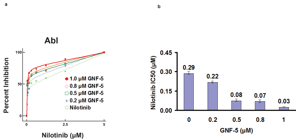
Supplementary Figure 10. Enzymatic inhibition of wild-type Abl kinase by combination treatments. a , Inhibition of wild-type Abl kinase activity by nilotinib in the presence of increasing concentrations of GNF-5. b , \text{IC}_{50} values for inhibition of wild-type Abl by nilotinib with increasing concentrations of GNF-5. Error bars are s.e.m.
