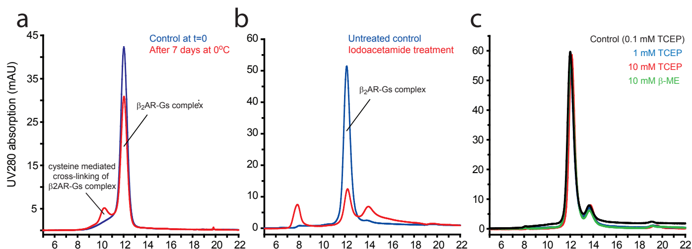
Figure S12: Effect of alkylating and reducing agents on the stability and aggregation of the \beta_2 AR-Gs complex.
