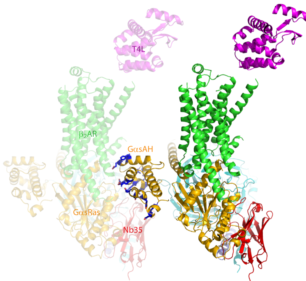
Figure S5: Packing interactions of G \alpha sAH domain
