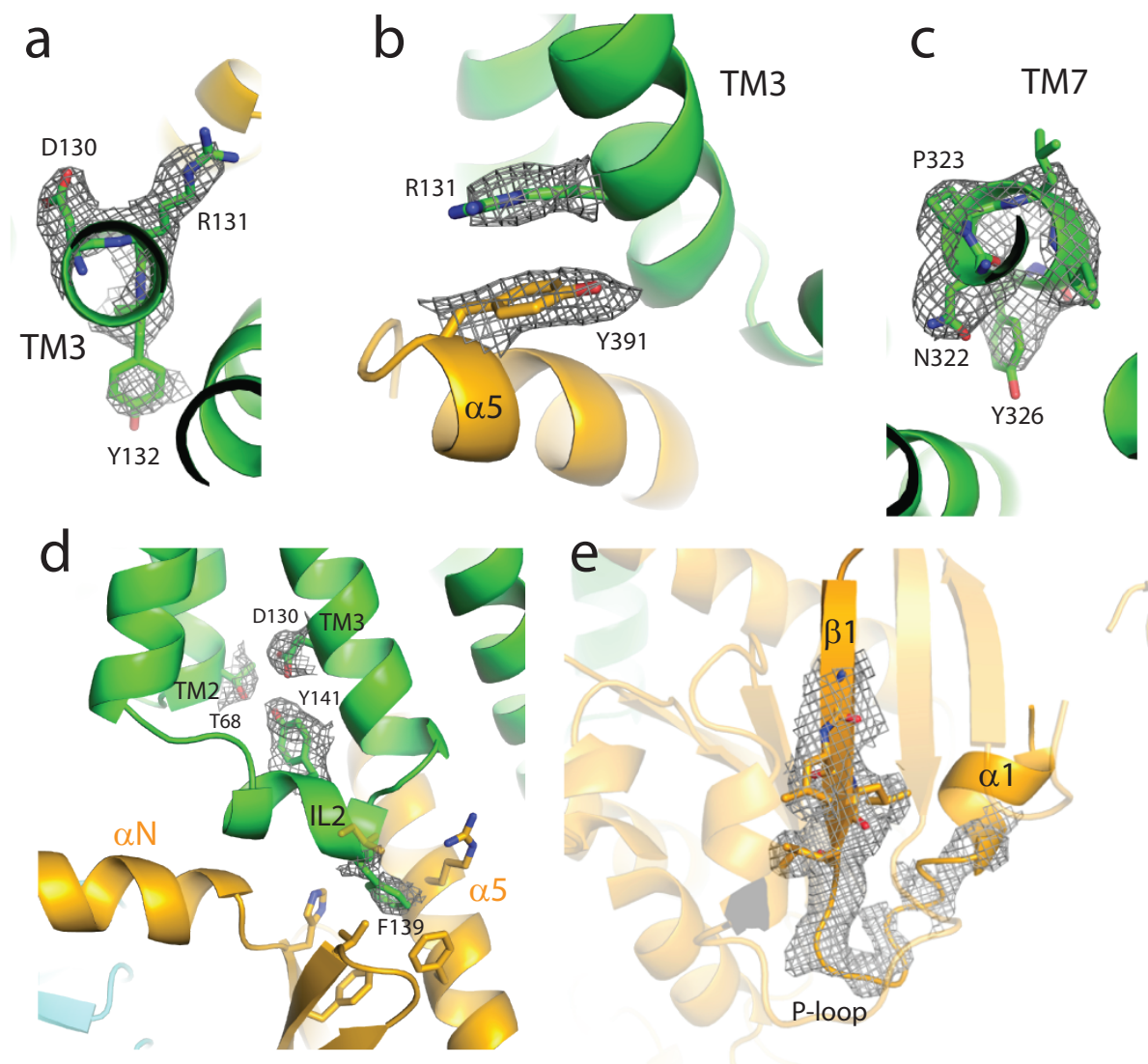
Figure S3: Views of electron density for residues in the \beta_2 AR-Gs interface.
