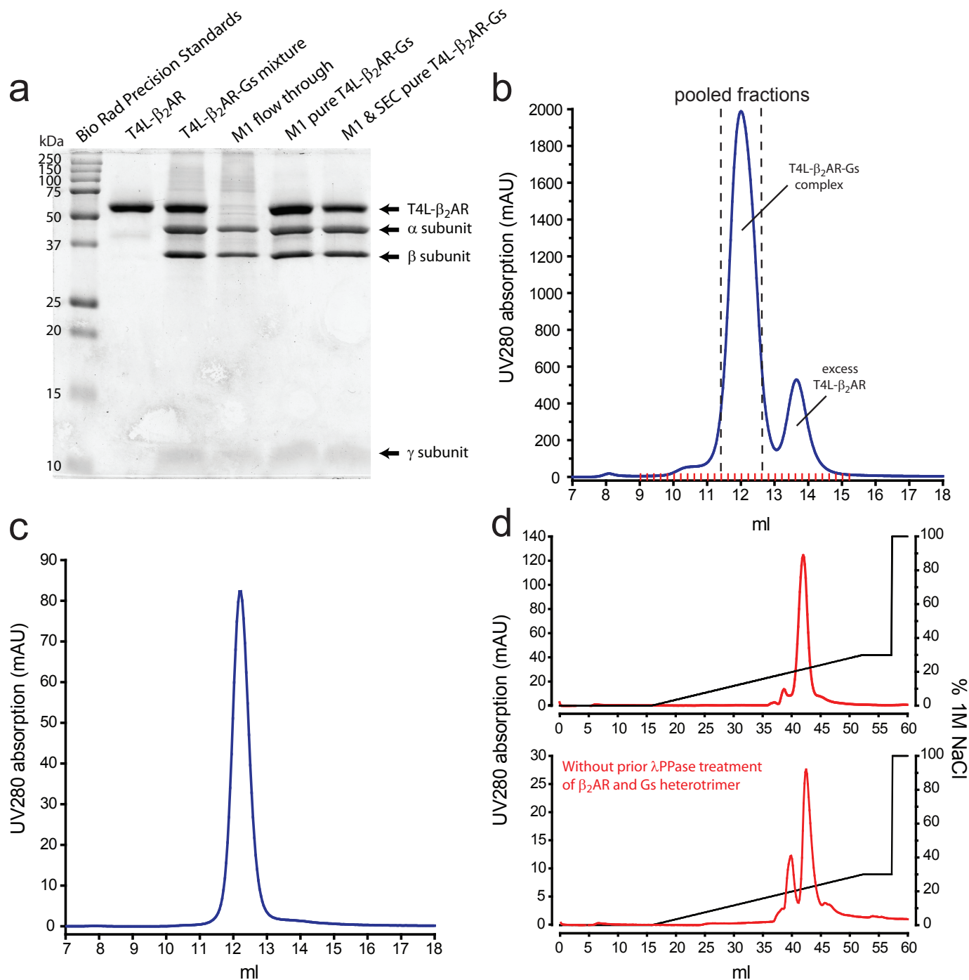
Figure S8: Purity and homogeneity of the \beta_2 AR-Gs complex
