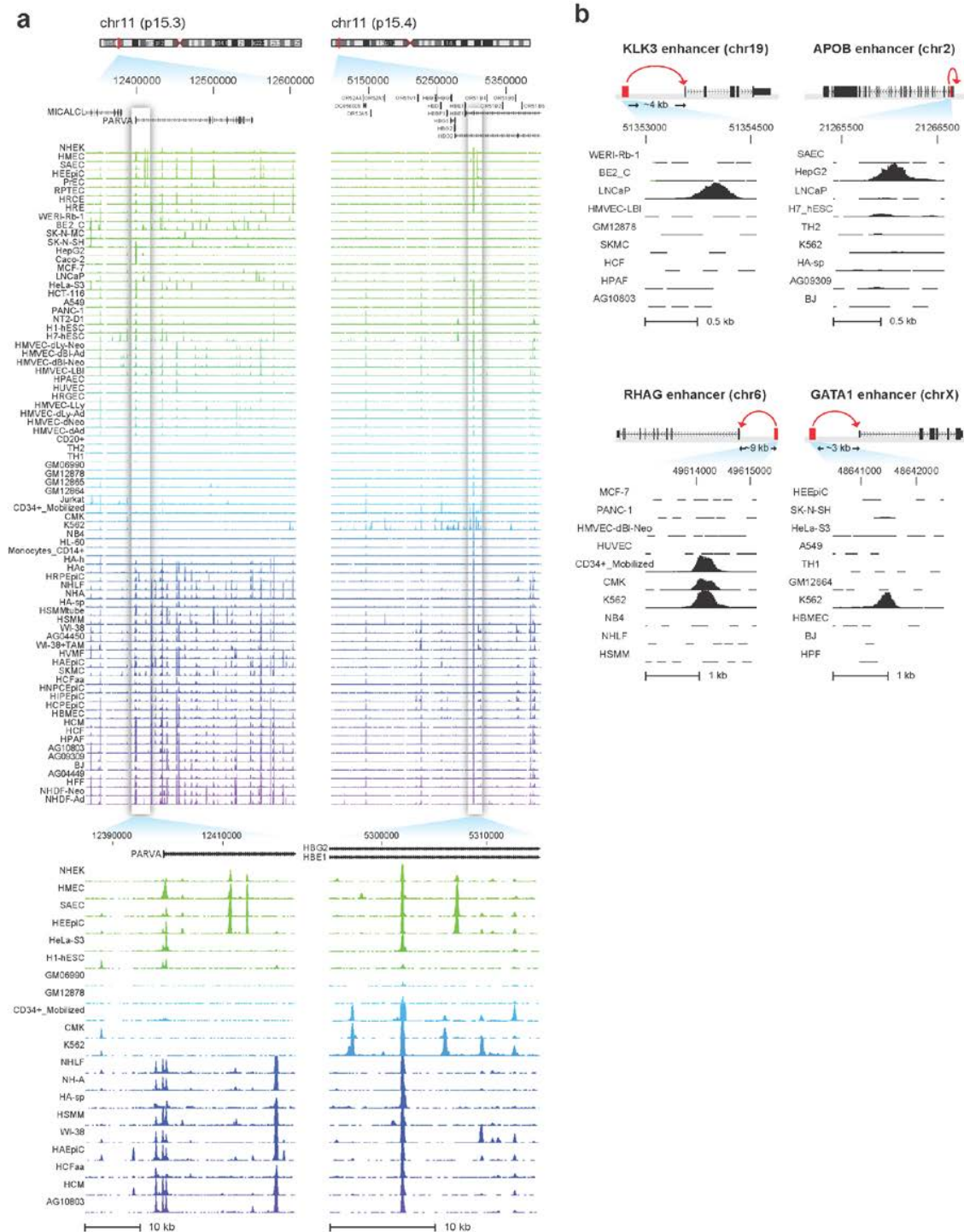
Supplementary Figure 2. (a) This is a subset of the data shown in Supplementary Fig. 1, providing greater visual detail. Data for 77 of the 125 cell types is shown. (b) Examples of known cell-selective enhancers. Shown above each set of DNaseI data are schematics showing enhancer location (red) relative to the gene it controls.
