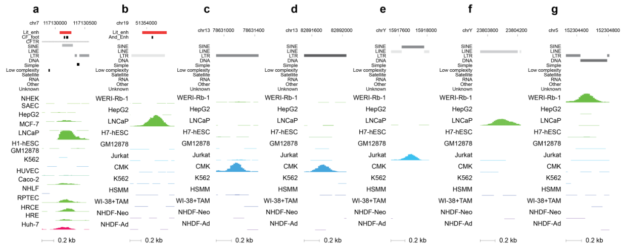
Supplementary Figure 4. Examples of DHSs in repetitive elements. Panels (a) and (b) show data for two well-characterized enhancers which lie in repeat-masked sequence. A CFTR enhancer 3 is shown in panel (a). A red bar marks the position of the literature enhancer which largely overlaps a SINE element. In vitro footprints observed at the enhancer are shown below the red bar, in black. The enhancer has been previously reported in Caco-2 and Huh7 cells. We observe a strong signal in LNCaP also. The PSA enhancer of the KLK2 gene 4 shown in panel (b) largely overlaps an LTR element. A red bar marks the known site and a black bar below marks the observed in vitro footprint. A strong DHS is observed in the expected cell type, LNCaP, but not in other cell types. Panels (c)-(g) are examples of DHSs primarily overlapping LTR, SINE, LINE, and DNA elements.
