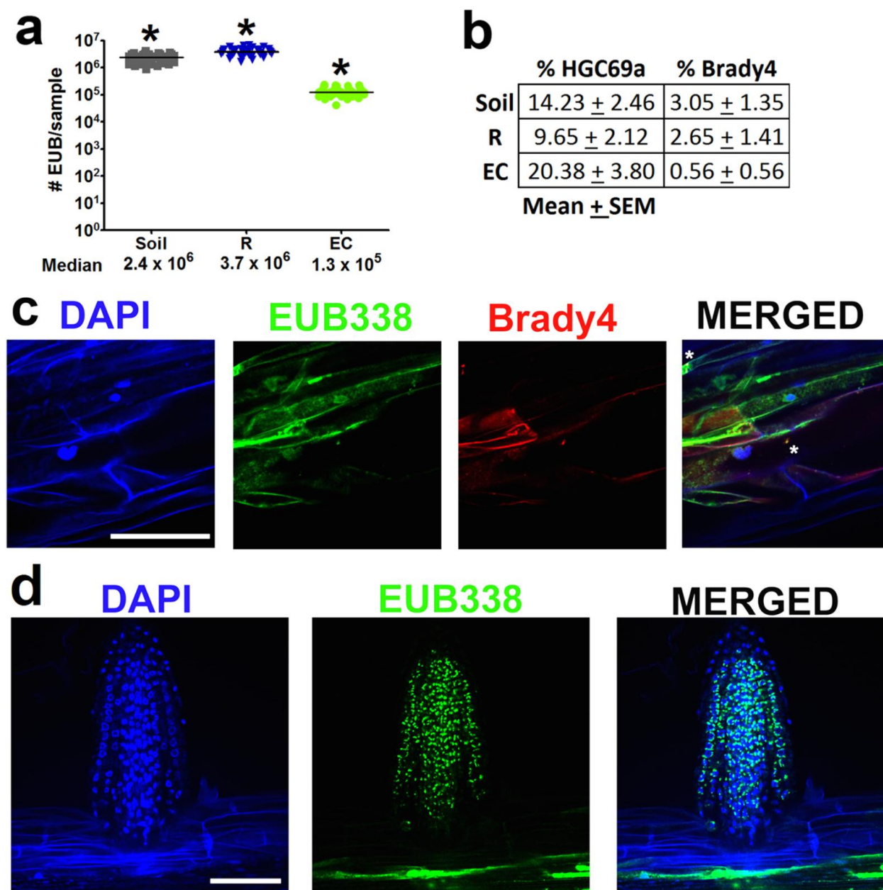
Supplementary Figure S12: Quantification of microbes in the three sample fractions using CARD-FISH. Four sets of Col-0 roots were pooled, processed, diluted, and put onto filters. (a) CARD-FISH using the EUB338, eubacterial probe, was applied and counterstained with DAPI. The number of EUB positive signals co-localizing with a DAPI signal was counted and the number of EUB positive signals per sample was calculated. This is an estimate for the number of bacteria present in each of our samples that DNA was extracted from with bulk soil ( n=40 ), rhizosphere ( n=39 ), and endophytic compartment ( n=40 ). * indicates statistical significance at p < 1 \times 10^{-16} (ANOVA with post-hoc TukeyHSD) between each of the sample groups (b) Using double CARD-FISH on filters made from equal concentration of the 3 sample fractions, we determined the % of DAPI positive eubacteria that are also co-localize with either the HGC69a (Actinobacteria) or Brady4 (Bradyrhizobiaceae) probes on filters made from bulk soil ( n=10 ), rhizosphere ( n=10 ), and endophytic compartment ( n=10 ) samples. Actinobacteria was in higher abundance in EC samples and Bradyrhizobiaceae was in lower abundance in EC samples compared to soil and R samples as expected from our pyrotag sequencing data. (c) Double CARD-FISH was applied using the EUB338, eubacterial probe (green) and the Brady4, Bradyrhizobiaceae probe (red), counterstained with DAPI (the asterisks indicate signals that are positive in all 3 channels). (d) Newly forming lateral roots and root tips were found commonly to be heavily colonized. Scale bars represent 50 microns.
