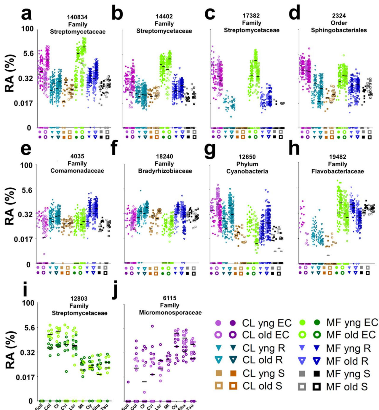
Supplementary Figure 11: Dot plots of notable OTUs. Relative abundance for each OTU (number at top of each panel; keyed to Supplementary Table ST3) from the frequency-normalized table was \log_2 transformed and the abundance for each sample (y-axis) plotted as an individual symbol. The y-axis is labeled with the actual (untransformed) relative abundance values. In a-h , each position on the x-axis is labeled with a symbol to represent the sample group (legend, lower right), and samples from that group are plotted column-wise directly above. Biological replicates are shown in the same column with different hues. The median of each biological replicate is shown with a horizontal black bar; some may not be visible because they are at 0. In i and j , sample color is according to the legend, and each position on the x-axis is labeled by Arabidopsis accession, with samples from that accession plotted above each label. Each OTU in the figure has model predictions in several categories (Supplemental table ST3).
