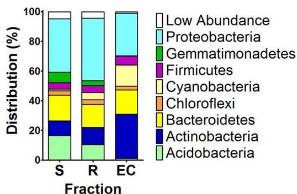
Supplementary Figure S15: Phyla in each sample fraction by soil type. Histogram displaying the distribution of the phyla present in the 778 measurable OTUs in soil (S), rhizosphere (R) and endophytic compartments (EC) with each soil type, MF and CL, considered independently. Rarefaction-normalized on top; frequency-normalized on bottom. Accompanying statistics on the distributions are in Supplementary Table ST5.
