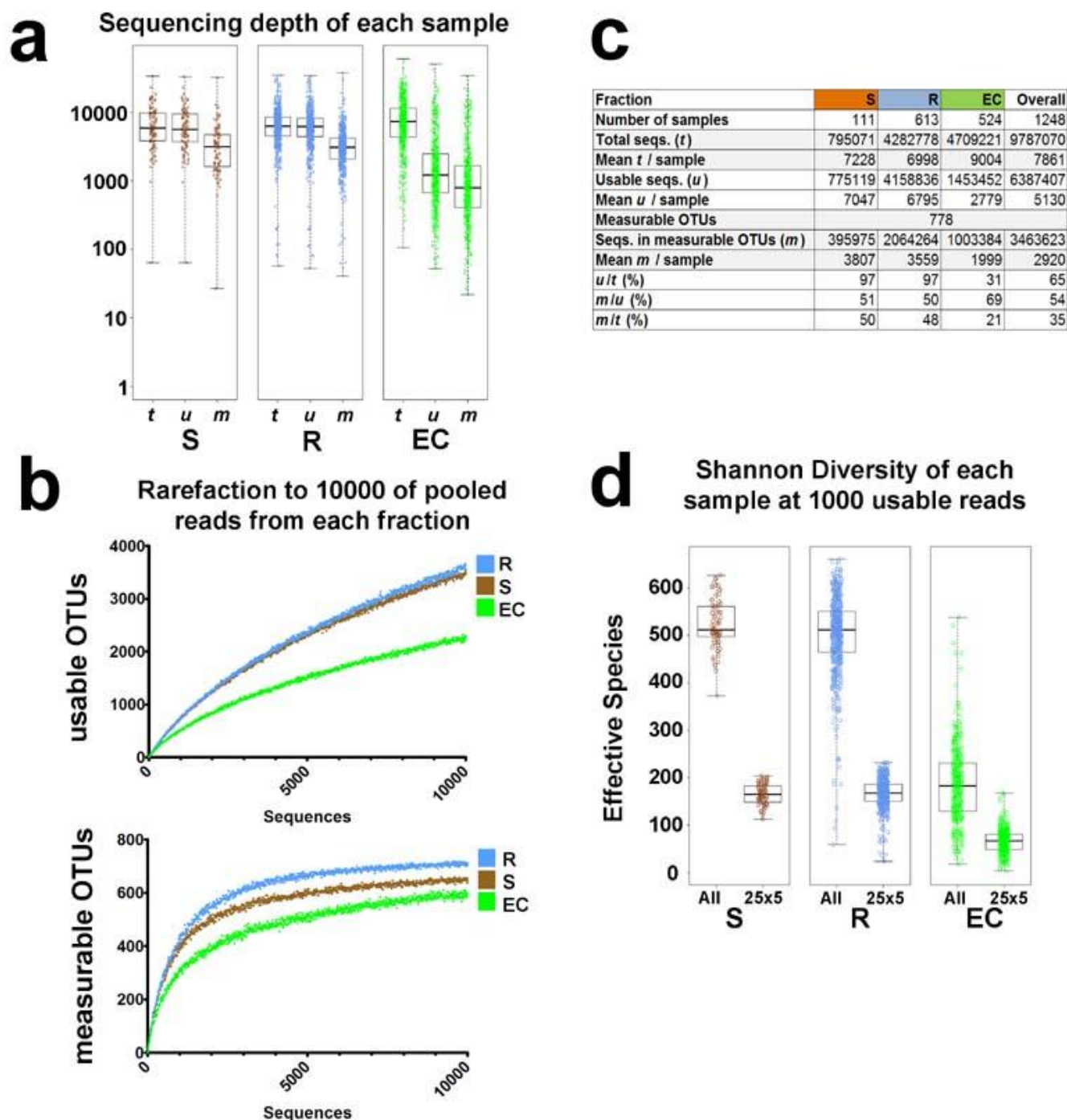
Supplementary Figure S4: Sequencing statistics and quality. a ) Sequencing depth per sample in reads for the three sample fractions S, R, and EC. Each dot represents a single plant or soil sample. Within each fraction, the total ( t ), usable ( u ), and measurable ( m ) read counts are shown for all samples. The box plots contain the 1st and 3rd quartiles, split by the median; whiskers extend to include the farthest outliers. b ) Rarefaction curves to 10,000 sequences for cumulative reads from S, R, and EC fractions considering all usable OTUs (top) and only measurable OTUs (bottom). c ) Table, split by sample fraction, summarizing: cumulative numbers of total high quality reads, 'usable' (non-plant & non-chimera) reads, number of OTUs after the technical reproducibility '25x5' threshold is applied, 'measurable' reads (reads contained in OTUs that pass the 25x5 threshold). d ) Shannon diversity of individual samples from each fraction, calculated from the rarefaction-normalized table, before (left) and after (right) applying the 25x5 measurable OTU threshold.
