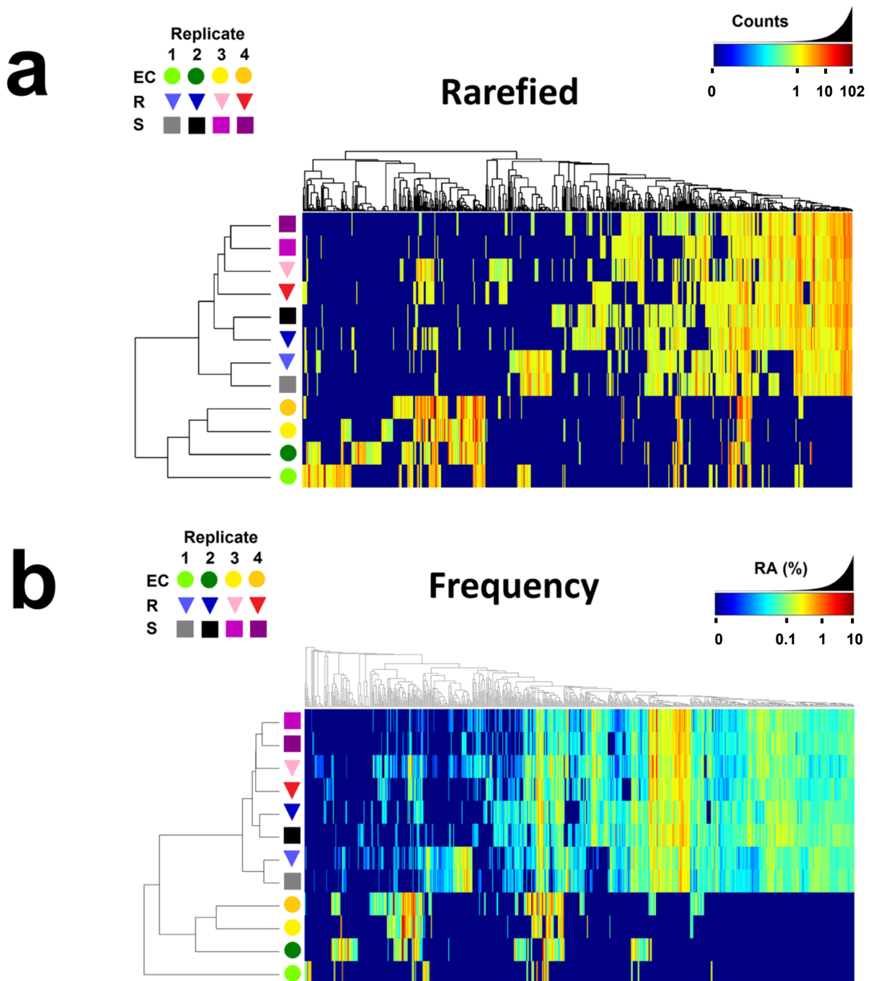
Supplementary Figure S6: OTUs identified from four independent biological replicates are reproducible. Heat map displaying the reproducibility between four independent replicates at the yng developmental stage of bulk soil (squares), Col-0 R samples (triangles), and Col-0 EC samples (circles). Each symbol represents the median of six or more samples. All data were \log_2 transformed for visualization, but for ease of interpretation the quantities shown in the color key represent the original (untransformed) counts (in panel a) and frequencies (in panel b) for each color. Although all 778 measurable OTUs were included, some OTUs had a median of 0 in all Col-0 and soil groups shown and were removed from the display.
