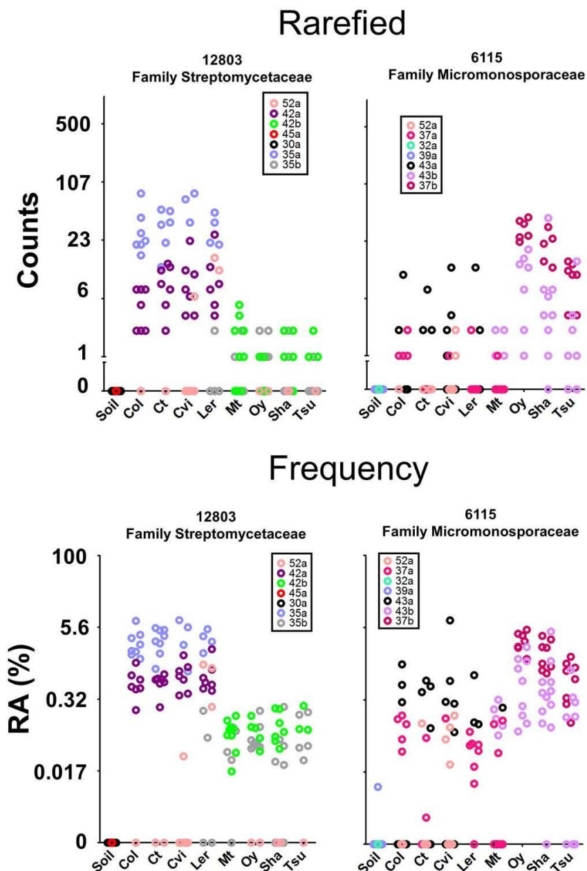
Supplementary Figure S14: Genotype-variable OTUs colored by sequence plate. Displays the data from Fig. 3i (MF old EC, left) and Fig. 3j (CL old EC right), colored by sequence plate (instead of biological replicate as in Figure 3) according to the legend within each plot. The top panel is based on rarefied data, as in Figure 3, and the bottom panel is based on the relative abundance, as in Supplementary Figure S11. (Note: 'a' and 'b' in our plate naming scheme do not represent different regions of the same plate. All 454 regions were modeled independently in the Full GLMM).
