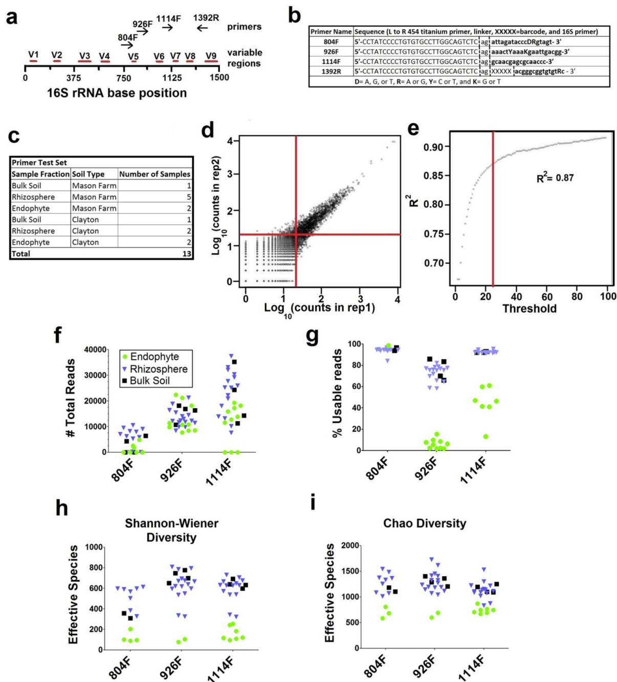
Supplementary Figure S2: Primer test and technical reproducibility. a ) Position on the 16S gene of each of the primers tested. b ) Sequence of each primer used. c ) Composition of the 13 samples tested. d ) Log 10 transformation of raw reads per OTU for one independent replicate (x-axis) vs. the other (y-axis), where both replicates were PCR-amplified and sequenced from the same sample (axes labels are transformed and cover a range of 0-10,000 reads). The intersection of the red lines shows where an OTU with 25 reads in both replicates would lie. e ) Progressive drop-out analysis displaying the R^2 correlation of the data in d as OTUs with low read numbers are discarded. When only OTUs with \geq 25 reads are considered (red line) the R^2 is acceptable at 0.87, a balance between reproducibility and data loss for low-abundance OTUs. In f-i , green circles are EC samples, blue triangles are R samples, and black squares are bulk soil samples. f ) Total reads obtained from amplicons made with 804F, 926F, or 1114F paired with bar-coded 1392R. g ) Percent of the 'usable' reads from f which are not identified as plant or chimeric OTUs. h ) Shannon-Wiener species diversity of 1000 usable reads (for each sample with \geq 1000 reads). i ) Chao1 diversity of 1000 usable reads from each sample (for each sample with \geq 1000 ).
