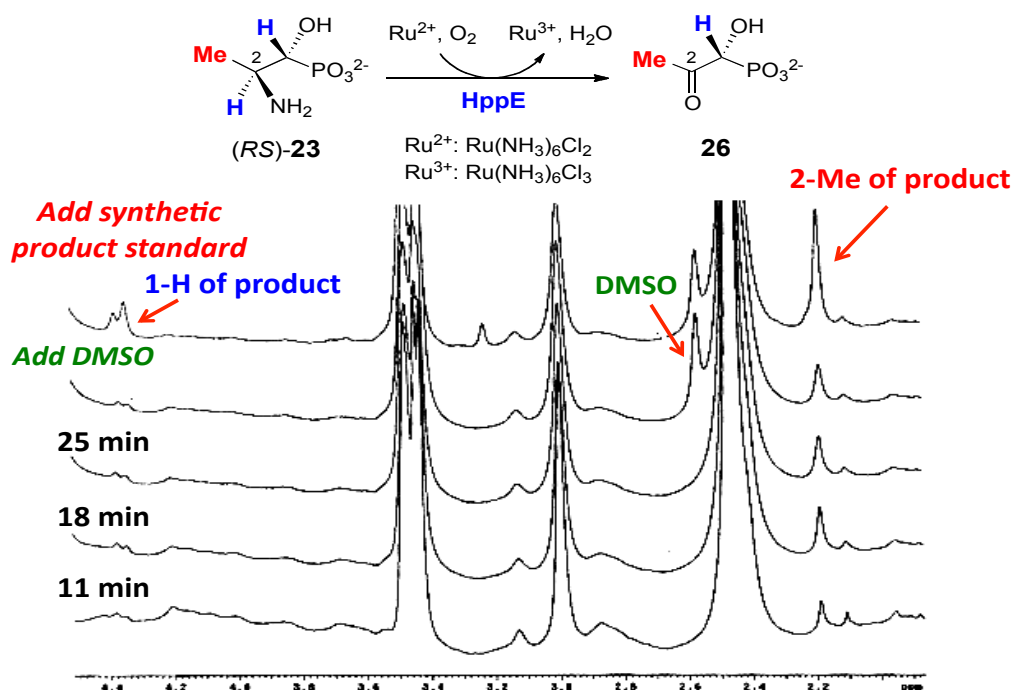
Figure S4: (B) 1 H NMR time-course for the HppE-catalyzed conversion of (RS)-23 to 26 using Ru(NH 3 ) 6 Cl 2 as reducing agent. Additional DMSO- d 6 was introduced as an internal standard prior to the addition of synthetic 26.
