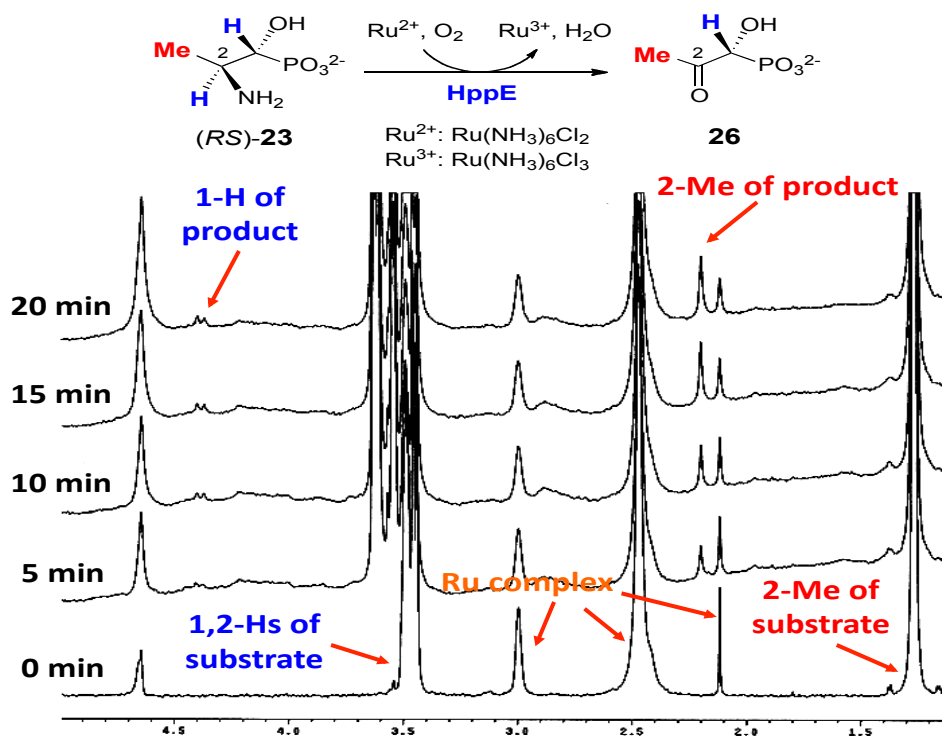
Figure S4: (A) 1 H NMR time-course for the HppE-catalyzed conversion of (RS)-23 to 26 using Ru(NH 3 ) 6 Cl 2 as reducing agent.
