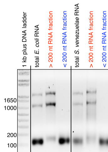
Supplementary Figure 10. Silica column-based size fractionation of cellular RNA. Total E. coli or S. venezuelae RNA was separated into fraction I (RNAs of length > \sim 200 nucleotides) and fraction II (RNAs of length < \sim 200 nucleotides) using a Qiagen RNeasy silica column. The starting total RNA and each fraction (1 \mu\text{g} per lane) was analyzed by 1% TAE-agarose gel electrophoresis and stained with ethidium bromide.
