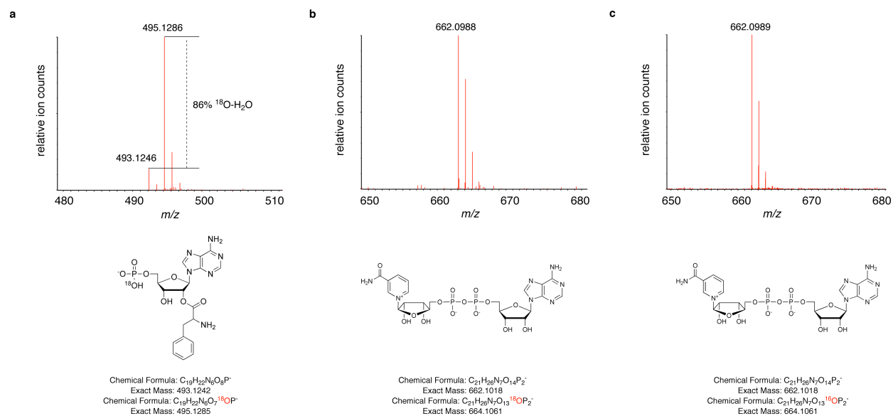
Supplementary Figure 7. In the presence of ^{18}\text{O} water, all nuclease P1 digestion products other than the nucleotides at the 5' ends of substrates will exhibit a +2 Da mass shift compared with the products arising from digestion in ^{16}\text{O} water. (a) Phenylalanyl AMP, a known small molecule-RNA conjugate that exists at the 3' end of tRNA, exhibits the expected +2 Da shift. (b) No mass shift is observed in the case of NAD, indicating that this modification is located at the 5' terminus of the RNA(s). (c) Authentic NAD has a similar isotope pattern as NAD from nuclease P1 digestion of total RNA.
