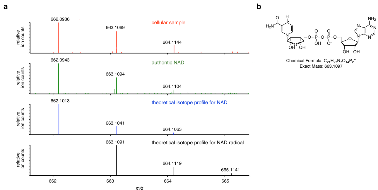
Supplementary Figure 13. NAD radical may contribute to the [M-H]^- m/z 663.1069 signal in the authentic and cellular NAD spectra. (a) Mass spectra of cellular and authentic NAD, and the theoretical isotope profiles for NAD and NAD radical. (b) Structure of NAD radical.
