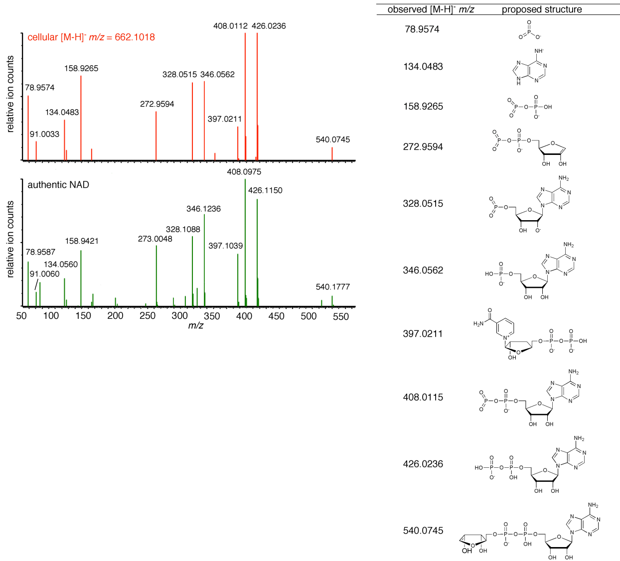
Supplementary Figure 5. MS/MS fragmentation of E. coli cellular species [M-H] - m/z = 662.1018 and comparison with authentic NAD confirms the assignment of the [M-H] - m/z = 662.1018 as NAD. A table of plausible fragment ion structures is provided.
