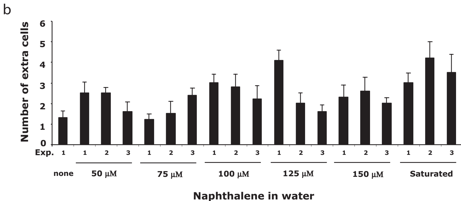
Supplementary Figure 1. Naphthalene in air or water has inconsistent dosage effects in suppressing apoptosis. ced-3(n2438) animals were exposed to naphthalene dissolved in air (a) or water (b) at the indicated concentrations and the numbers of extra cells in the anterior pharynx were scored. Three independent experiments (Exp.) were carried out at each concentration point. At 0.6 g/L iter air, naphthalene can be lethal to animals. There were not enough surviving animals to score in two experiments at this concentration. The y-axis represents the average number of extra cells scored in the anterior pharynx of ced-3(n2438) mutants. Error bars are standard errors of the mean. Ten animals were scored in each experiment.
