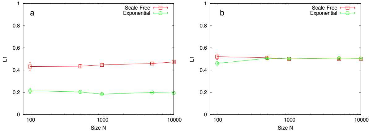
Supplementary Figure S5: (a) The L_1 distance between pagerank scores of the original and perturbed networks as a function of system size N . The red squares correspond to a scale-free network and the green circles correspond to an exponential network, both with average degree \langle k \rangle = 1.5 . The points are averaged over N realizations for each N . There is no evident scaling with N in either network. (b) The L_1 distance between the ranked lists in the same networks, where the ranks have been converted to a probability distribution using equation (S60). There is no scaling with size here as well, in addition the two networks are virtually indistinguishable.
