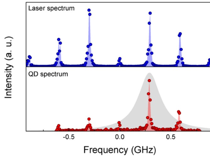
Supplementary Figure S3| Spectra for laser pulses and resulting spectra for coherent QD scattering. For the two-photon interference coherent laser pulses are created by applying electrical pulses down to 100 ps duration from an arbitrary pulse pattern generator with 10-GHz bandwidth to the EOM. An additional DC offset with feedback controls the slow drifts of the EOM operation settings. Top panel: Measured spectrum for laser pulses of \sim 400 ps width and a repetition rate of 300 MHz. The spacing of spectral components corresponds to the pulse repetition rate. Bottom panel: The resulting QD emission spectrum for 260-MHz detuning from the central laser frequency. Since the pulse width is significantly shorter than the QD excitonic lifetime, the amplitude of spectral components is strongly modified by the QD bandwidth.
