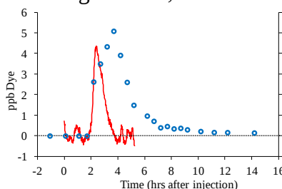
Figure S2.4b. Traces from L7 in 2009. Symbols follow Fig. S2.4a.
