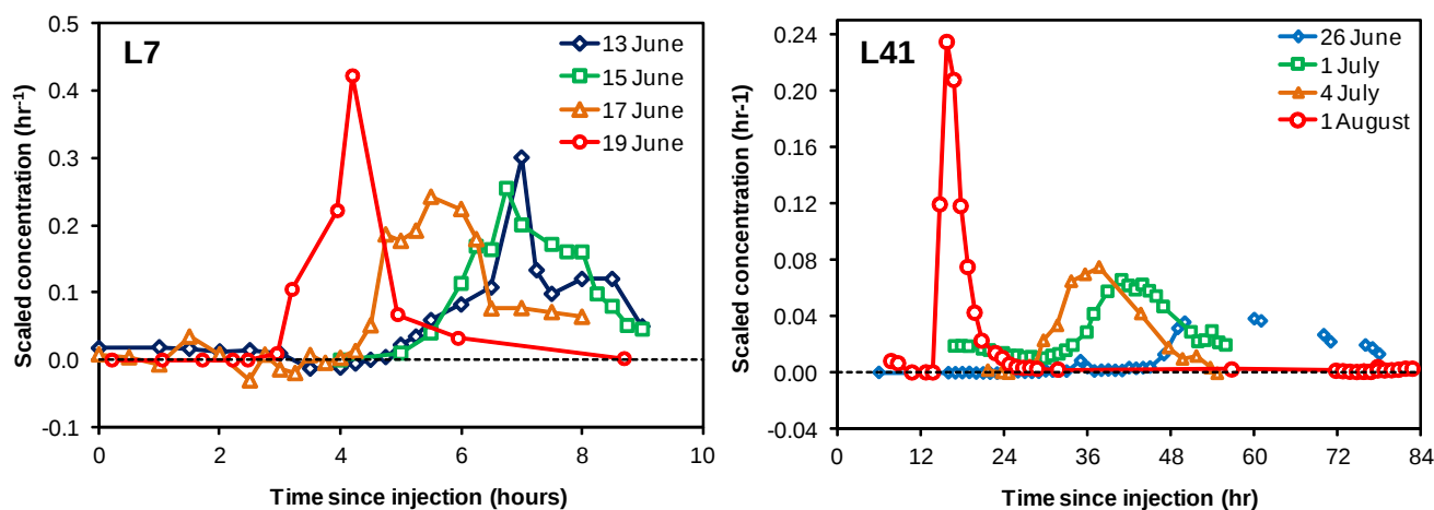
Figure S2.5. \text{SF}_6 traces from L7 and L41 in 2011. Tracer returns have been scaled to have unit area.
