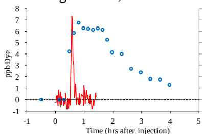
Figure S2.4a. Dye (red lines) and SF_6 (blue circles) traces from L1 in 2009. Dye concentrations were recorded at 1 minute intervals; SF_6 concentrations were measured in discrete samples represented by individual data points.
