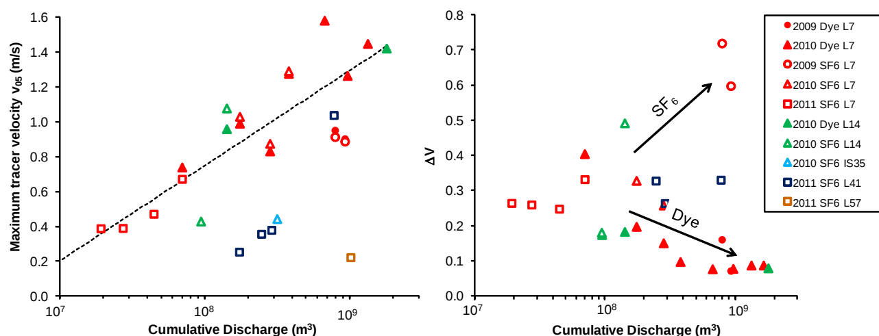
Figure S2.8: Evolution of tracer velocity and dispersion with time. While maximum velocities for \text{SF}_6 are shown to be representative of the water flow (see text), the dispersion values can be strongly influenced by degassing and are not reliable estimates of the true values: instead they may reflect drainage system pressurisation. Time is measured by cumulative discharge to allow comparison between years with different timing and intensity of surface melt. The dashed line in the left panel is the regression curve for Site L7, which has the form v_{05} = A \ln(\Sigma Q) + B where v_{05} is the maximum velocity (here corresponding to the time at which 5% of the recovered tracer had emerged) and A , B are regression parameters ( A = 0.235 \text{ m s}^{-1} , B = -3.59 \text{ m s}^{-1} ; r^2 = 0.63 , p < 0.01 ). See Section S2 for definitions of velocity and dispersion.
