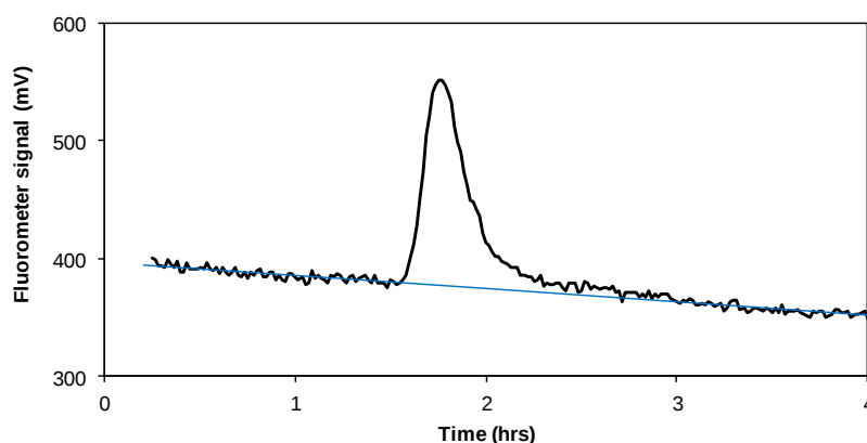
Fig. S2.1: Example dye trace from L7, 21 June 2010, showing the measured fluorometer signal V_m (black line) and inferred background V_b (blue line).
