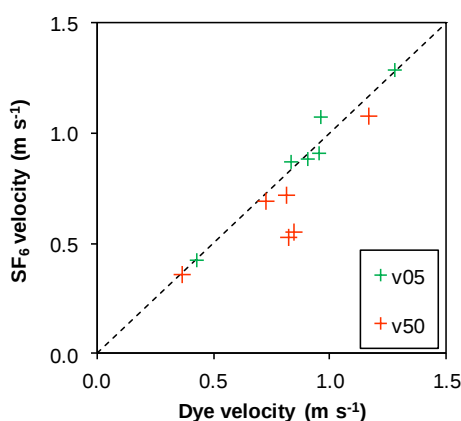
Figure S2.7. Comparison of tracer velocities in dual traces from moulins L7 and L14. v_{05} and v_{50} represent the maximum and mean tracer velocities, respectively. Traces close to the dashed line yielded similar velocities for dye and \text{SF}_6 .
