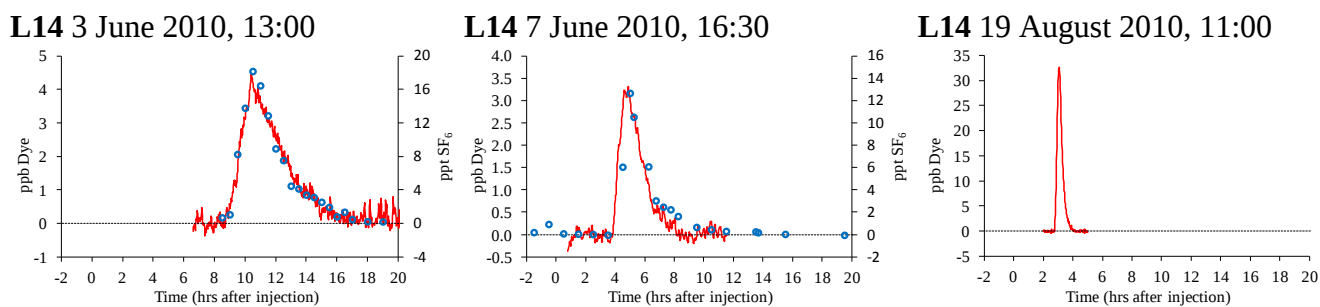
Figure S2.4e. Traces from L15 in 2010. Symbols follow Fig. S2.4a.
