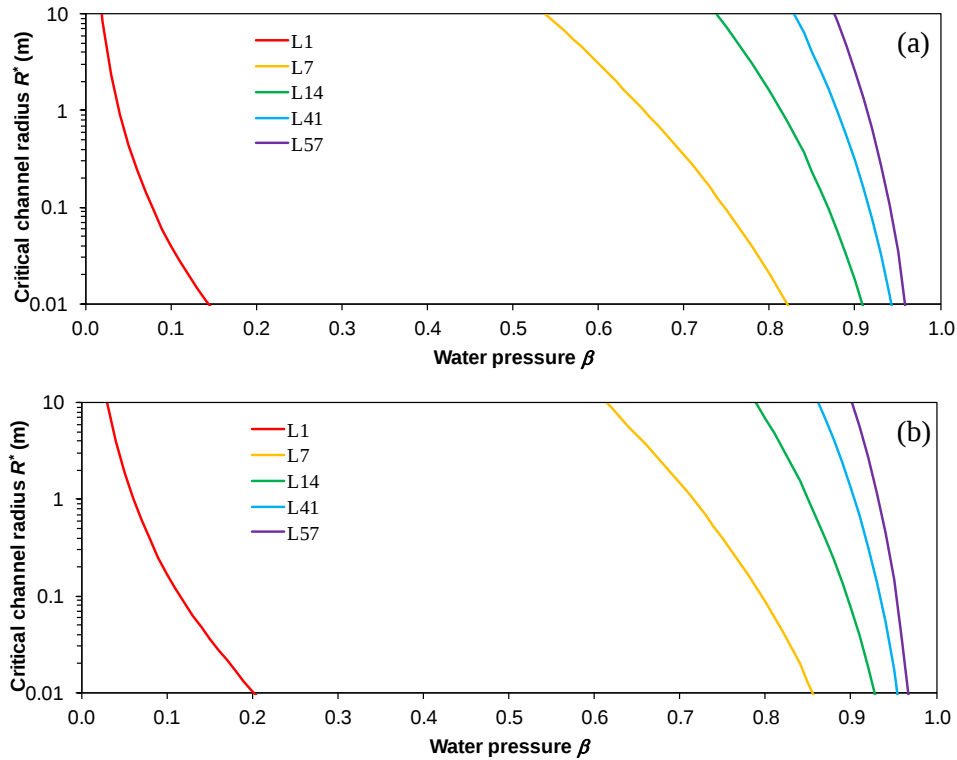
Fig. S4.1: Variation in critical radius R^* with channel pressurisation \beta , calculated using estimated values of H and dH/ds for locations at increasing distances from the terminus. Part (a): semicircular channels with ice walls and floor, using parameters suggested by Schoof 7 ; part (b) is the same as (a) but with a sediment-based channel.
