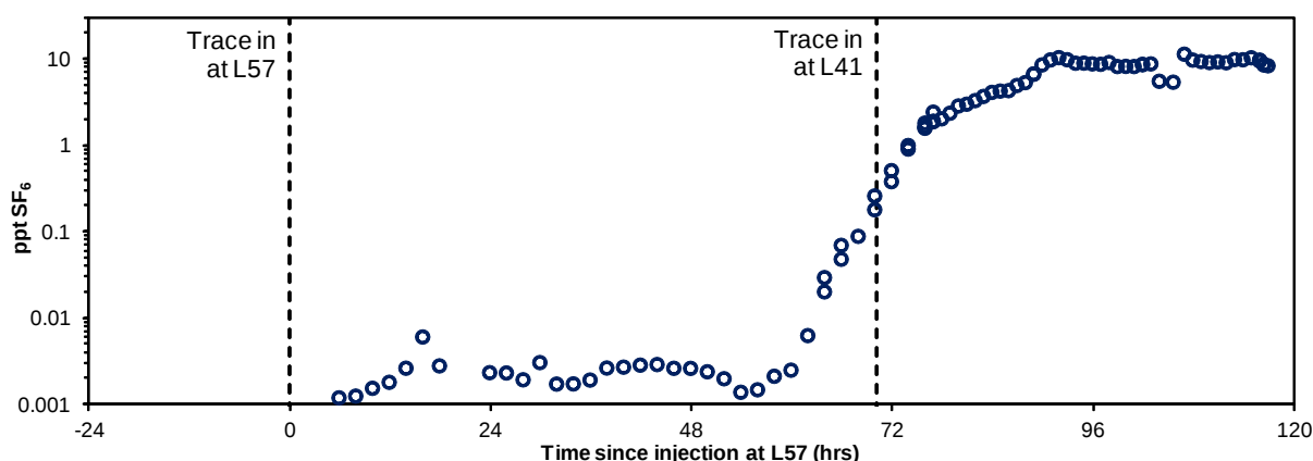
Figure S2.6: \text{SF}_6 returns from the last two traces in 2011, at L57 (12 August, 20:30) and L41 (15 August, 18:30). Water samples for both traces were collected in bottles for analysis in the U.K., and the later than expected arrival of the L57 trace unfortunately interfered with the subsequent L41 trace. However, the arrival of the L57 trace prior to injection of the L41 trace enables an estimate of the maximum velocity of the L57 trace ( 0.22 \text{ m s}^{-1} ). Given the rapid passage of previous L41 traces in < 24 \text{ hr} (see Fig. S2.4) it is likely that most of the sustained, high \text{SF}_6 concentrations are due to the L57 trace; however, this cannot be confirmed. Noting the log scale, we find that the \text{SF}_6 analysis method employed in this study can yield data with apparently low noise levels over 4 orders of magnitude.
