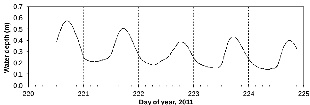
Figure S3.4: Water depth in the stream feeding Moulin L57 during days 220 – 224 (8 – 12 August) 2011. The single \text{SF}_6 trace of L57 was injected at the end of this period (20:30 hrs, 12 August).
