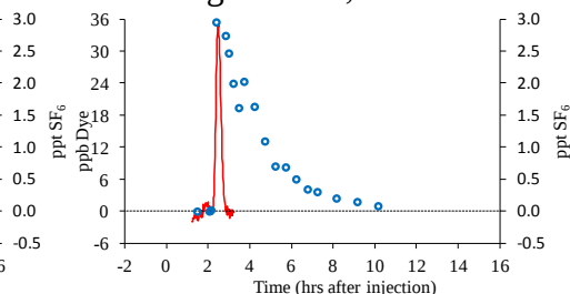
Figure S2.4b. Traces from L7 in 2009. Symbols follow Fig. S2.4a.
