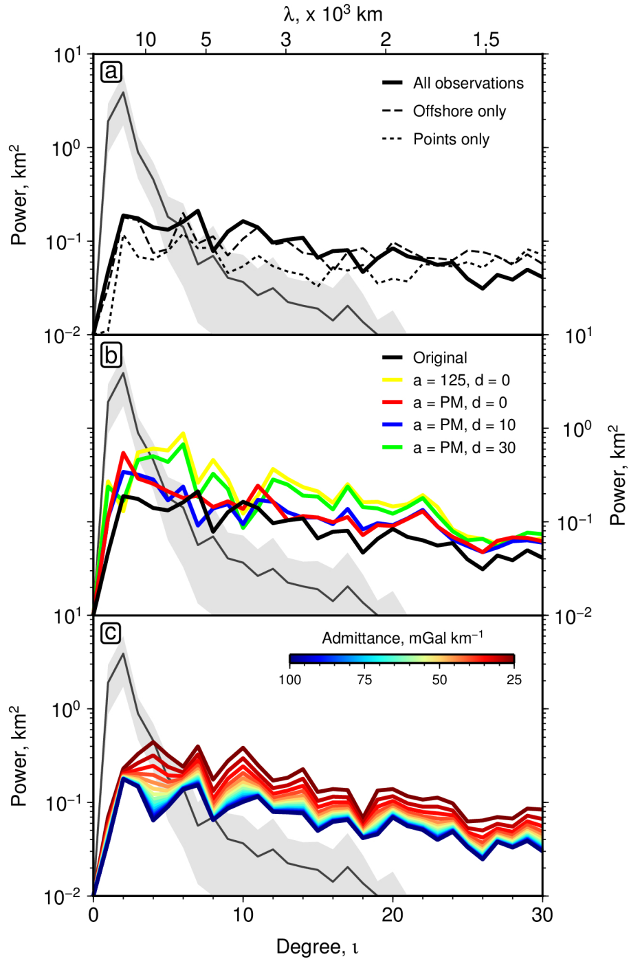
Figure S3: Continental Tests. (a) Power spectra for decimated datasets. Solid line = power spectrum for complete observational database (Figure 1b of main text); dashed line = power spectrum for oceanic spot measurements and ship-track data alone (i.e. no continental input); dotted line = power spectrum for oceanic spot measurements alone. Grey line/band = mean/standard deviation of 5 predictive models of dynamic topography [4, 5, 6, 7, 8]. (b) Power spectra for alternative continental observations. Black line = power spectrum using continental dynamic topography calculated from long-wavelength free-air gravity anomalies; yellow line = power spectrum using continental dynamic topography calculated from CRUST 1.0 database assuming constant lithospheric thickness of 125 km [9]; red line = as before but using variable lithospheric thickness [10]; blue line = as before where lithosphere thicker than 175 km is depleted by 10 \text{ kg m}^{-3} ; green line = as before with depletion of 30 \text{ kg m}^{-3} . (c) Coloured lines = power spectra using continental dynamic topography calculated from long-wavelength free-air gravity anomalies using admittance values ranging from 25–100 \text{mGal km}^{-1} .
