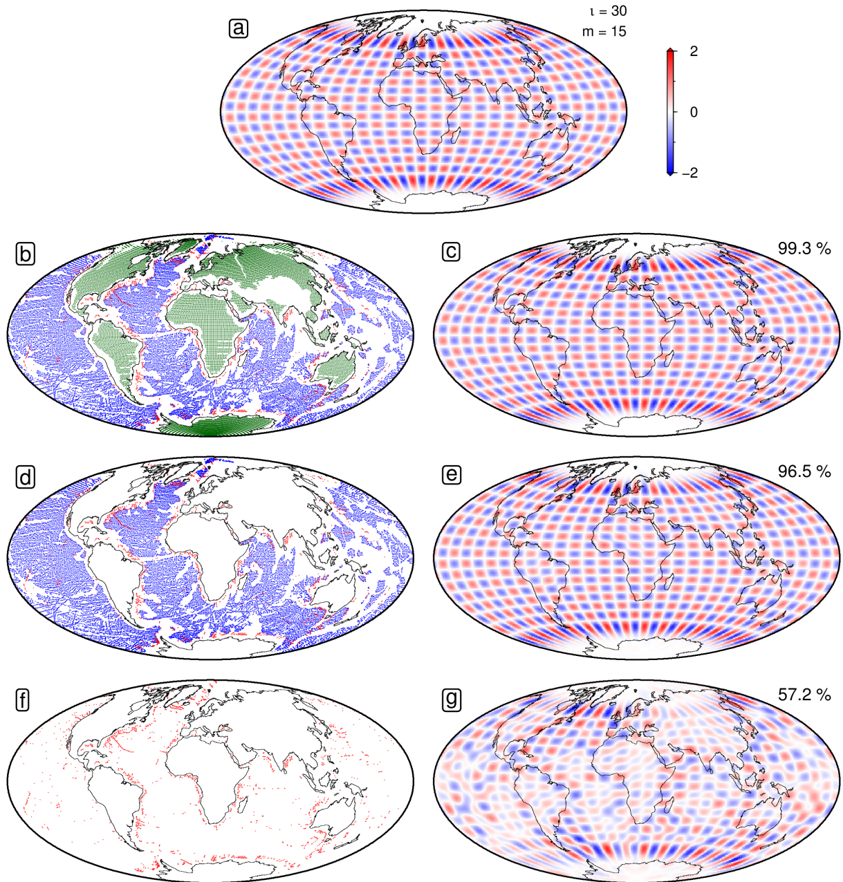
Figure S7: Synthetic checkerboard test. (a) Input spherical harmonic function with l = 30 and m = 15 . (b) Locations of all oceanic and continental data points used to sub-sample input model. (c) Resulting spherical harmonic fit with recovery of input coefficients. (d) All measurements from oceanic realm alone. (e) Recovery obtained using (d). (f) Only spot measurements from oceanic realm (symbols from Figure 1b of main text). (g) Recovery obtained using (f).
