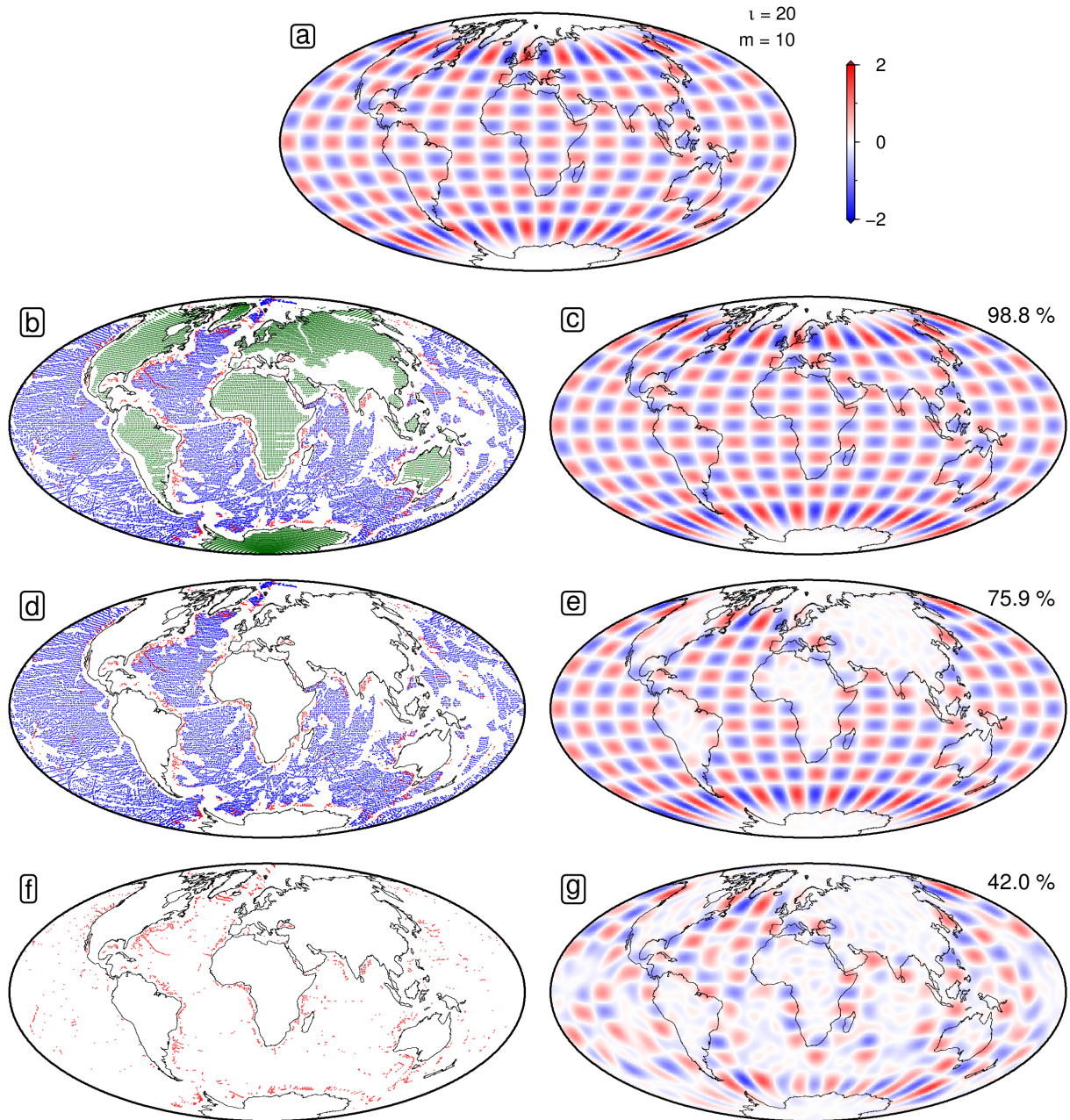
Figure S6: Synthetic checkerboard test. (a) Input spherical harmonic function with l = 20 and m = 10 . (b) Locations of all oceanic and continental data points used to sub-sample input model. (c) Resulting spherical harmonic fit with recovery of input coefficients. (d) All measurements from oceanic realm alone. (e) Recovery obtained using (d). (f) Only spot measurements from oceanic realm (symbols from Figure 1b of main text). (g) Recovery obtained using (f).
