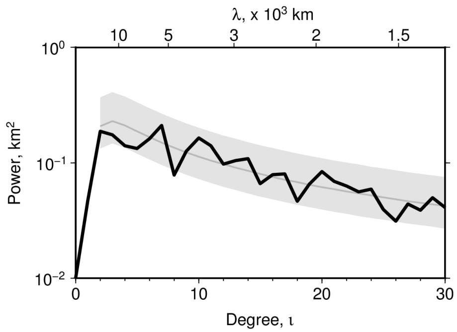
Figure S10: Kaula's rule. Solid line = power spectrum of observational database (Figure 5b in main text); grey line/band = power spectrum calculated using Equation 4 for Z = 12 \pm 3 \text{ mGal km}^{-1} .
