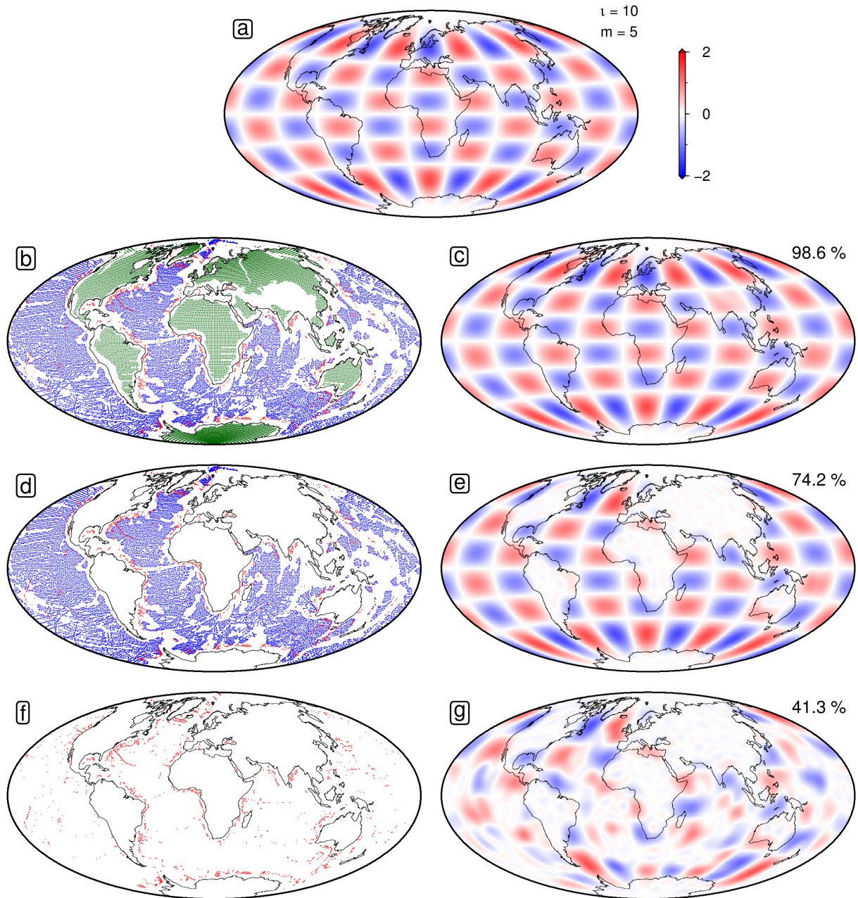
Figure S5: Synthetic checkerboard test. (a) Input spherical harmonic function with l = 10 and m = 5 . (b) Locations of all oceanic and continental data points used to sub-sample input model. (c) Resulting spherical harmonic fit with recovery of input coefficients. (d) All measurements from oceanic realm alone. (e) Recovery obtained using (d). (f) Only spot measurements from oceanic realm (symbols from Figure 1b of main text). (g) Recovery obtained using (f).
