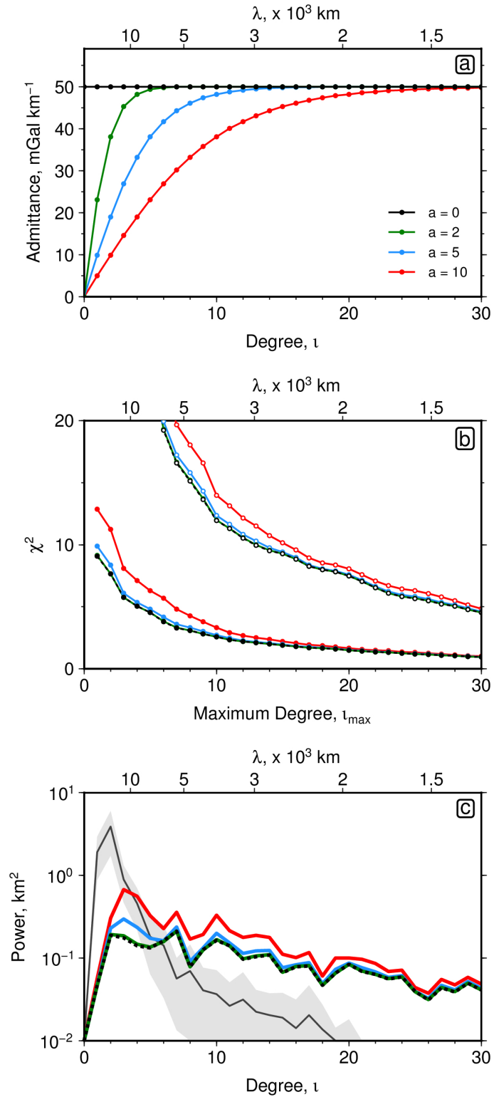
Figure S4: Wavelength-dependent admittance tests. (a) Admittance curves used to calculate four different sets of gravity-derived continental dynamic topographic databases. (b) Residual misfit, \chi^2 , for these four sets. Solid circles = oceanic and continental databases; open circles = spot measurements from oceanic realm alone. (c) Power spectra. Thick lines = power spectra calculated from four different sets of databases; thin line with grey bounds = mean and standard deviation of power spectra for five predictive models.
