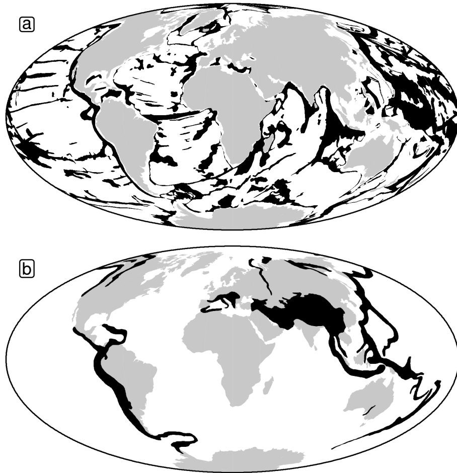
Figure S1: Exclusion polygons. (a) Distribution of exclusion polygons within oceanic realm that were used to excise regions of anomalously thick or thin oceanic crust from residual topographic measurements derived from ship-track database. (b) Distribution of exclusion polygons that were used to excise orogenic and flexural zones from maps of long-wavelength gravity anomalies.
