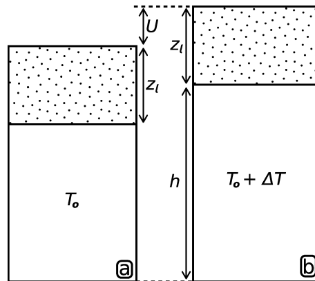
Figure S11: Sub-plate asthenospheric isostatic balance. (a) Standard case, where T_o = average temperature of the asthenosphere. Dotted pattern = crust and lithospheric mantle. (b) Air-loaded uplift, U , generated from a sub-plate channel of thickness h , and average temperature T_o + \Delta T .
