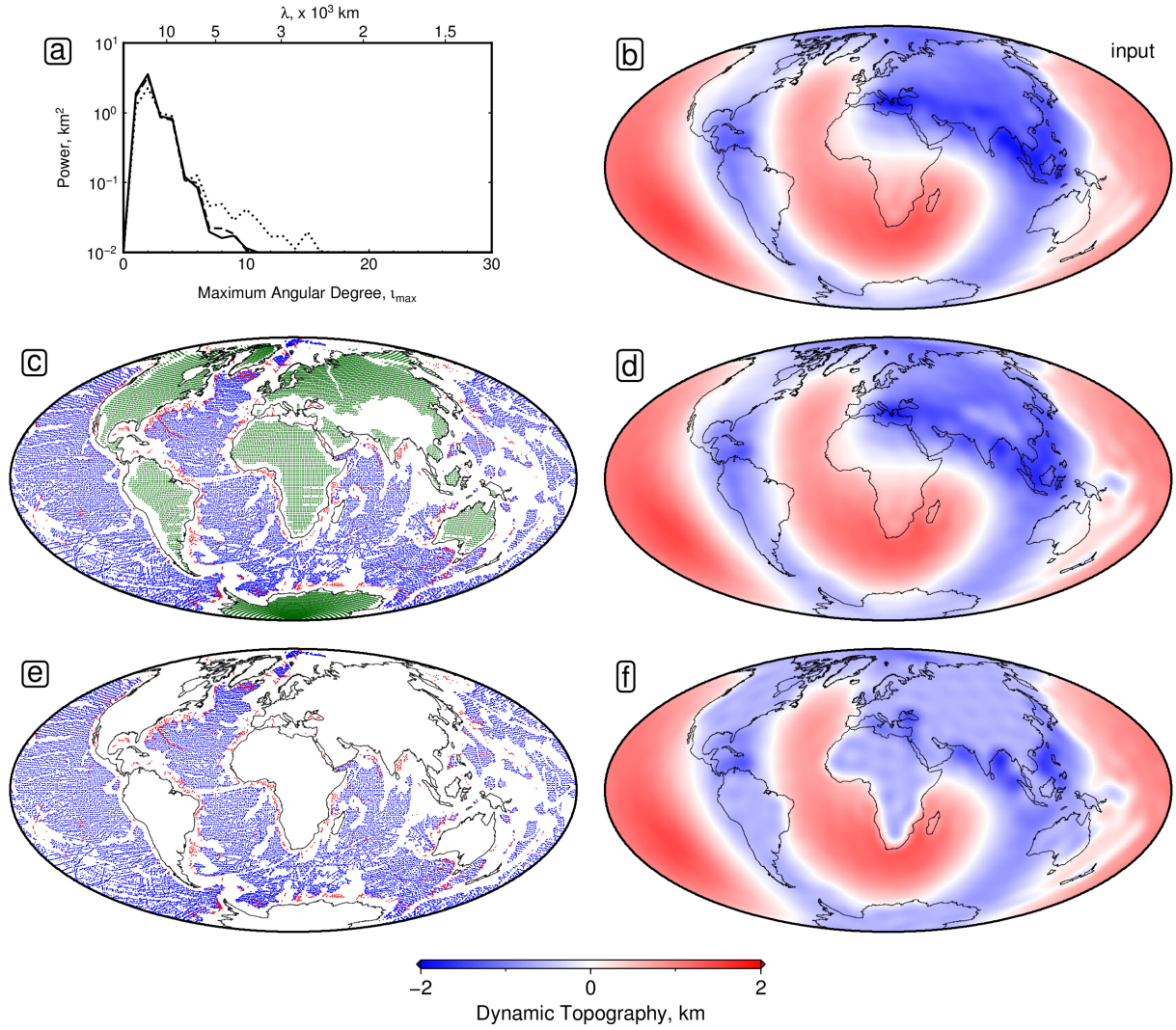
Figure S8: Benchmark test. (a) Solid line = power of predicted dynamic topographic model shown in (b); dashed line = recovered power using data distribution shown in (c); dotted line = recovered power using data distribution shown in (e). (b) Global dynamic topography prediction from Flament et al. [8]. (c) Oceanic and continental data points used to sub-sample input model. (d) Recovered model obtained using (c). (e) Oceanic data points. (f) Recovered model obtained using (e).
