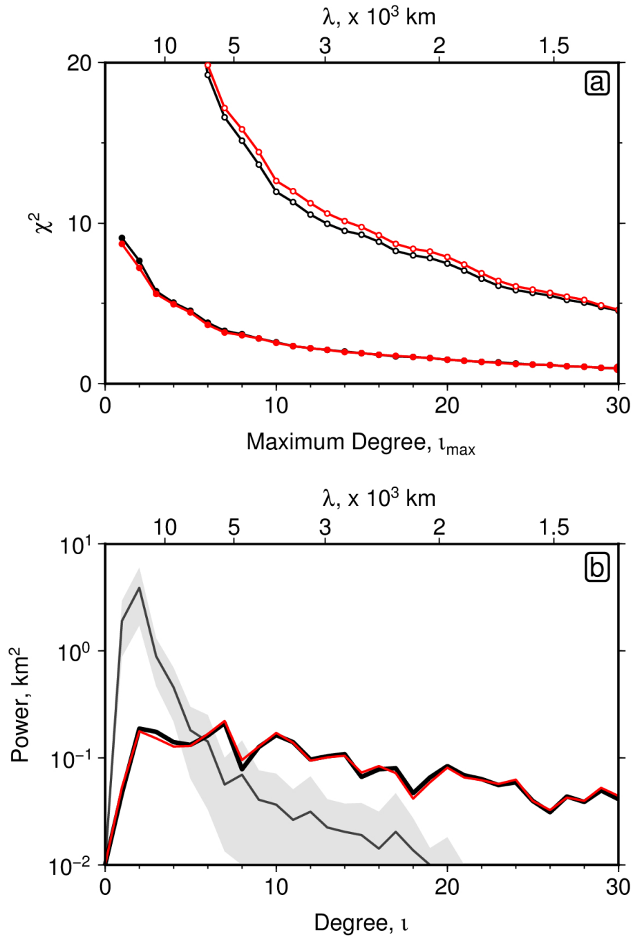
Figure S9: Effect of weighting the data by latitude. (a) Residual misfit, \chi^2 , plotted as function of maximum degree; solid circles = \chi^2 values from fitting combined offshore/onshore global database of dynamic topographic observations; open circles = \chi^2 values from fitting spot measurements from oceanic realm alone; black = original, non-latitude weighted data; red = including a latitude weighting. (b) Power spectra of observed dynamic topography using non-latitude (black) and latitude-weighted (red) misfit functions. Grey line/bounds = mean/standard deviation of the five predictive models.
