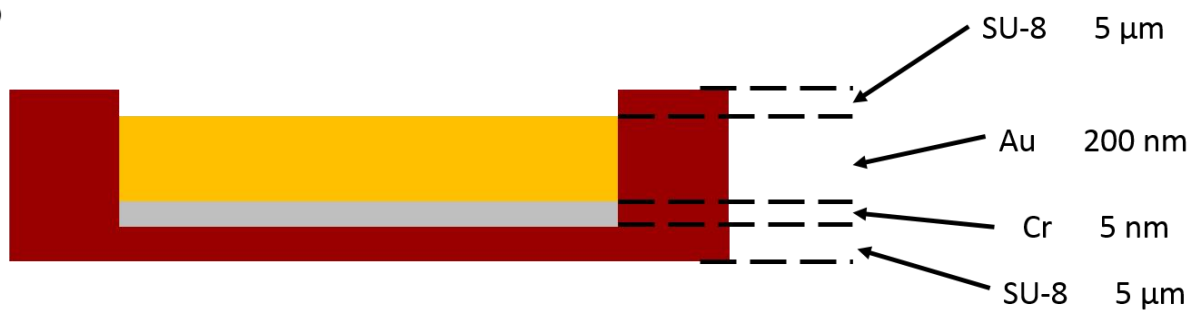
Figure S2 | Electrode fabrication and design. Electrodes were deposited on top of a 5 \mu\text{m} SU-8 bottom layer and passivated with a 5 \mu\text{m} SU-8 top layer. Pads were left exposed in order to contact cells. Scale bar: 2 \mu\text{m} .
