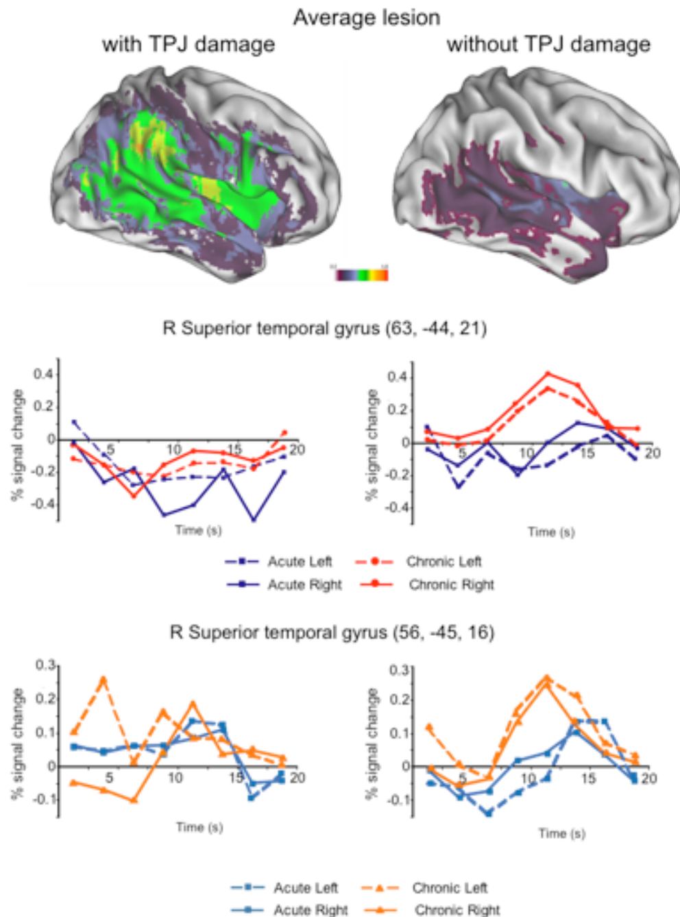
Figure 3. Reactivation of TPJ as function of anatomical damage. Top: Average anatomical damage in patients with or without TPJ damage. Note larger lesion volume in TPJ group. Middle: BOLD signal in right STG (63,-44,21, ROI selected from voxel-wise ANOVA Stage x Time, Table 2) recovers only in patients without TPJ damage. Bottom: BOLD signal in right STG (56,-45,16 ROI selected from voxel-wise ANOVA Stage x Validity x Time, table 3) shows that response for invalid targets is weaker and delayed at the acute stage, but only in patients without TPJ damage.
