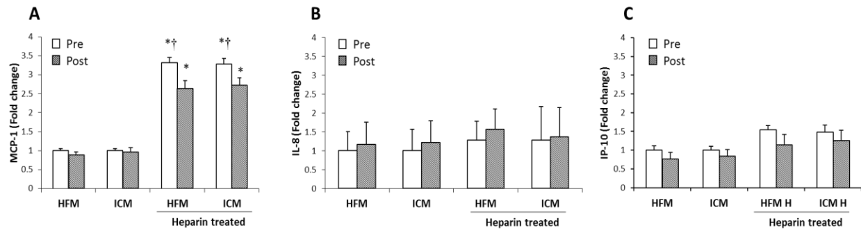
Figure S2. Effects of HFM and ICM on plasma and RBC-bound chemokine levels. Plasma MCP-1, IL-8, and IP-10 were assayed following consumption of either HFM or ICM. Heparin was used to liberate chemokines bound to DARC on RBCs. Pre refers to pre meal, and post refers to post meal. *Significant vs no heparin treatment, †Significant vs post meal.
