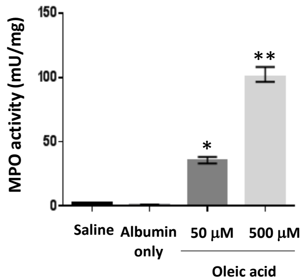
Figure S3. Effects of oleic acid on MPO release from monocytic cells. Treatment of albumin-conjugated oleic acid released active MPO from THP-1 cells in a dose-dependent manner. *Significant vs Albumin only (* p <0.05, ** p <0.001, n =3).
