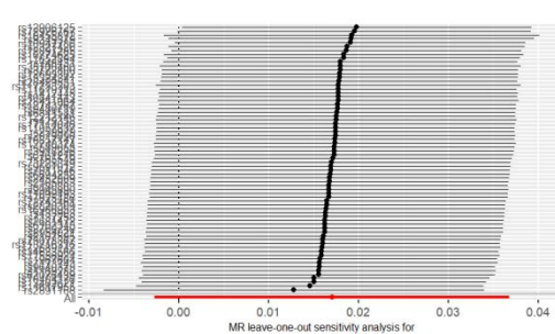
MI on MDD(PGC)
