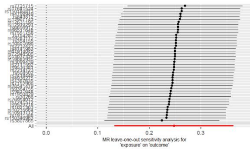
MDD(PGC) on Hypertension
