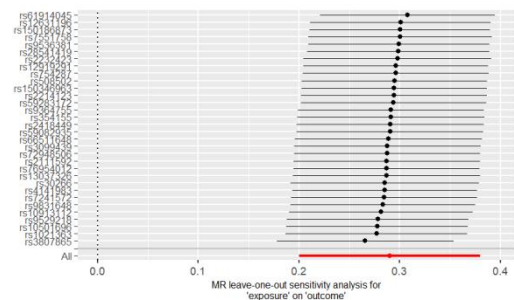
MDD(PGC) on CAD
