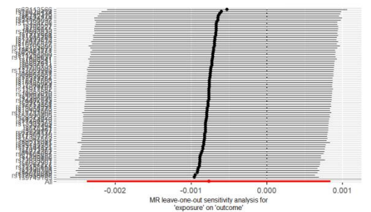
Anxiety(PGC) on Hypertension
