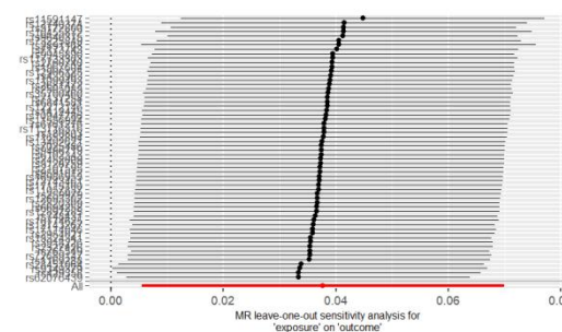
MI on Anxiety(PGC)
