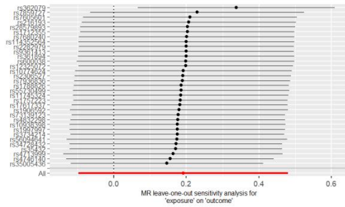
Hypertension on MDD(PGC)
