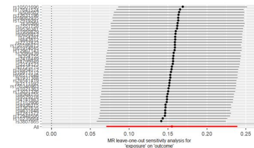
MDD(PGC) on CVD
