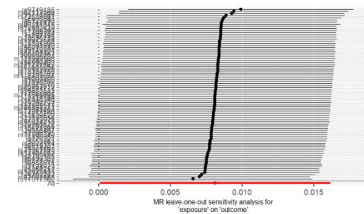
Anxiety(PGC) on HF
