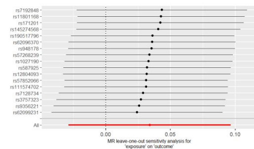
MDD(PGC) on CVD
