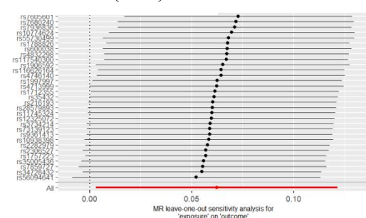
HF on MDD(PGC)
