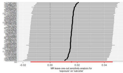
CAD on Anxiety(PGC)
