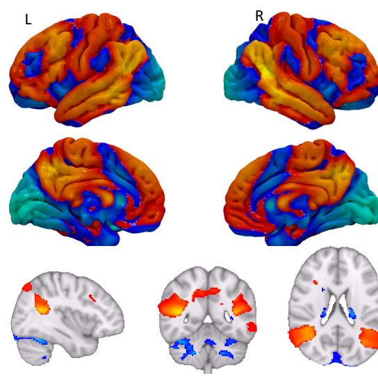
ANM using middle temporal tau
