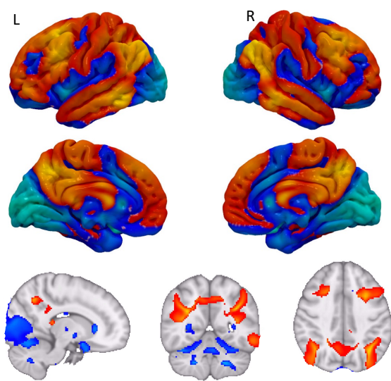
ANM using fusiform tau
