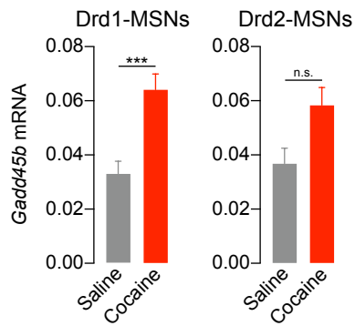
Figure S1. Cocaine-induced changes in Gadd45b mRNA are specific to Drd1-MSNs. snRNA-seq dataset from NAc tissue harvested 1 hr following acute cocaine (20 mg/kg; from Savell, Tuscher, Zipperly, Duke, Phillips et al., Science Advances 2020). In Drd1-MSNs (saline, n=1151; cocaine, n=1597), Gadd45b mRNA is increased by cocaine. In Drd2-MSNs (saline, n=815; cocaine, n=1168), Gadd45b does not differ in saline and cocaine treated rats. *** p < 0.001 for indicated comparison.
