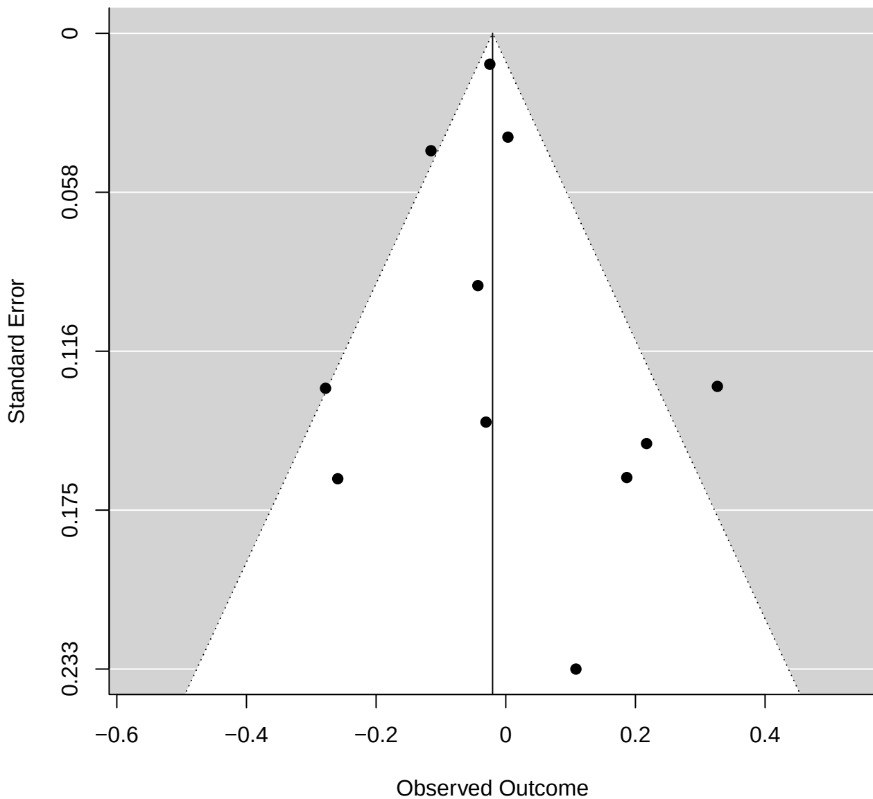
Funnel plot of rs1801131 ( p = 0.733 )
