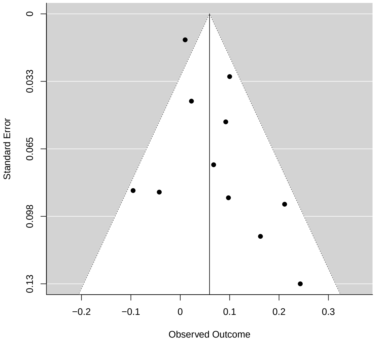
Funnel plot of rs10489202 ( p = 0.0972 )
