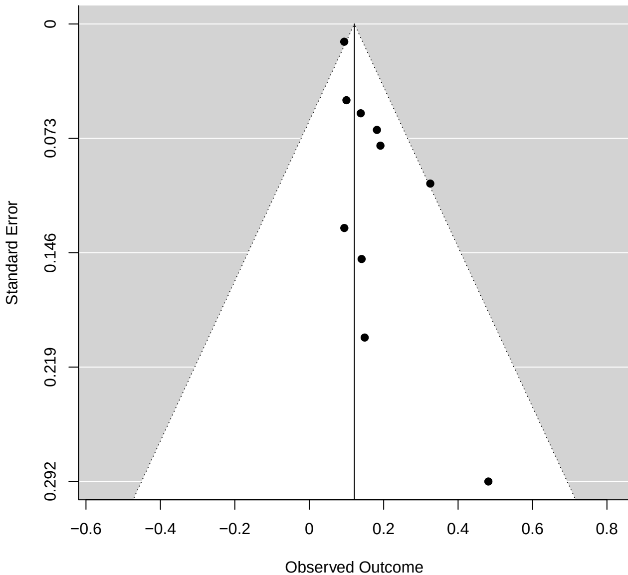
Funnel plot of rs1006737 ( p = 0.0125 )
