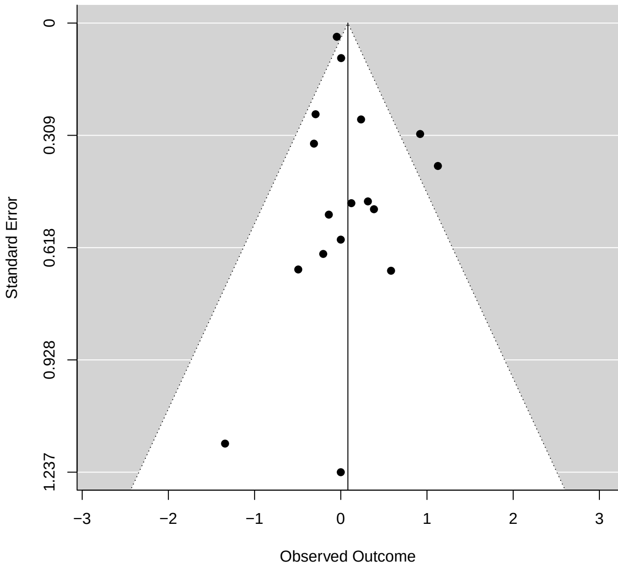
Funnel plot of rs1801028 ( p = 0.27 )
