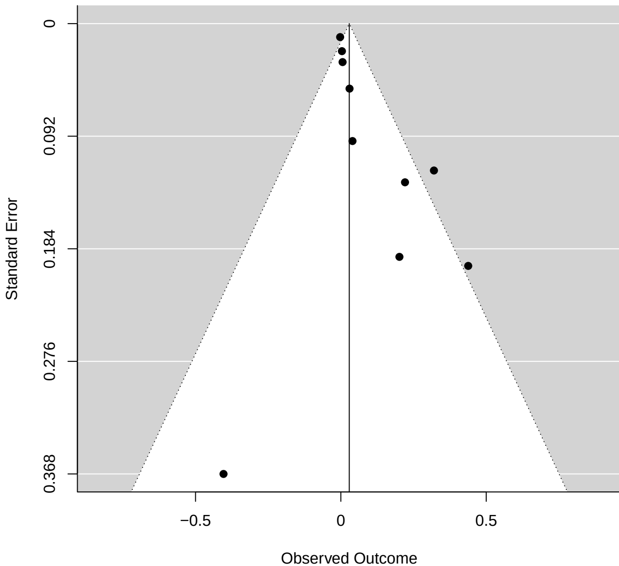
Funnel plot of rs1816072 ( p = 0.0397 )
