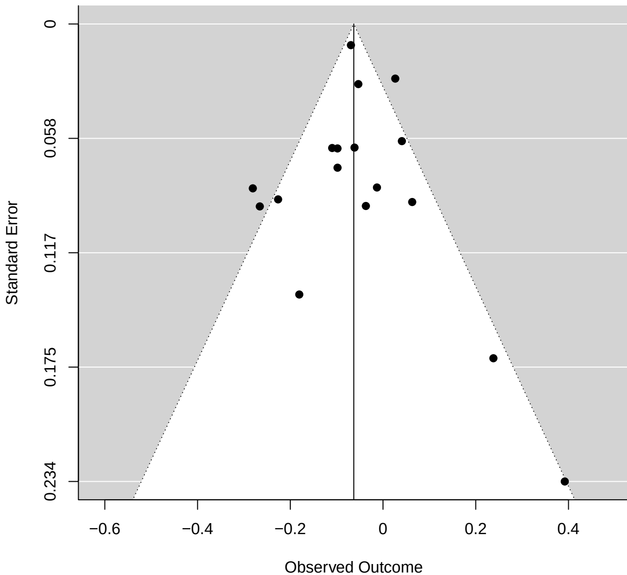
Funnel plot of rs1344706 ( p = 0.915 )
