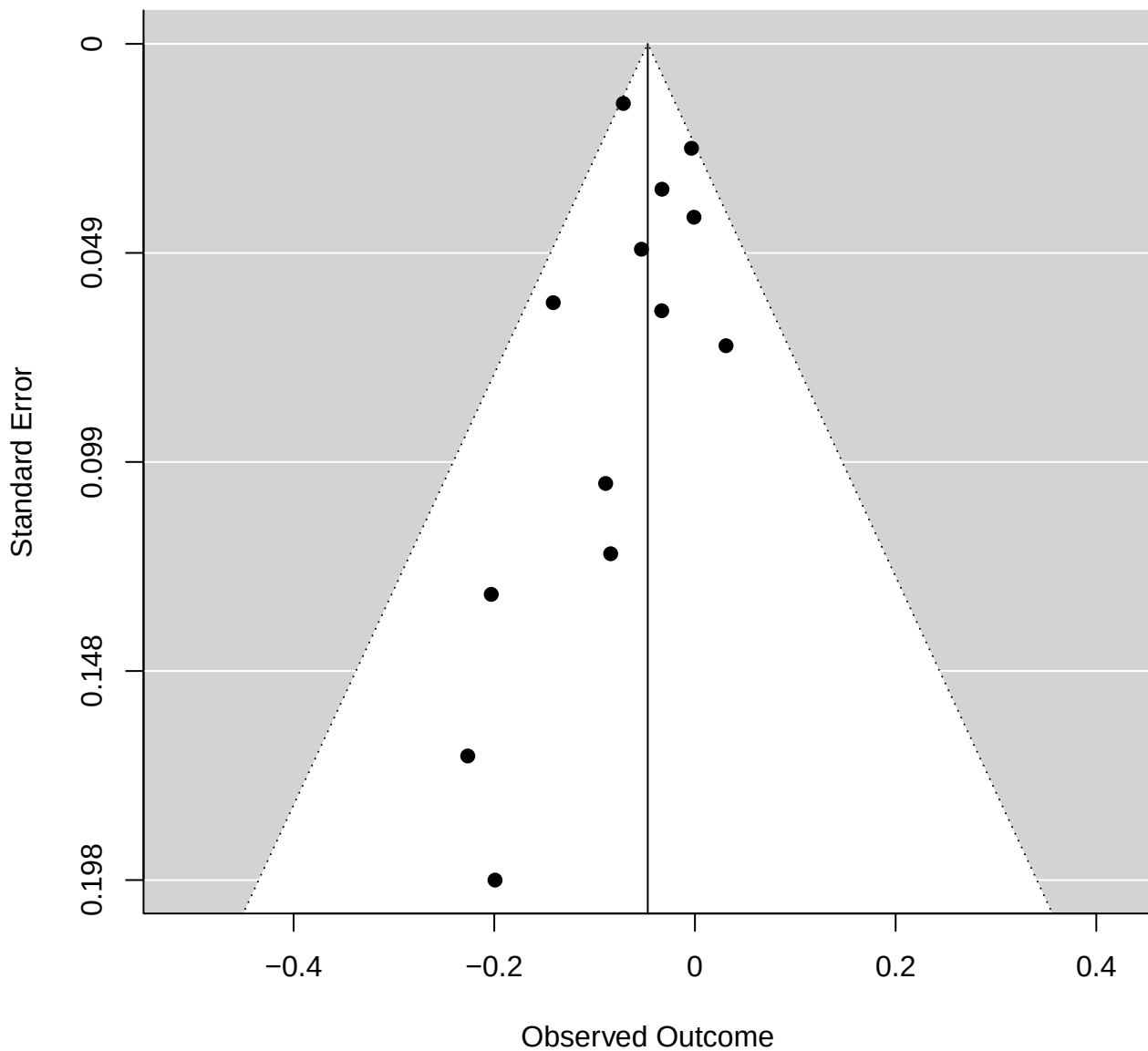
Funnel plot of rs12807809 ( p = 0.654 )
