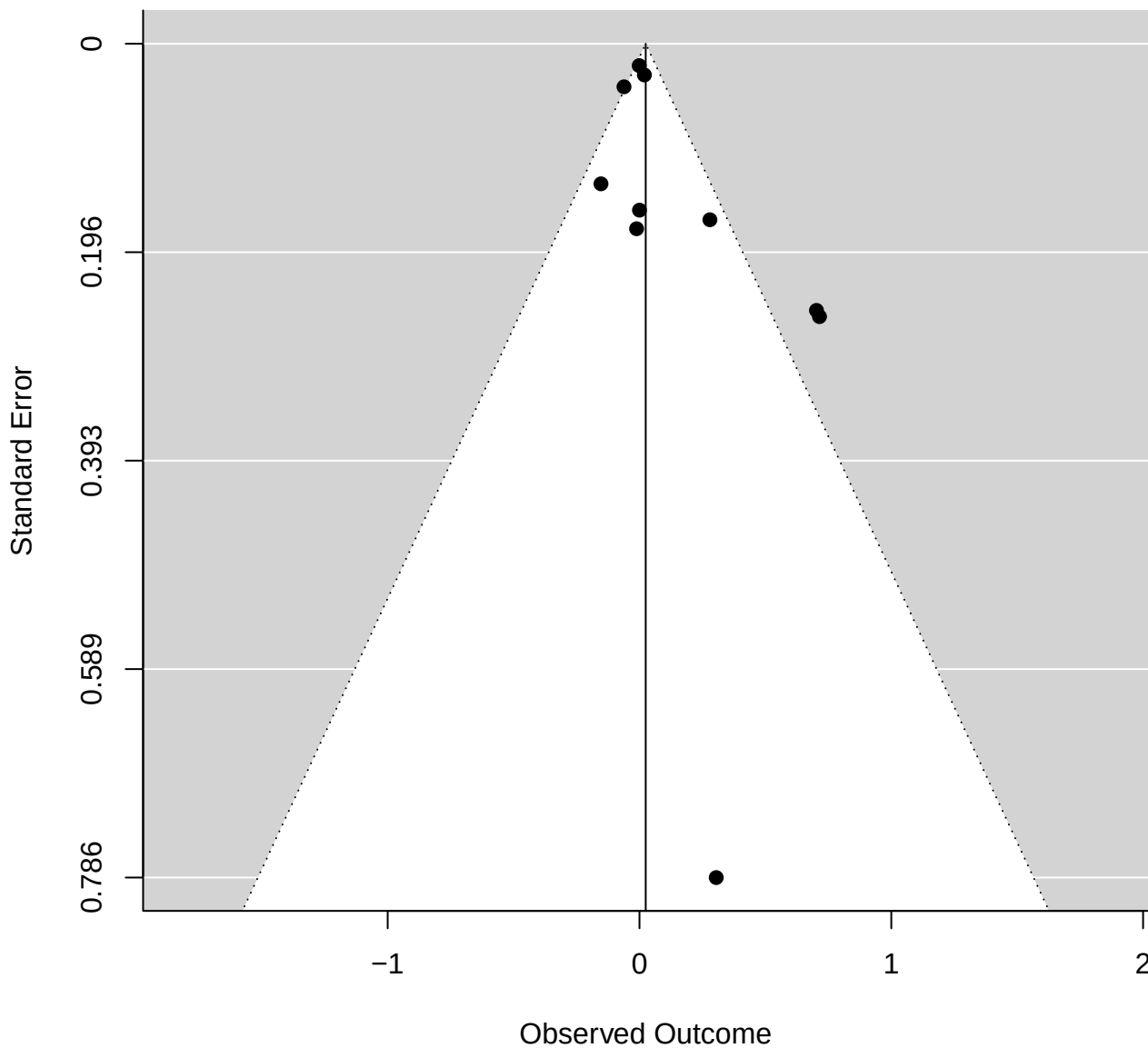
Funnel plot of rs6556547 ( p = 0.156 )
