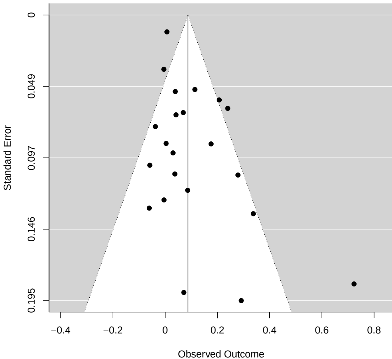
Funnel plot of rs1801133 ( p = 0.00745 )
