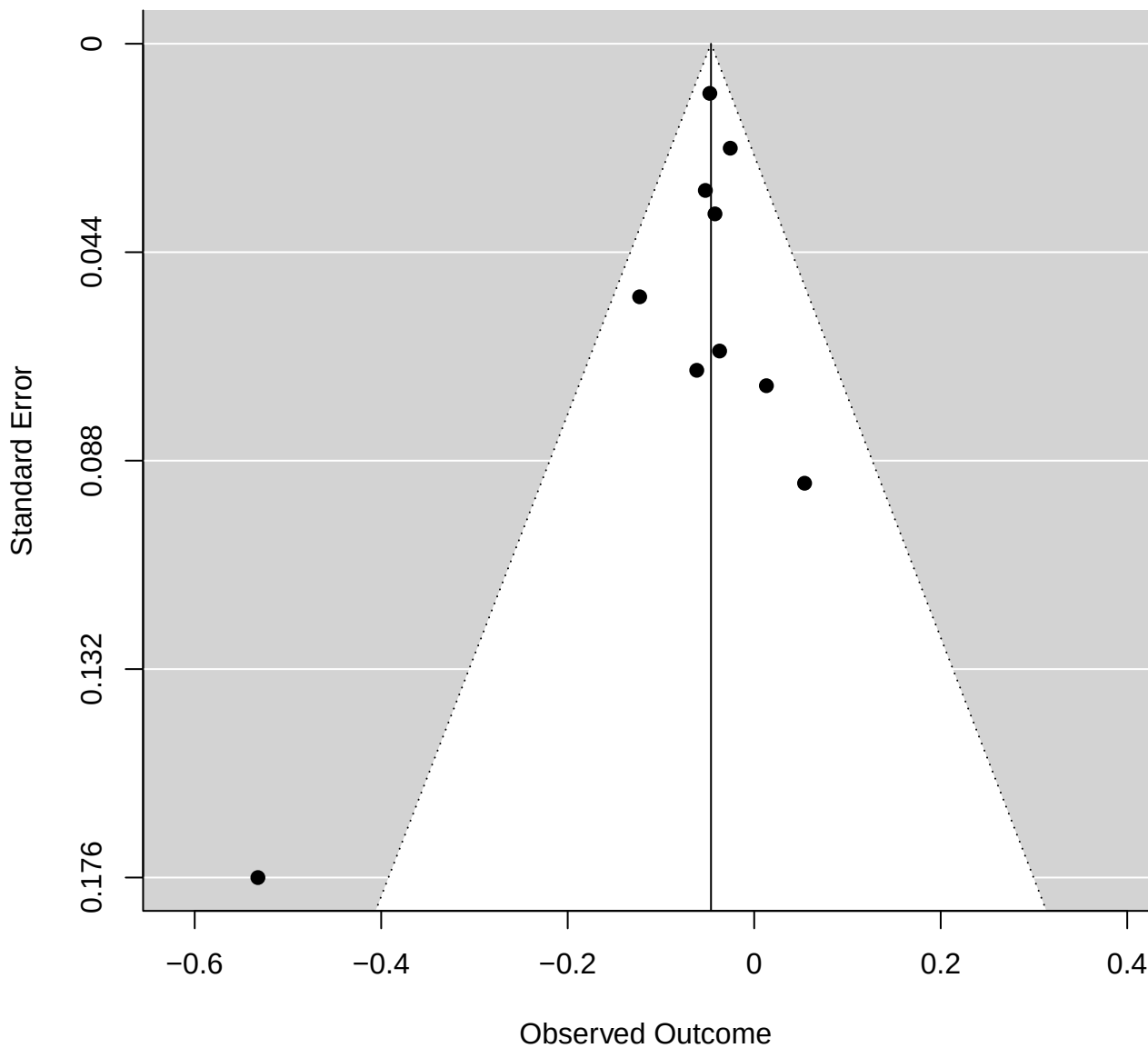
Funnel plot of rs3016384 ( p = 0.508 )
