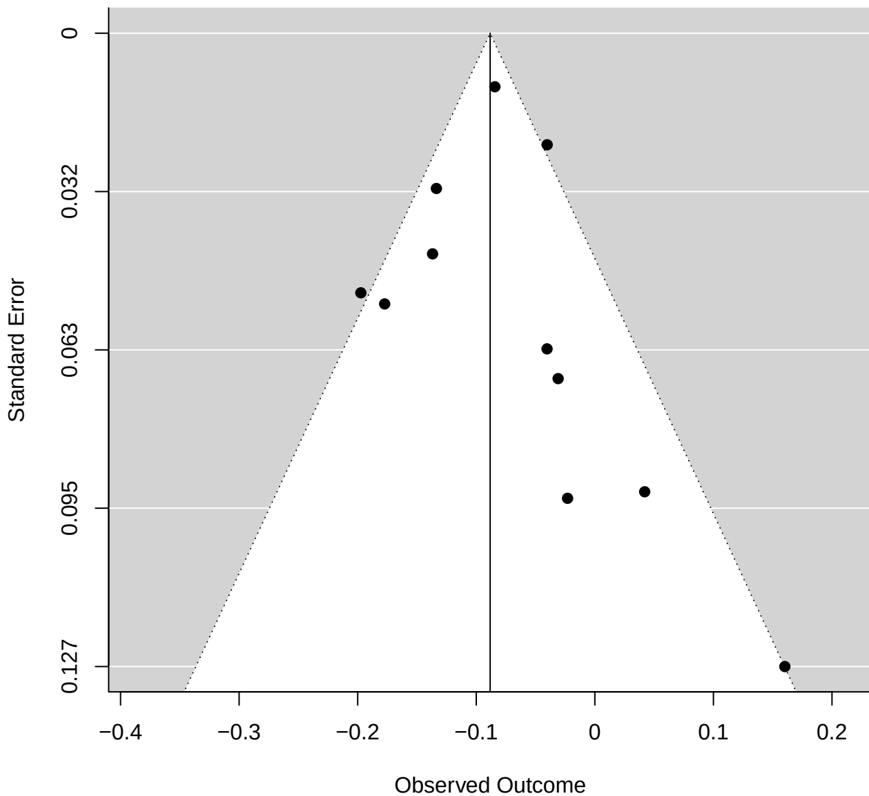
Funnel plot of rs7914558 ( p = 0.82 )
