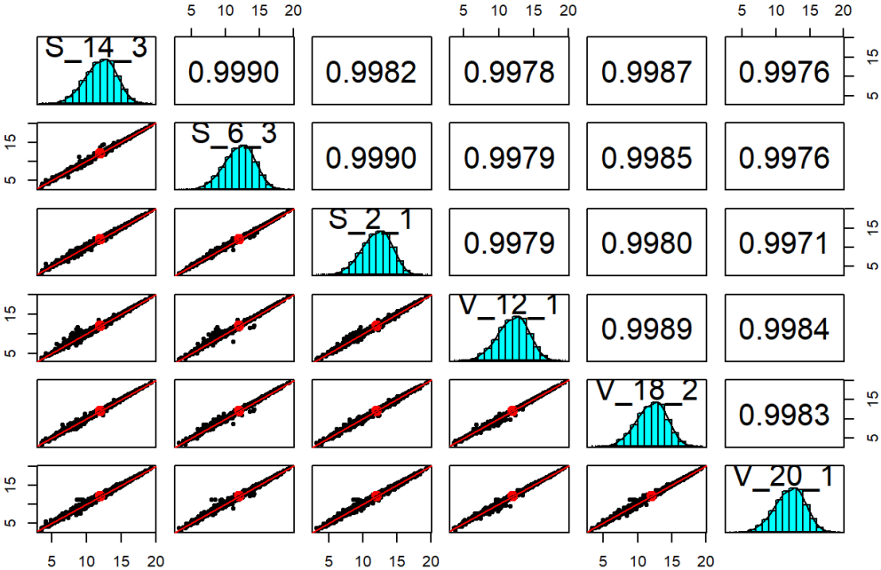
Correlation between TMT samples (Normalized)
