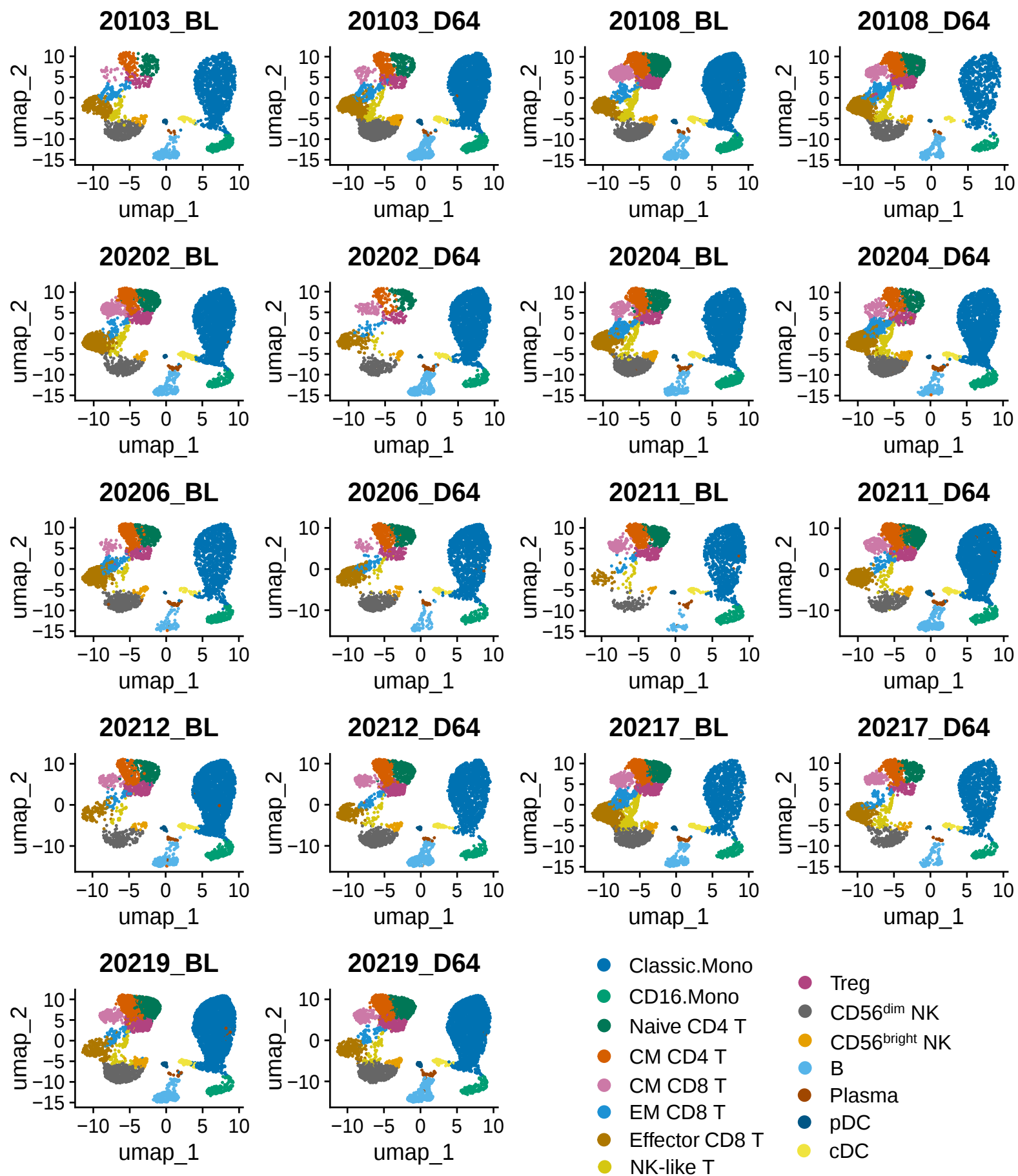
Supplemental Figure S1. Individual UMAP plots of baseline and day 64 PBMCs collected from patients before (BL) and after (D64) they were administered with TILT-123. CM CD4 T = Central Memory CD4 T cells, CM CD8 T = Central Memory CD8 T cells, EM CD8 T = Effector Memory CD8 T cells, Treg = T regulatory cells, cDC = conventional dendritic cells, pDC = plasmacytoid dendritic cells.
