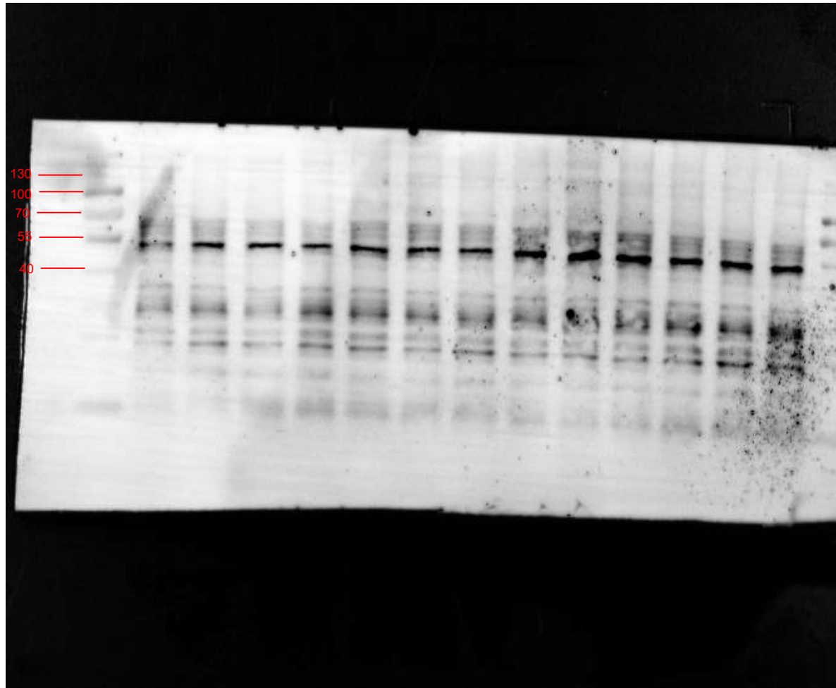
Figure 1G TRIM27
