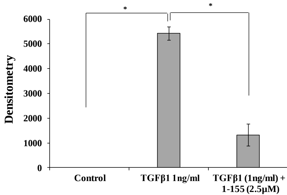
Supplementary Figure S4. Densitometry of the Western blots for TG2 present in the syndecan-4 immuno-complex as shown in Figure 4c . Data are the means \pm S.D. from 3 separate experiments. *, p < 0.05 .
