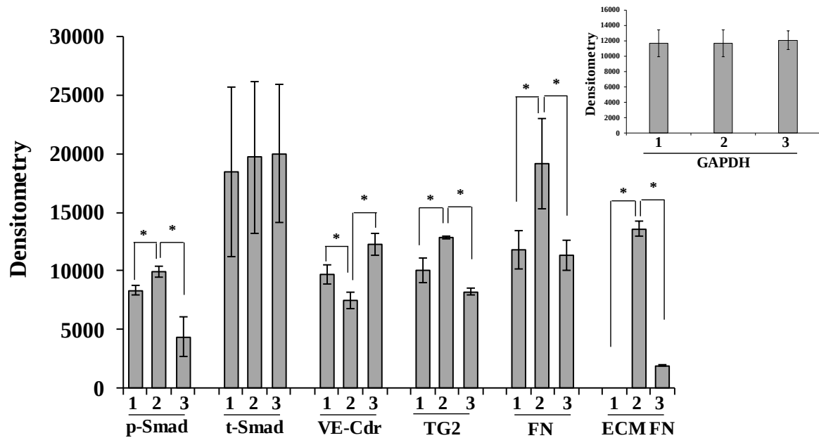
Supplementary Figure S6. Densitometry of the Western blots of phosphorylated Smad2/3 (p-Smad2/3), total Smad (t-Smad2/3), VE-cadherin (VE-Cdr) and FN in HUVEC and ECM FN deposition by these cells as shown in Figure 5a . GAPDH was used as the equal loading control. Lane 1: Control; Lane 2: TGFβ1 treatment at 1ng/ml; and Lane 3: TGFβ1 (1ng/ml) + 1-155 (2.5μM). Data are the means ± S.D. from 3 separate experiments. *, p<0.05.
