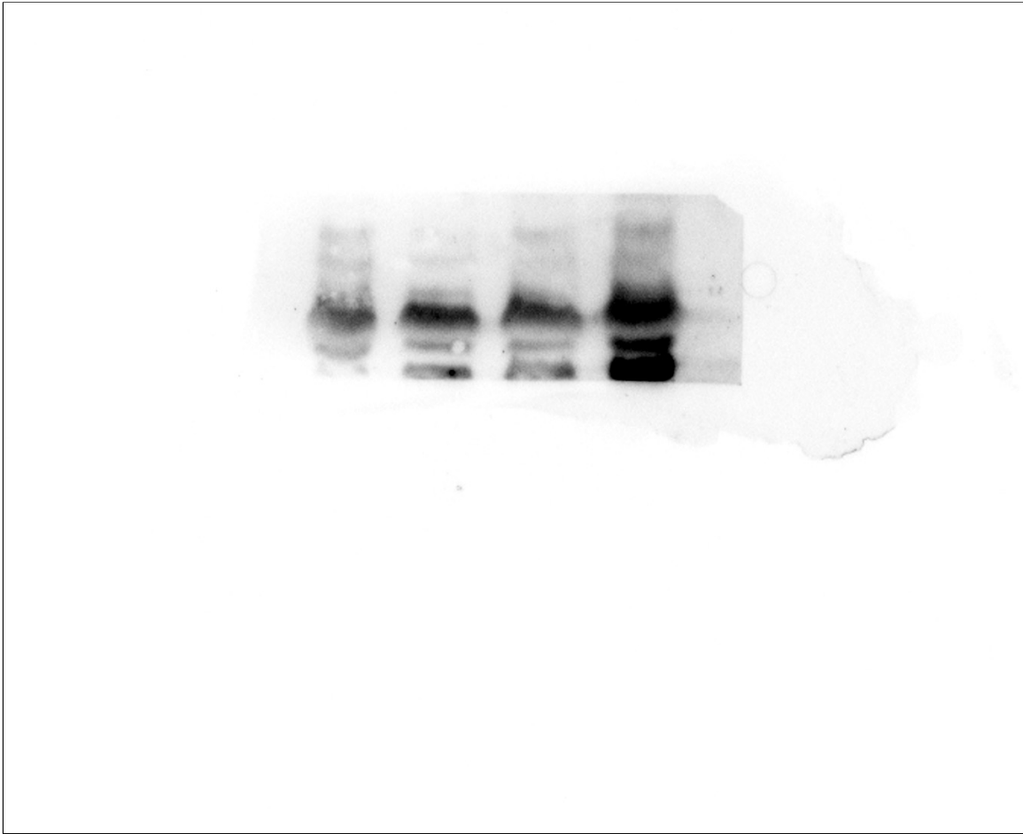
Cleaved Caspase-3
