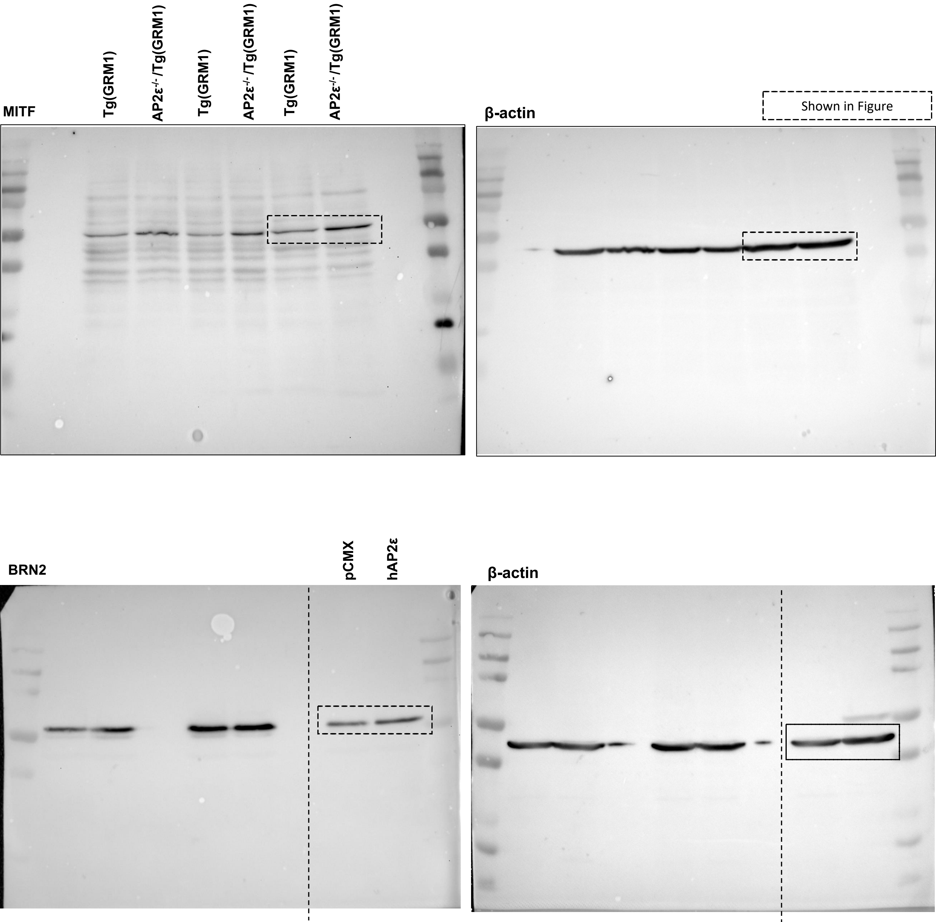
Figure 5 A – Western Blot
