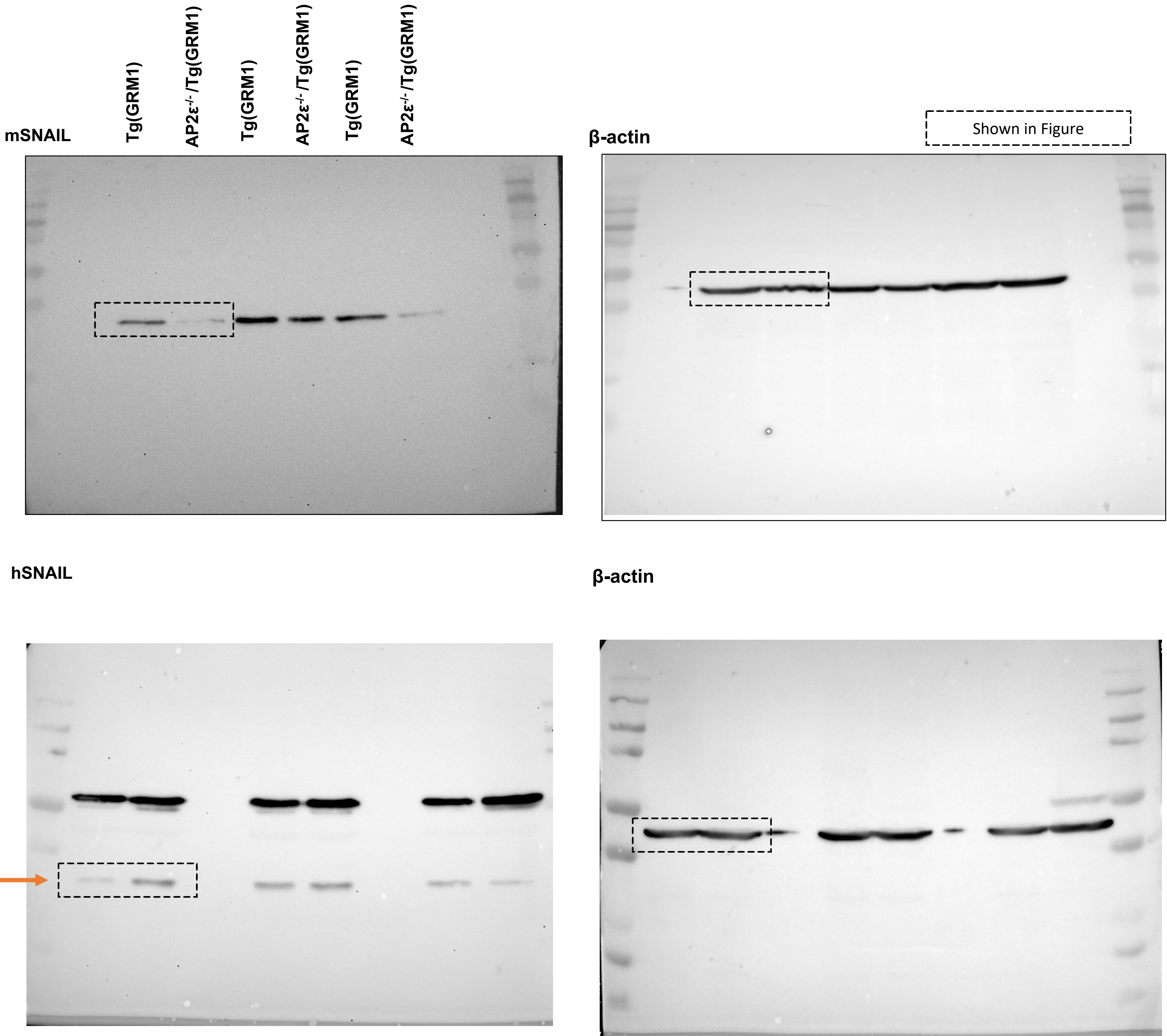
Figure 5C/D – Western Blot
