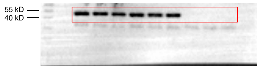
Pro-casp1
