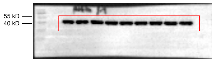
\beta -actin
