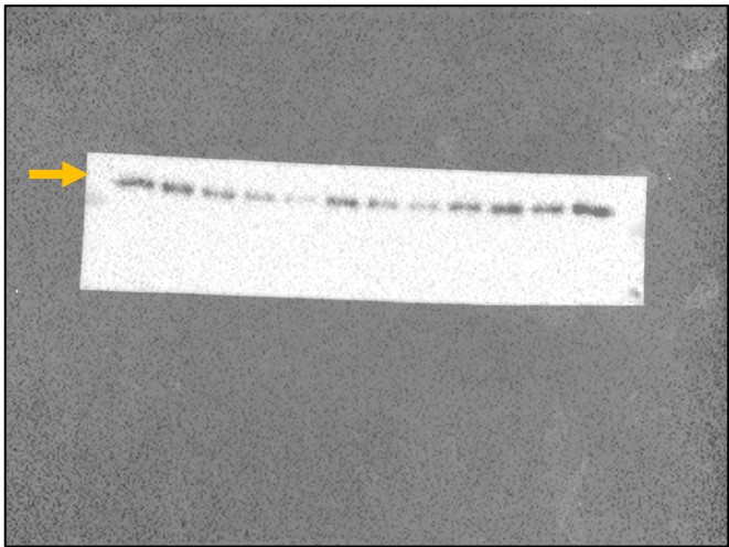
Gapdh (36 KDa)
