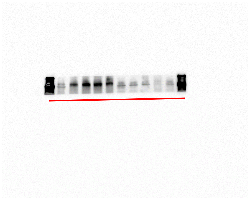
Fig 7D FOXM1
