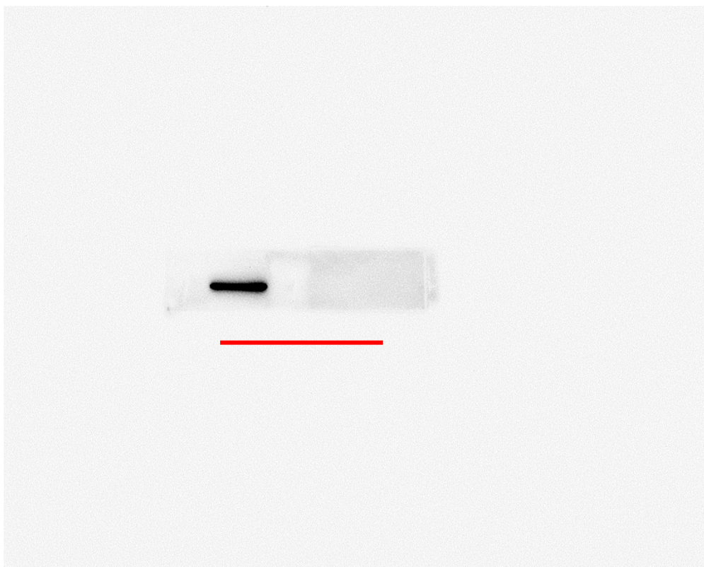
Fig 4B HSPA8
