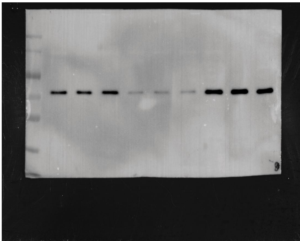
Figure 3A P62
