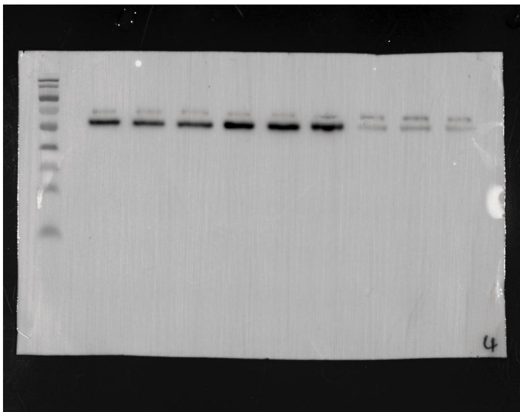
Figure 3A LC3II&LC3I
