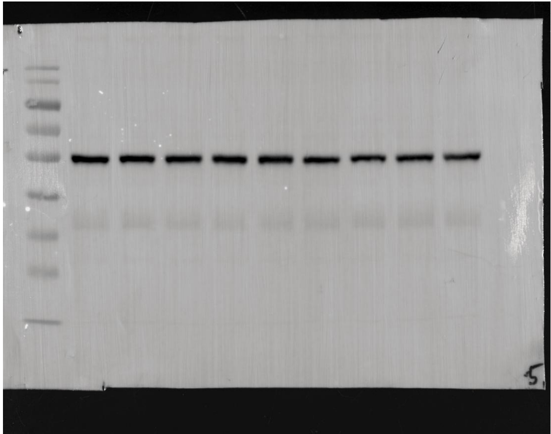
Figure 3A GAPDH
