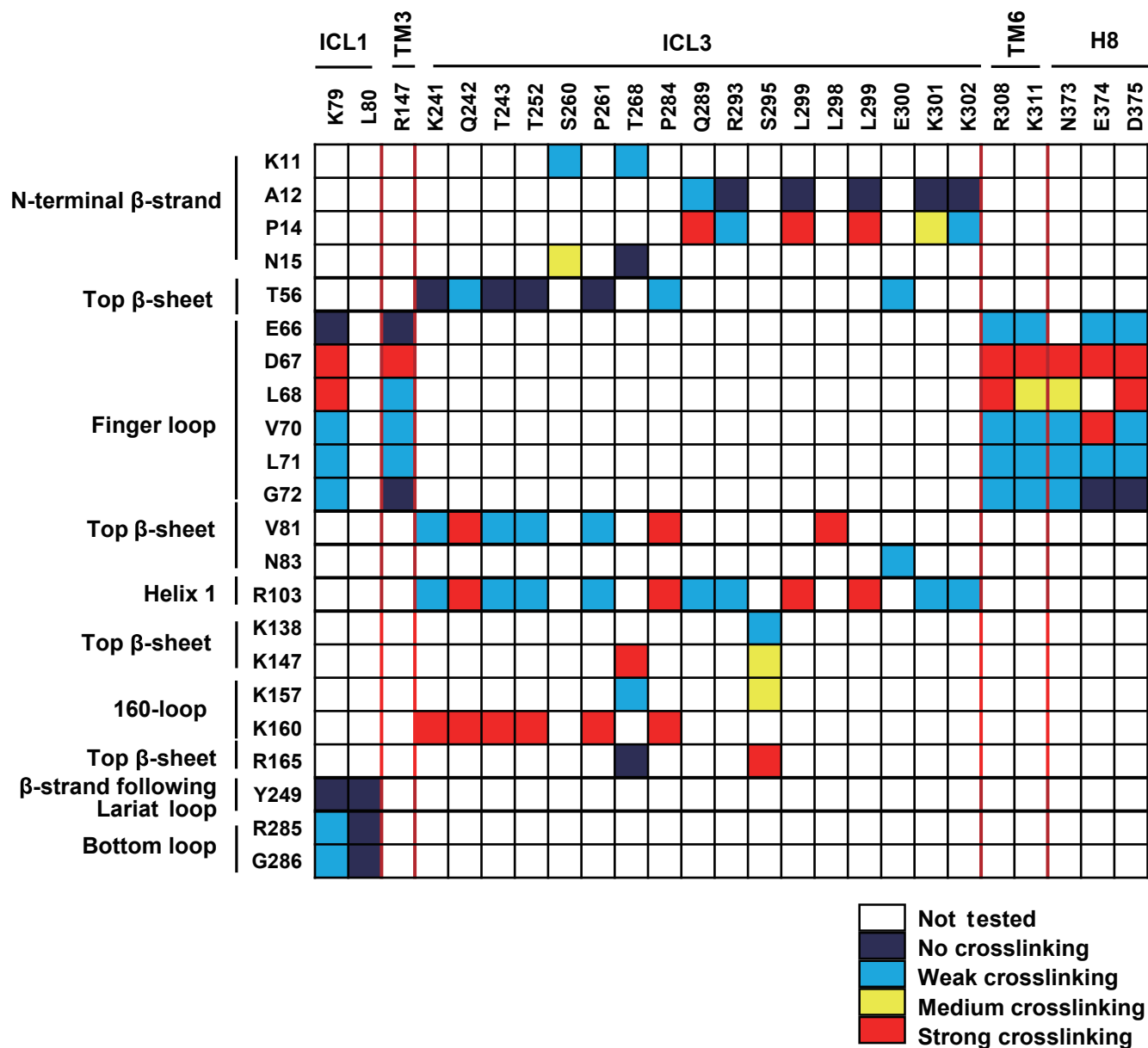
Supplementary information, Fig. S10| Heat map summary of all Arr2–5-HTR1B disulfide crosslinking data. Color code used for the strength of crosslinking signals: strong crosslinking is shown with red; medium crosslinking, yellow; weak crosslinking, cyan; and no obvious crosslinking signal, dark blue.
