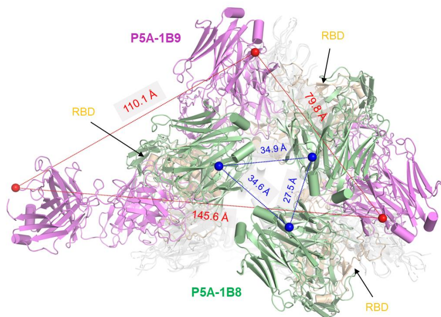
Supplementary information, Fig. S10 | The distance comparison between bound Fabs for P5A-1B8 and P5A-1B9.
